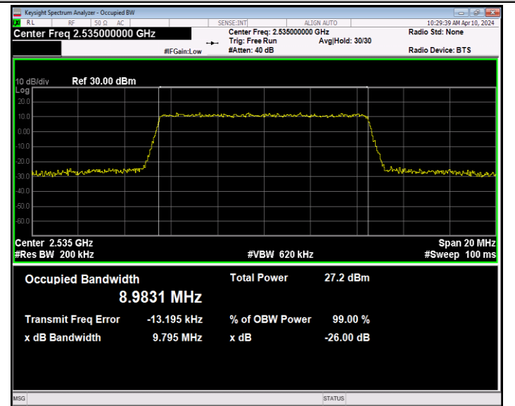
Band7-10MHz-16QAM-21100-50RB#0-PASS
