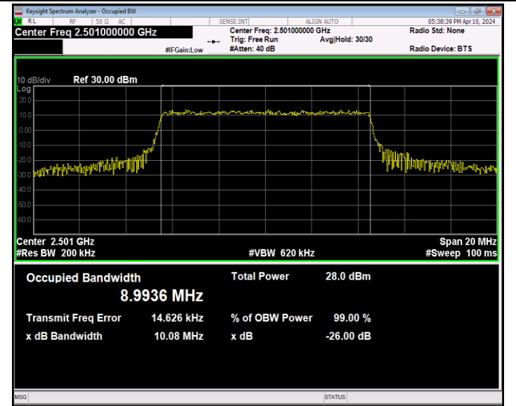
Band41-10MHz-QPSK-39700-50RB#0-PASS
