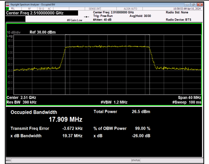
Band7-20MHz-64QAM-20850-100RB#0-PASS
