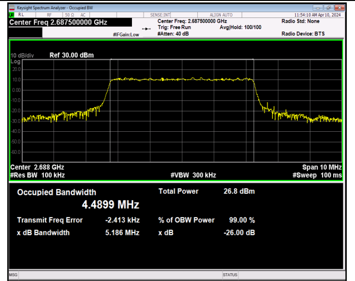
Band41-5MHz-16QAM-41565-25RB#0-PASS
