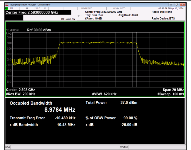
Band41-10MHz-16QAM-40620-50RB#0-PASS
