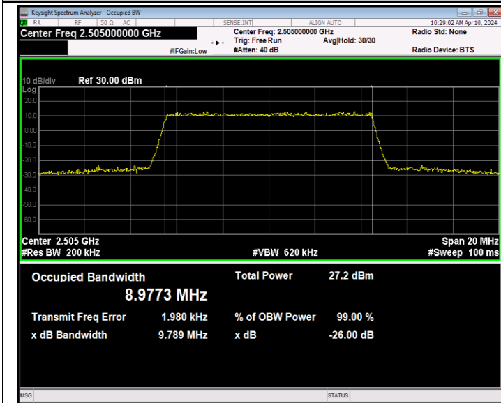
Band7-10MHz-16QAM-20800-50RB#0-PASS
