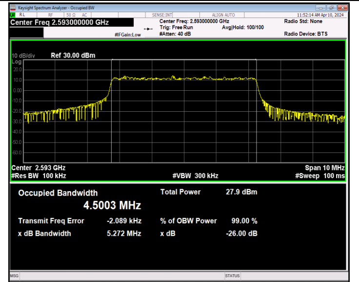
Band41-5MHz-QPSK-40620-25RB#0-PASS
