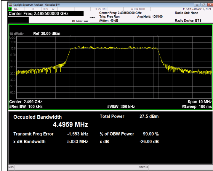
Band41-5MHz-QPSK-39675-25RB#0-PASS
