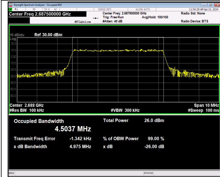
Band41-5MHz-64QAM-41565-25RB#0-PASS
