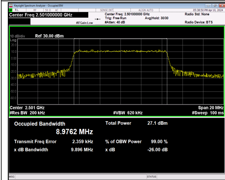
Band41-10MHz-16QAM-39700-50RB#0-PASS
