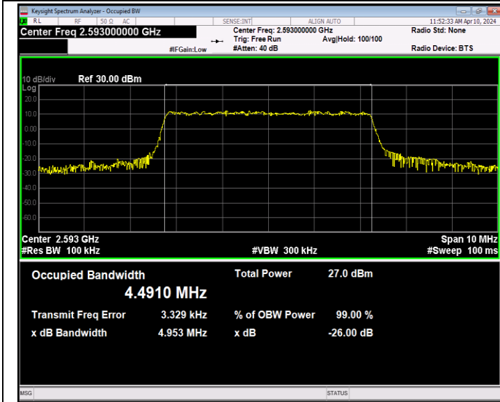
Band41-5MHz-16QAM-40620-25RB#0-PASS
