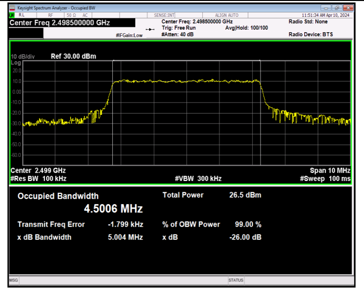
Band41-5MHz-16QAM-39675-25RB#0-PASS
