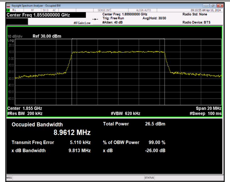
Band2-10MHz-64QAM-18650-50RB#0-PASS
