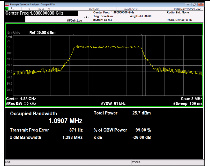
Band2-1.4MHz-64QAM-18900-6RB#0-PASS
