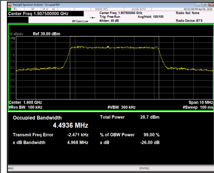
Band2-5MHz-QPSK-19175-25RB#0-PASS
