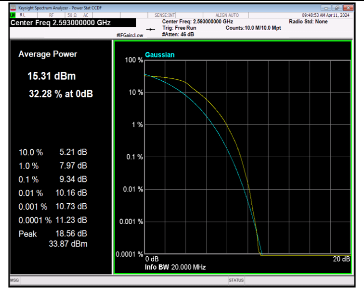
Band41-20MHz-QPSK-40620-100RB#0-PASS
