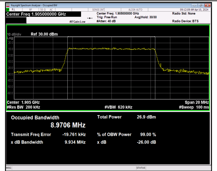
Band2-10MHz-64QAM-19150-50RB#0-PASS
