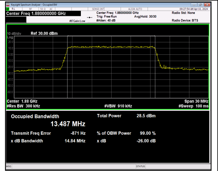
Band2-15MHz-QPSK-18900-75RB#0-PASS
