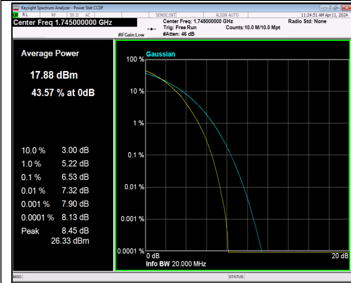
Band66-20MHz-64QAM-132322-100RB#0-PASS
