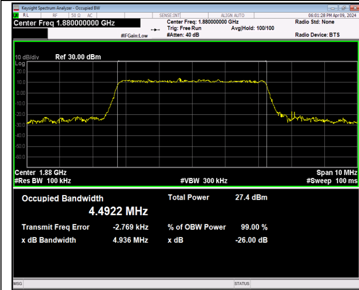
Band2-5MHz-16QAM-18900-25RB#0-PASS
