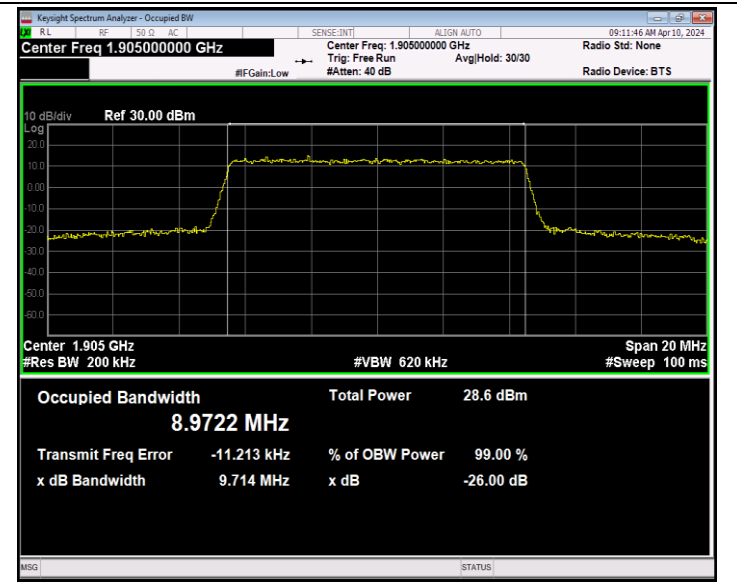
Band2-10MHz-QPSK-19150-50RB#0-PASS
