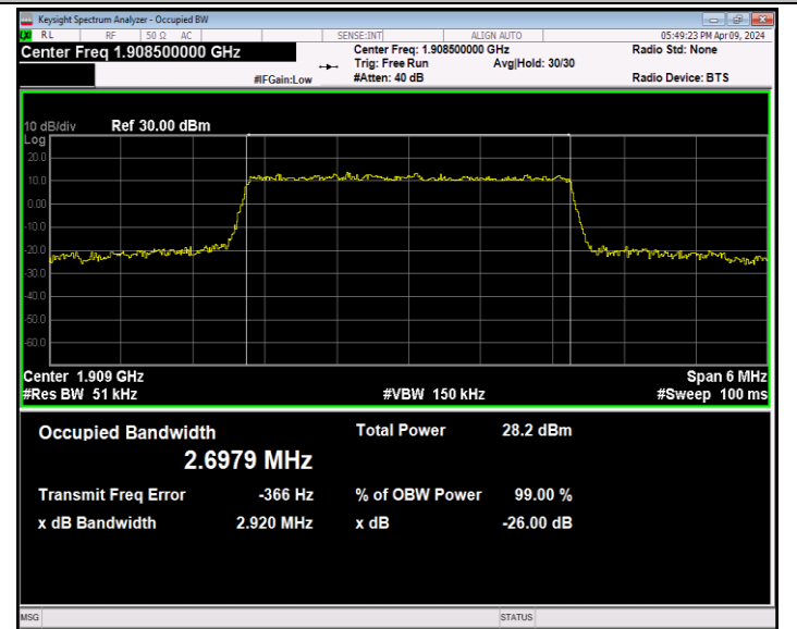
Band2-3MHz-QPSK-19185-15RB#0-PASS
