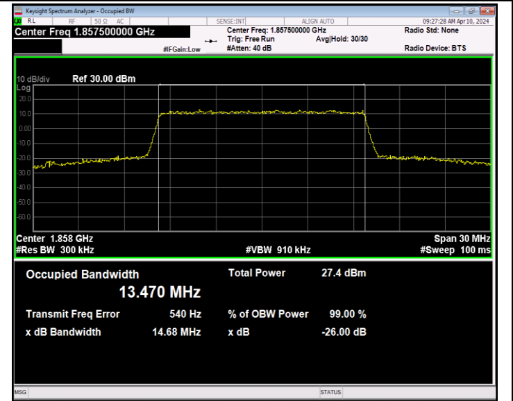
Band2-15MHz-16QAM-18675-75RB#0-PASS
