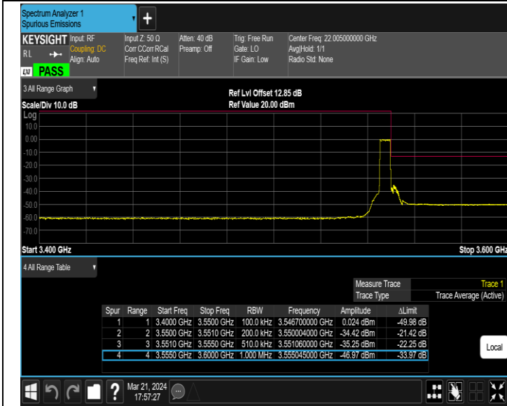
Band42_5MHz_64QAM_43065_25RB#0
