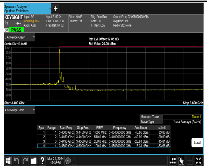
Band42_5MHz_16QAM_42115_1RB#0
