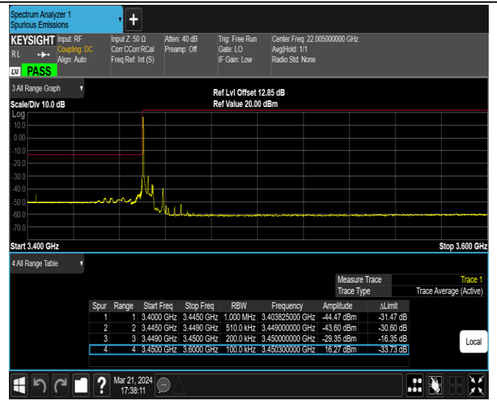
Band42_5MHz_64QAM_42115_1RB#0
