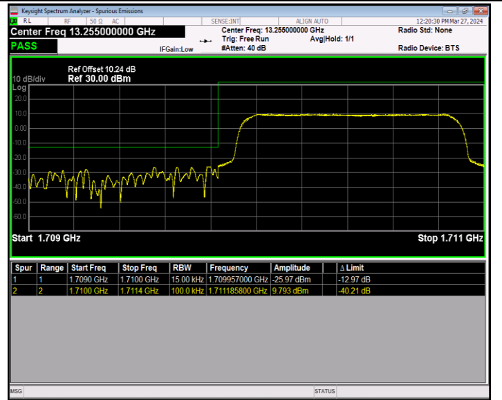
Band66_1.4MHz_QPSK_131979_6RB#0
