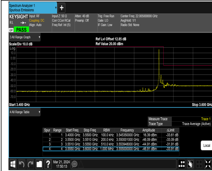
Band42_5MHz_64QAM_43065_1RB#0
