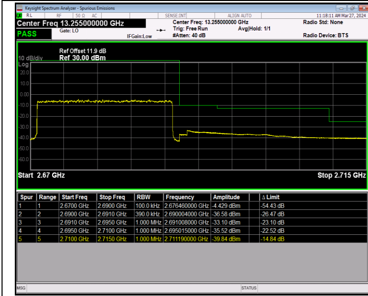
Band41_20MHz_64QAM_41490_100RB#0
