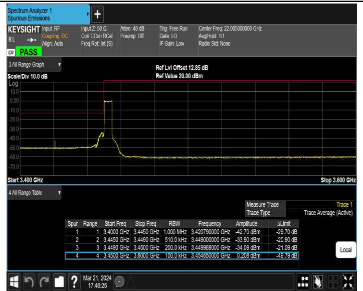
Band42_5MHz_64QAM_42115_25RB#0
