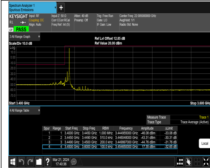
Band42_5MHz_16QAM_42115_1RB#24
