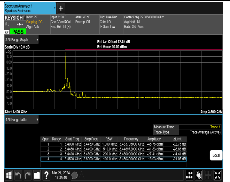
Band42_5MHz_QPSK_42115_1RB#0
