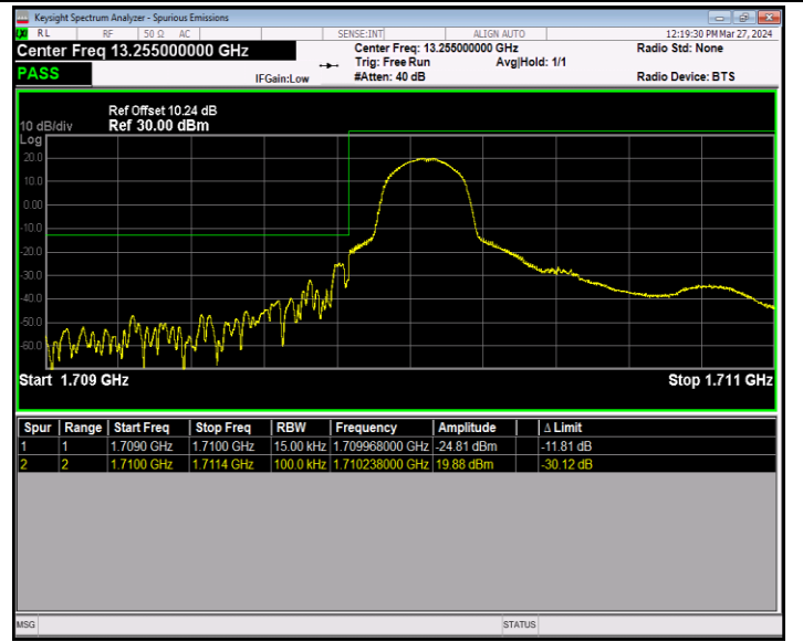
Band66_1.4MHz_QPSK_131979_1RB#0
