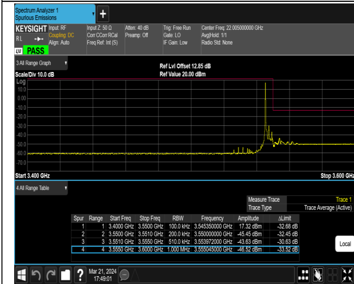
Band42_5MHz_16QAM_43065_1RB#0
