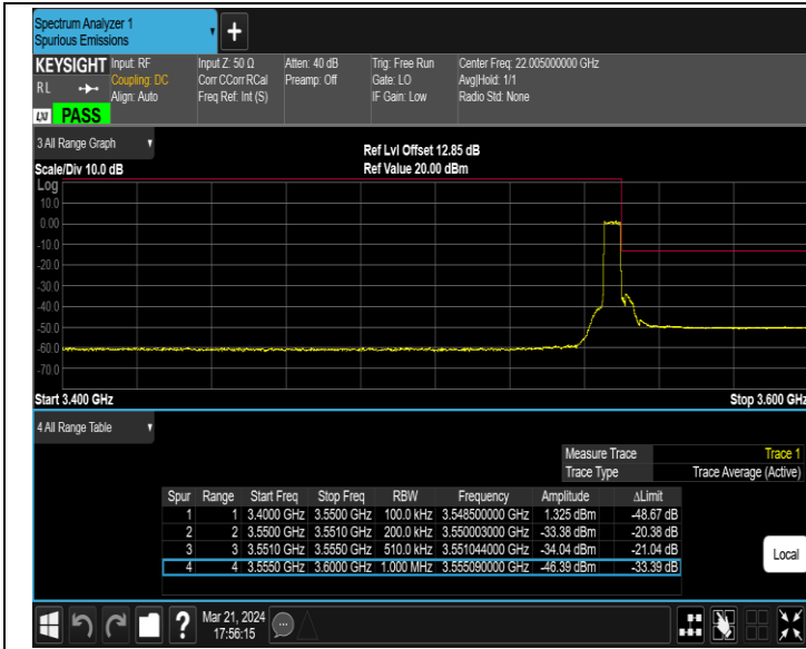
Band42_5MHz_16QAM_43065_25RB#0
