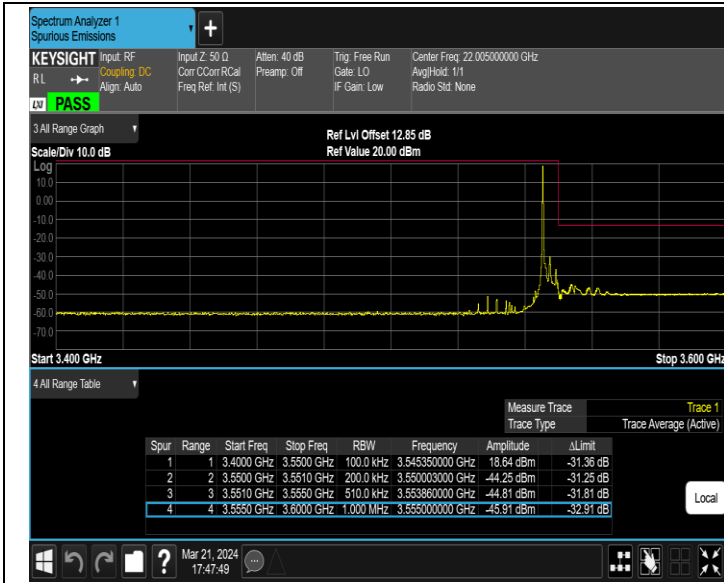
Band42_5MHz_QPSK_43065_1RB#0
