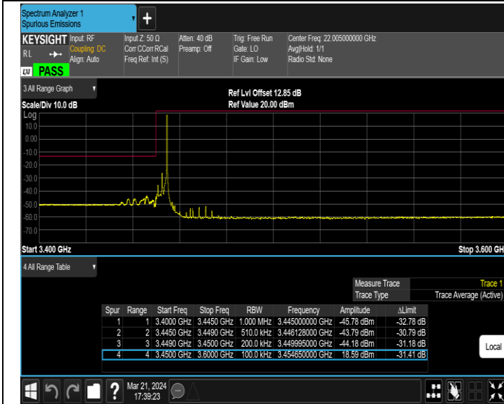
Band42_5MHz_QPSK_42115_1RB#24
