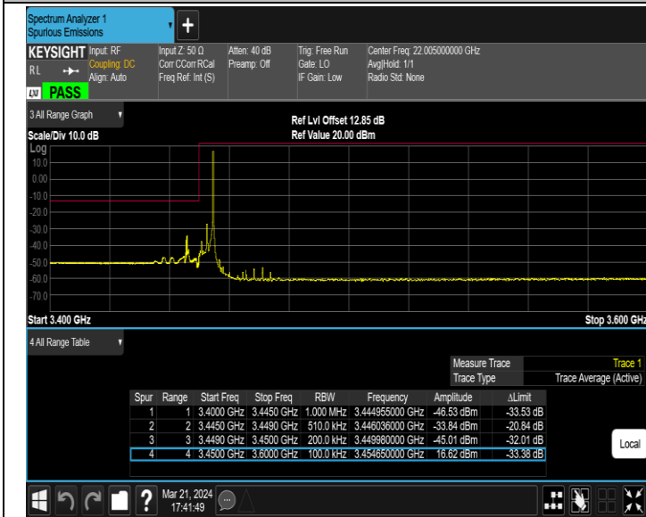
Band42_5MHz_64QAM_42115_1RB#24
