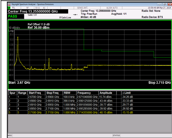
Band41_20MHz_64QAM_41490_1RB#0
