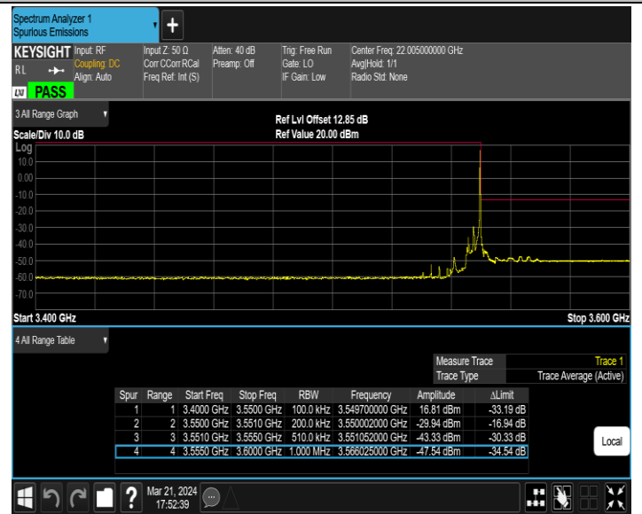
Band42_5MHz_16QAM_43065_1RB#24
