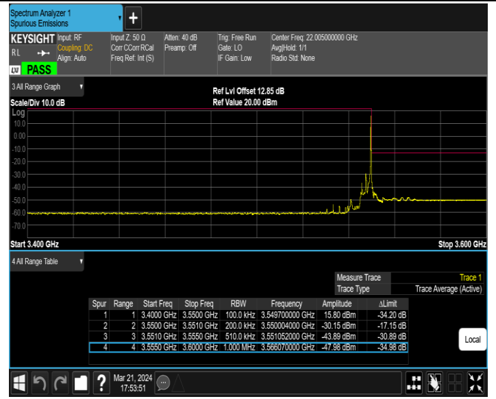
Band42_5MHz_64QAM_43065_1RB#24
