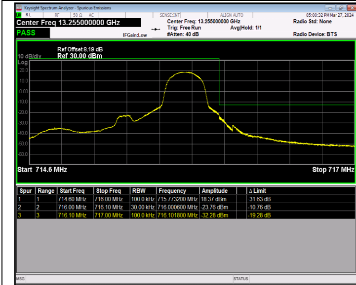
Band12_1.4MHz_16QAM_23173_1RB#5
