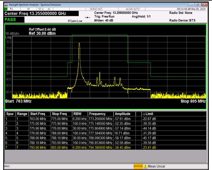
Band13_10MHz_16QAM_23230_1RB#0
