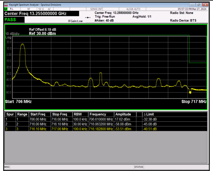
Band12_10MHz_64QAM_23130_1RB#0
