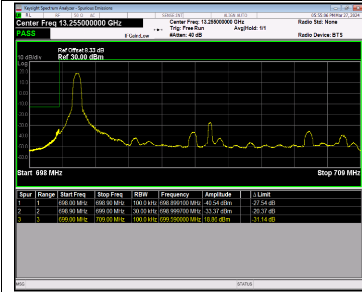
Band12_10MHz_16QAM_23060_1RB#0
