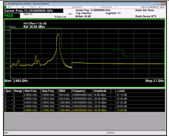
Band41_5MHz_QPSK_41565_1RB#24
