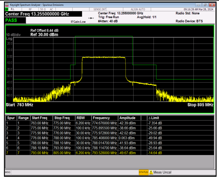
Band13_10MHz_16QAM_23230_50RB#0
