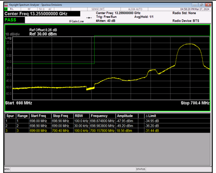
Band12_1.4MHz_16QAM_23017_1RB#0
