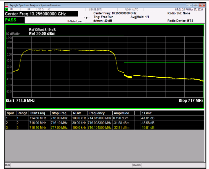
Band12_1.4MHz_64QAM_23173_6RB#0
