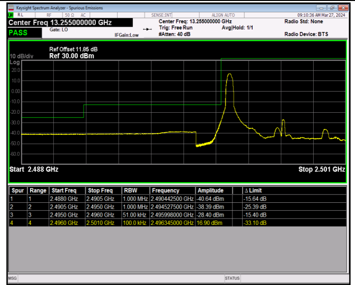
Band41_5MHz_64QAM_39675_1RB#0
