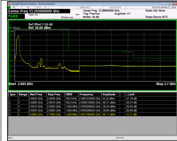
Band41_5MHz_16QAM_41565_1RB#0
