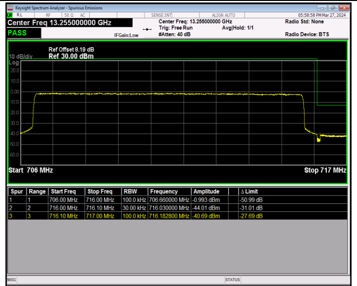
Band12_10MHz_64QAM_23130_50RB#0
