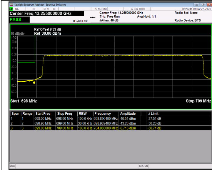
Band12_10MHz_64QAM_23060_50RB#0
