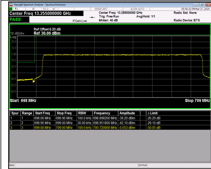
Band12_10MHz_16QAM_23060_50RB#0
