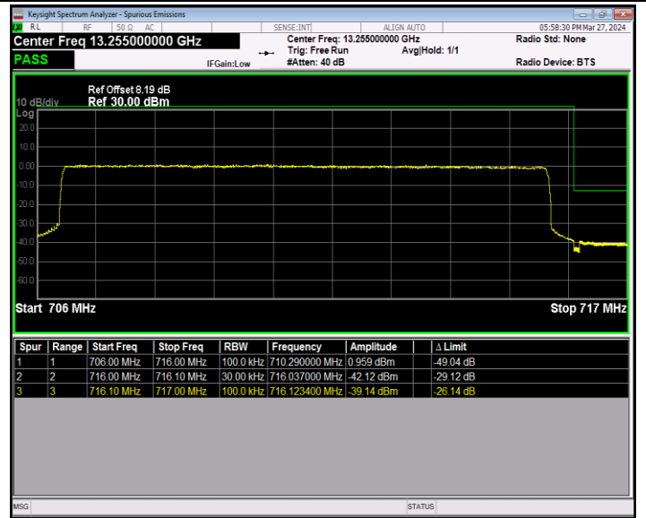
Band12_10MHz_QPSK_23130_50RB#0
