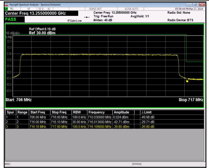
Band12_10MHz_16QAM_23130_50RB#0
