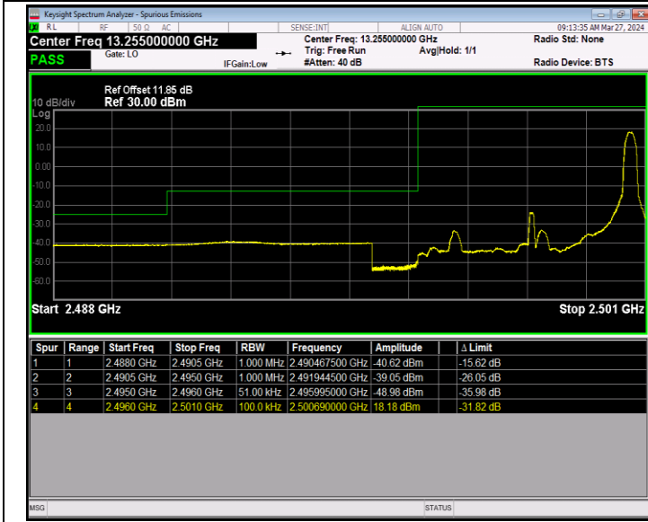
Band41_5MHz_16QAM_39675_1RB#24
