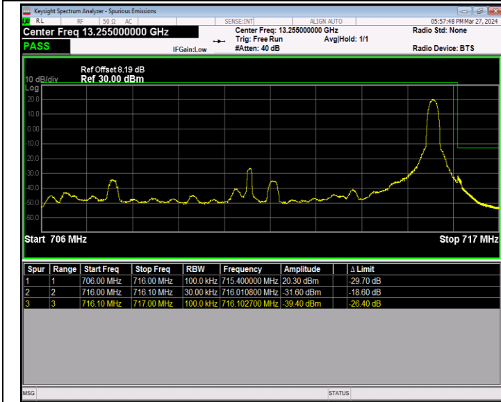
Band12_10MHz_QPSK_23130_1RB#49
