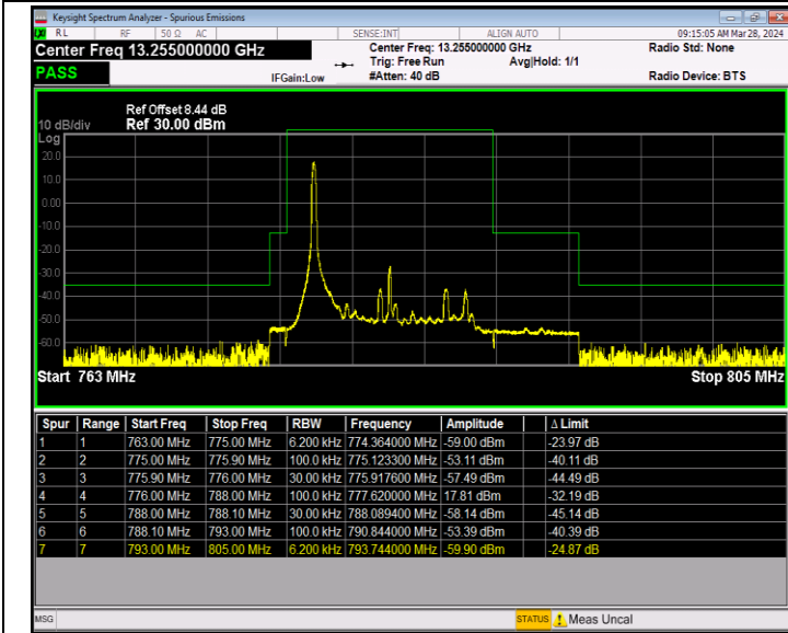
Band13_10MHz_64QAM_23230_1RB#0
