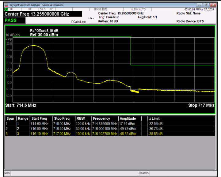
Band12_1.4MHz_64QAM_23173_1RB#0
