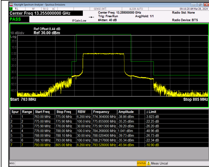
Band13_10MHz_QPSK_23230_50RB#0
