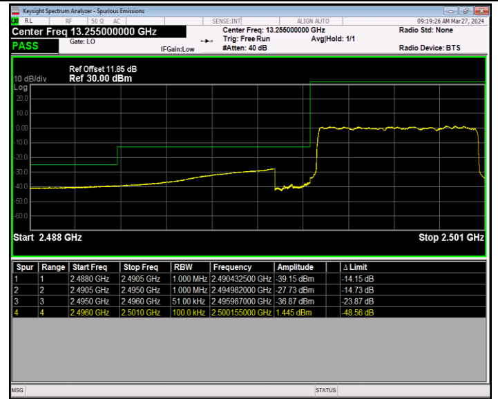
Band41_5MHz_64QAM_39675_25RB#0
