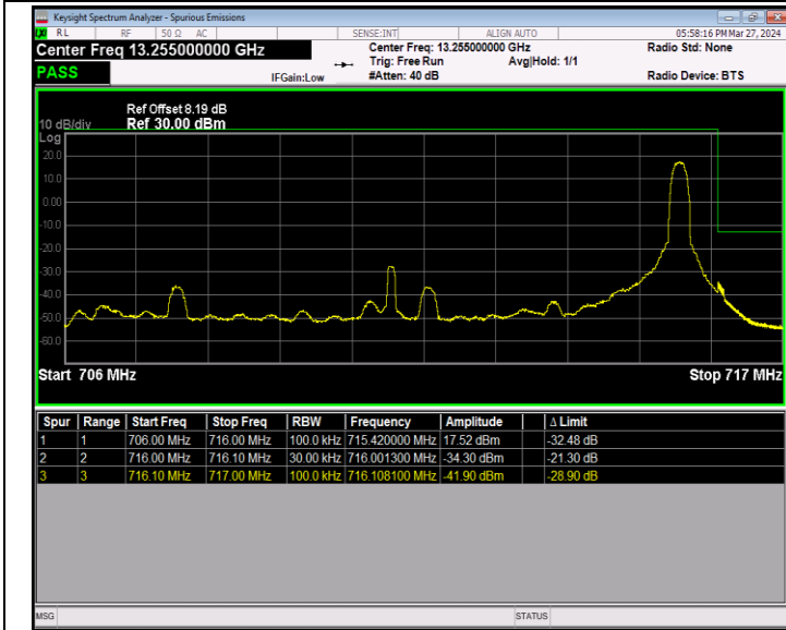
Band12_10MHz_64QAM_23130_1RB#49
