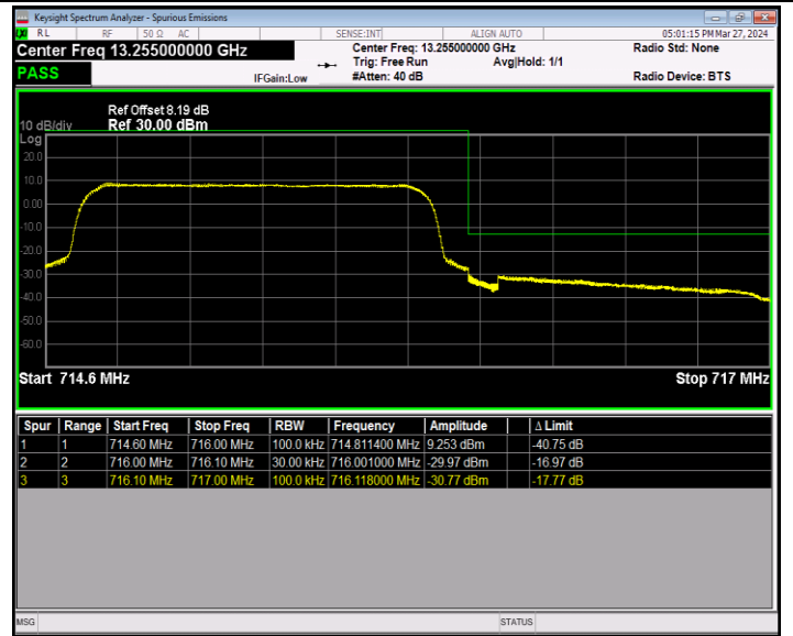
Band12_1.4MHz_16QAM_23173_6RB#0
