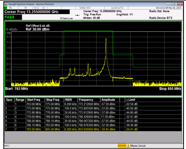
Band13_10MHz_64QAM_23230_1RB#49
