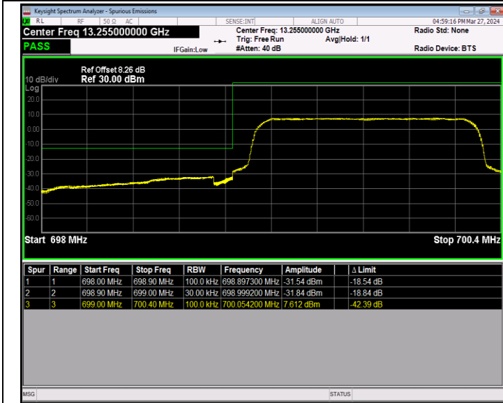
Band12_1.4MHz_64QAM_23017_6RB#0
