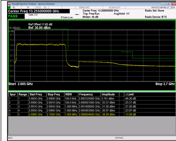
Band41_5MHz_QPSK_41565_25RB#0
