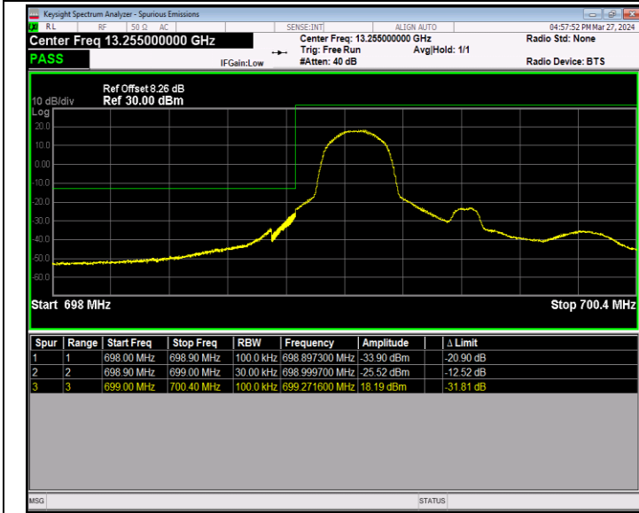
Band12_1.4MHz_64QAM_23017_1RB#0
