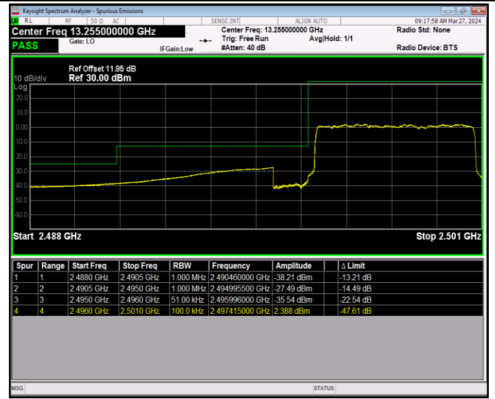
Band41_5MHz_16QAM_39675_25RB#0
