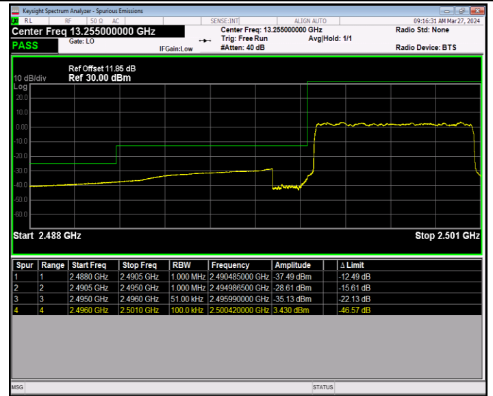
Band41_5MHz_QPSK_39675_25RB#0
