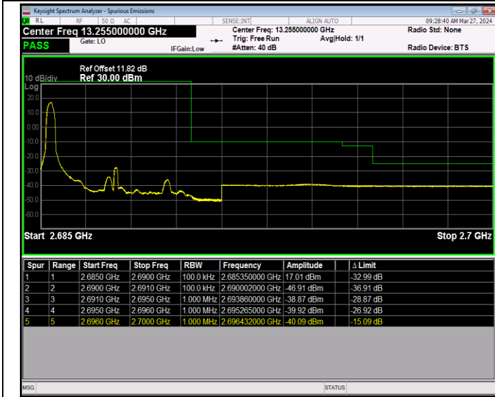
Band41_5MHz_64QAM_41565_1RB#0
