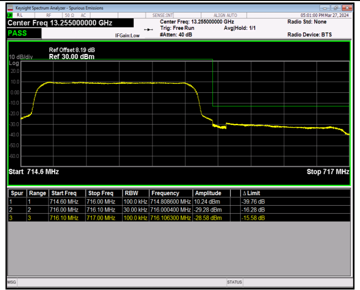
Band12_1.4MHz_QPSK_23173_6RB#0
