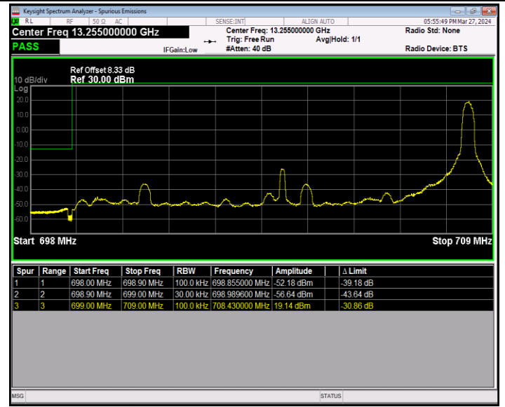
Band12_10MHz_16QAM_23060_1RB#49
