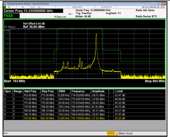
Band13_10MHz_QPSK_23230_1RB#49
