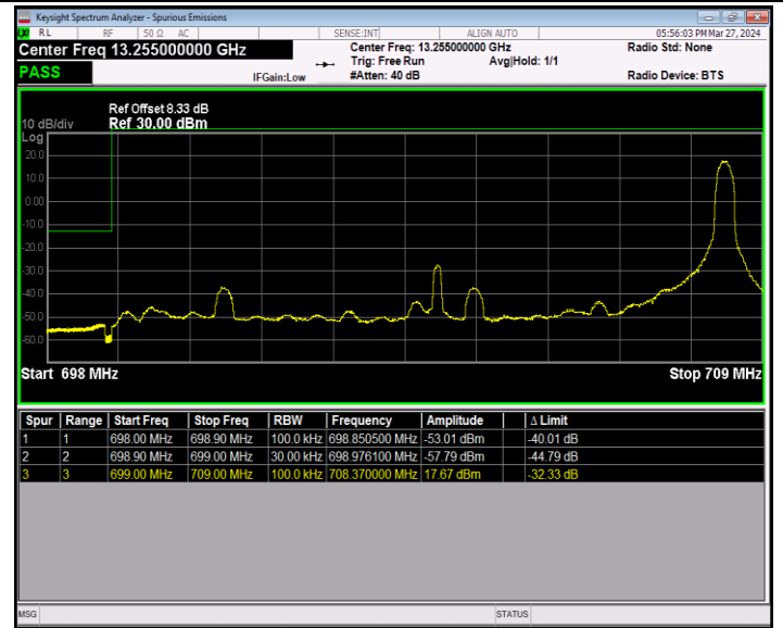
Band12_10MHz_64QAM_23060_1RB#49
