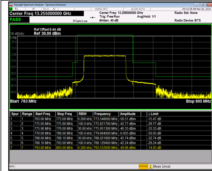
Band13_10MHz_64QAM_23230_50RB#0
