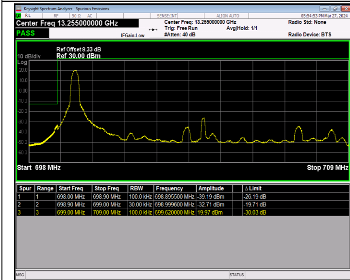
Band12_10MHz_QPSK_23060_1RB#0
