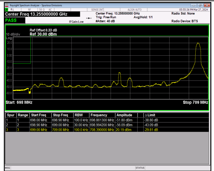
Band12_10MHz_QPSK_23060_1RB#49
