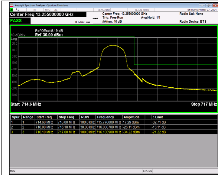
Band12_1.4MHz_64QAM_23173_1RB#5
