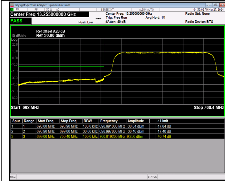
Band12_1.4MHz_16QAM_23017_6RB#0
