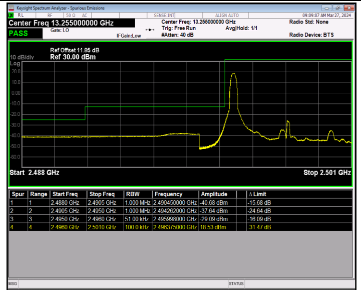
Band41_5MHz_16QAM_39675_1RB#0
