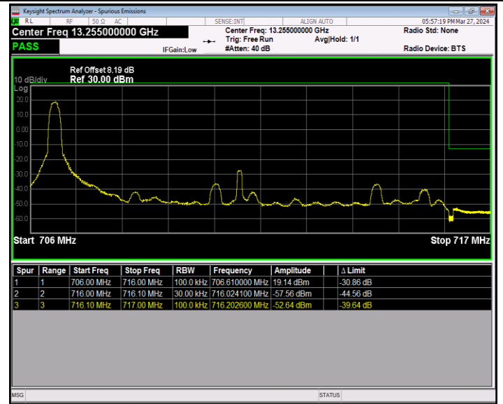
Band12_10MHz_16QAM_23130_1RB#0
