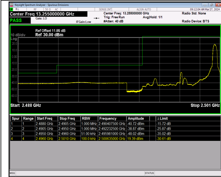
Band41_5MHz_QPSK_39675_1RB#24
