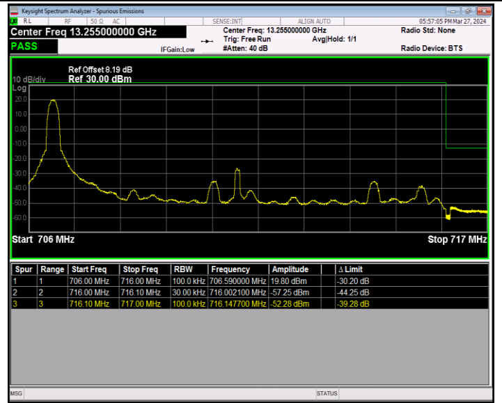
Band12_10MHz_QPSK_23130_1RB#0
