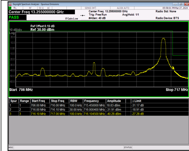
Band12_10MHz_16QAM_23130_1RB#49
