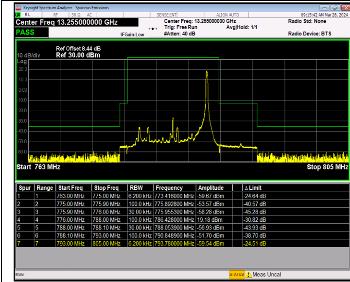
Band13_10MHz_16QAM_23230_1RB#49
