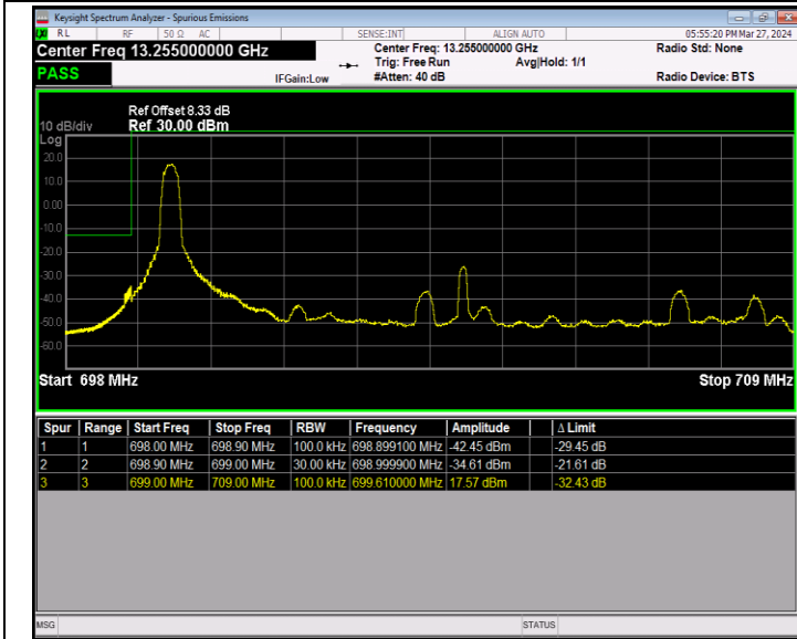
Band12_10MHz_64QAM_23060_1RB#0
