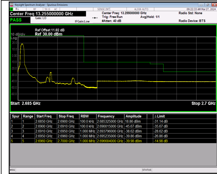
Band41_5MHz_QPSK_41565_1RB#0
