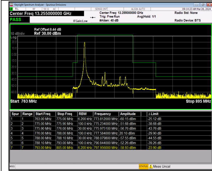
Band13_10MHz_QPSK_23230_1RB#0
