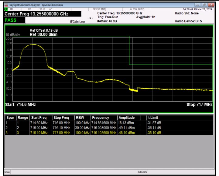
Band12_1.4MHz_16QAM_23173_1RB#0
