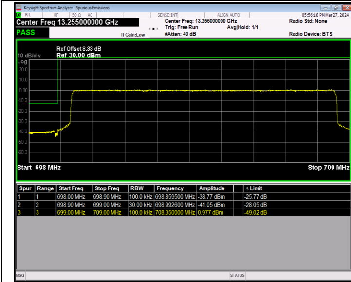
Band12_10MHz_QPSK_23060_50RB#0
