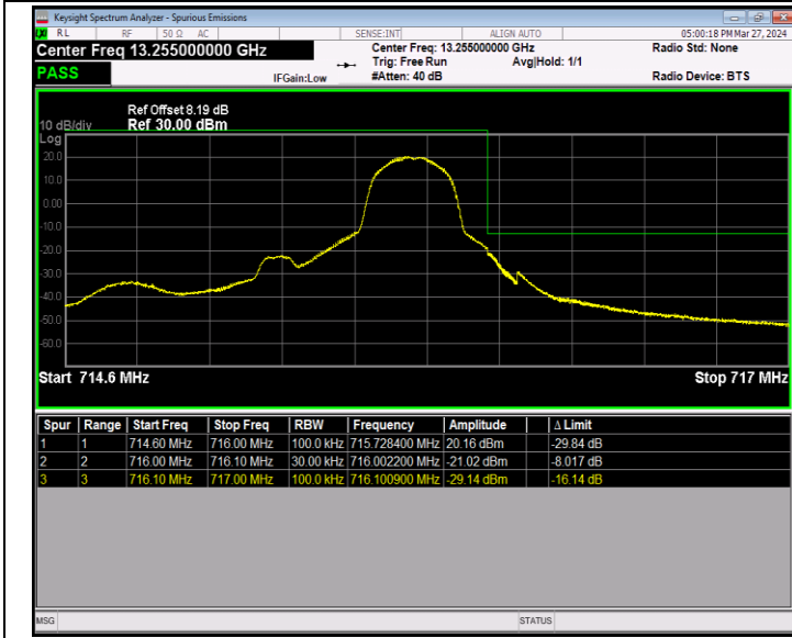
Band12_1.4MHz_QPSK_23173_1RB#5
