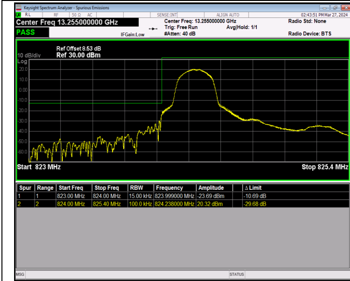
Band5_1.4MHz_QPSK_20407_1RB#0
