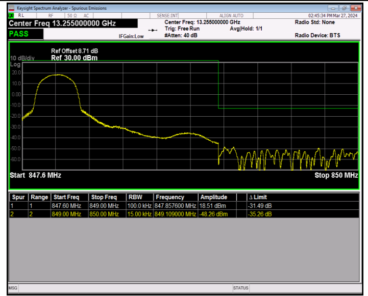
Band5_1.4MHz_16QAM_20643_1RB#0
