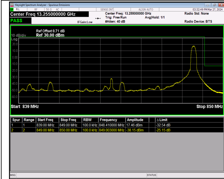
Band5_10MHz_64QAM_20600_1RB#49
