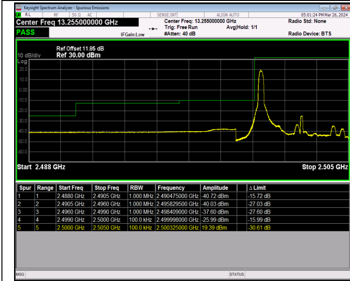
Band7_5MHz_QPSK_20775_1RB#0
