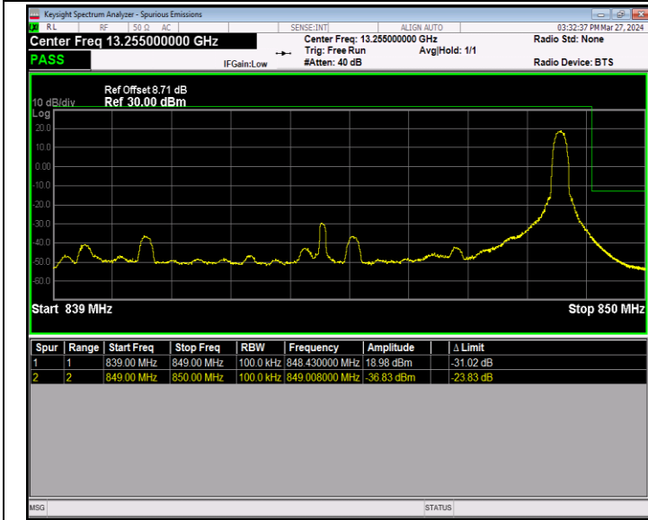
Band5_10MHz_16QAM_20600_1RB#49
