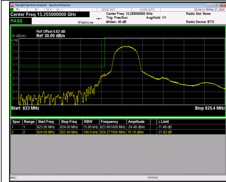
Band5_1.4MHz_64QAM_20407_1RB#0
