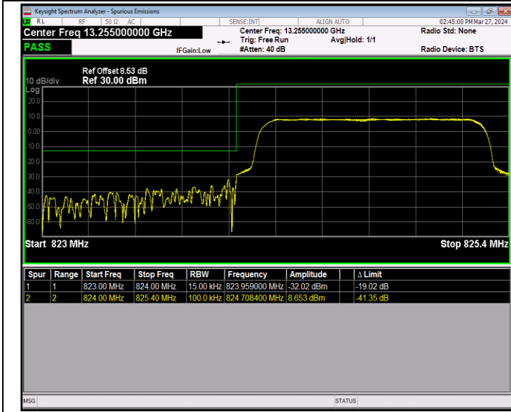
Band5_1.4MHz_16QAM_20407_6RB#0
