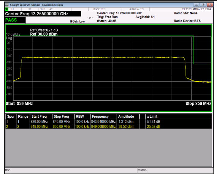
Band5_10MHz_64QAM_20600_50RB#0
