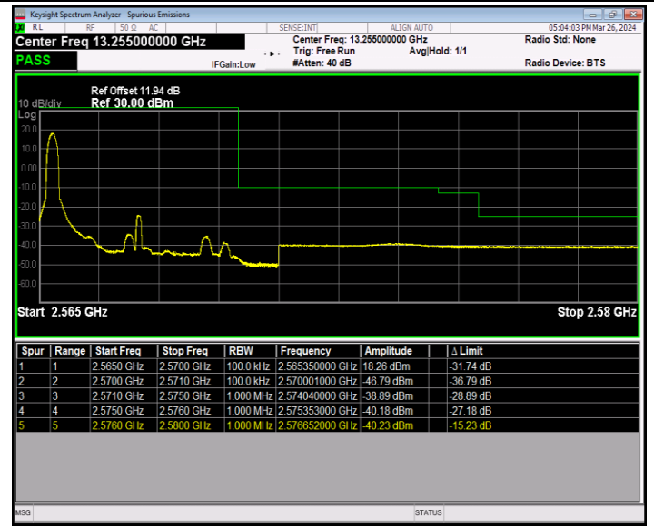
Band7_5MHz_16QAM_21425_1RB#0
