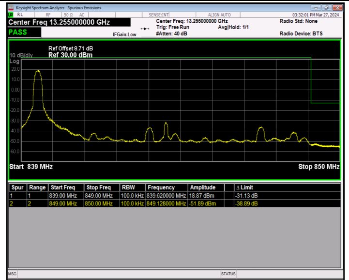
Band5_10MHz_16QAM_20600_1RB#0
