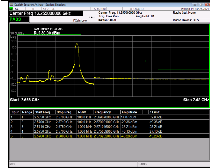
Band7_5MHz_64QAM_21425_1RB#24
