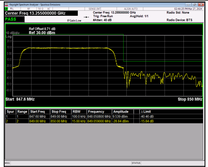
Band5_1.4MHz_QPSK_20643_6RB#0
