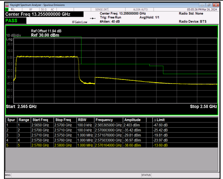
Band7_5MHz_16QAM_21425_25RB#0
