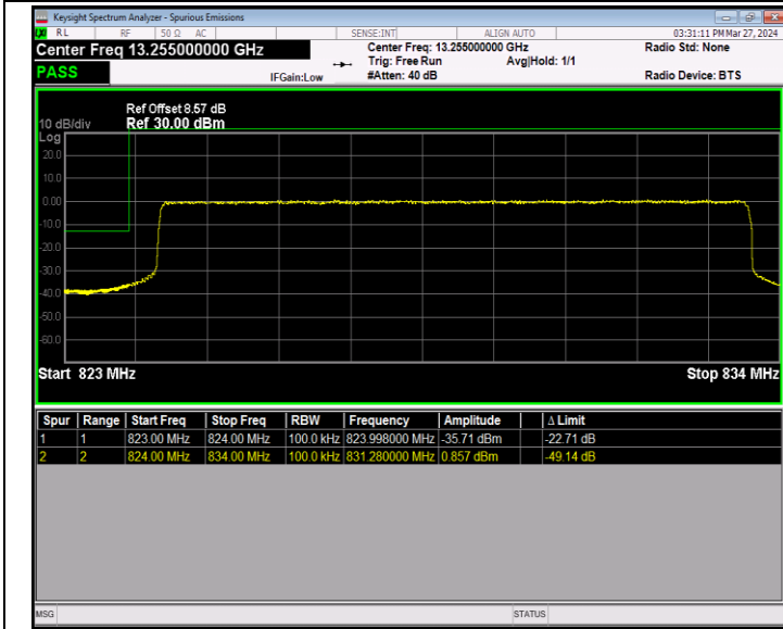
Band5_10MHz_QPSK_20450_50RB#0
