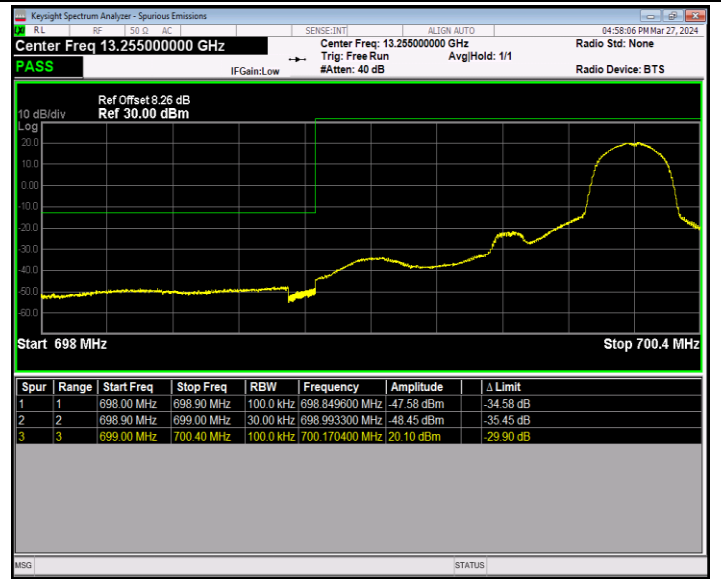
Band12_1.4MHz_QPSK_23017_1RB#5
