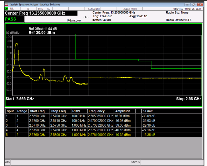
Band7_5MHz_64QAM_21425_1RB#0
