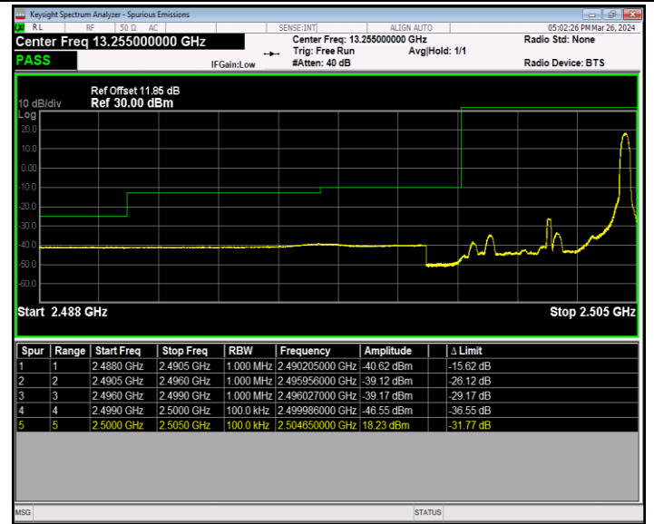
Band7_5MHz_16QAM_20775_1RB#24
