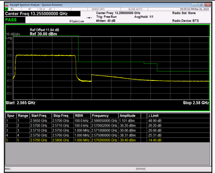
Band7_5MHz_64QAM_21425_25RB#0
