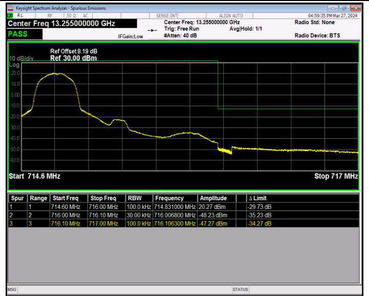
Band12_1.4MHz_QPSK_23173_1RB#0
