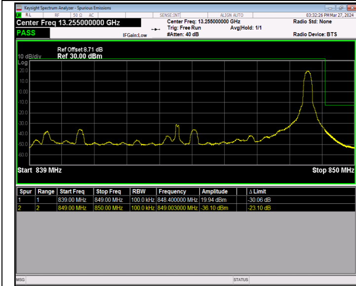
Band5_10MHz_QPSK_20600_1RB#49
