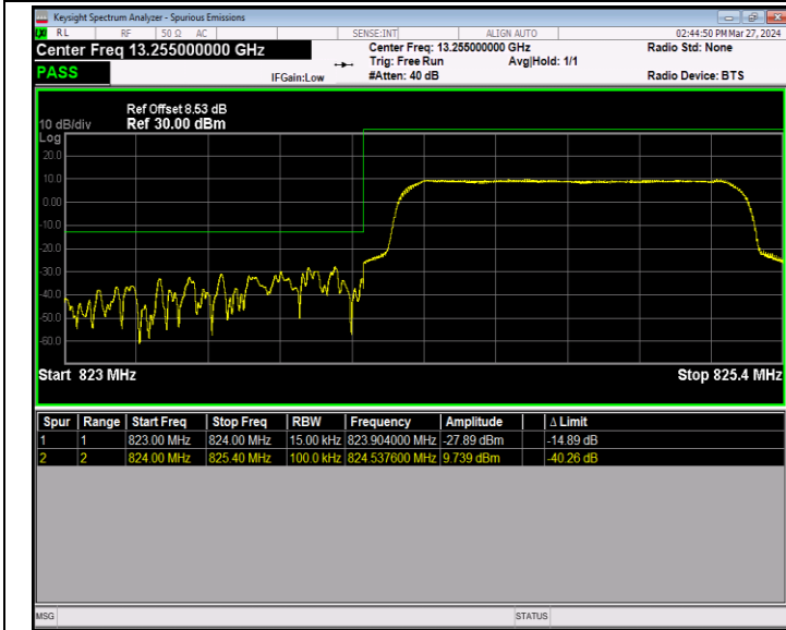
Band5_1.4MHz_QPSK_20407_6RB#0
