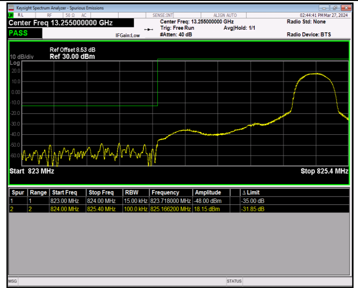
Band5_1.4MHz_64QAM_20407_1RB#5
