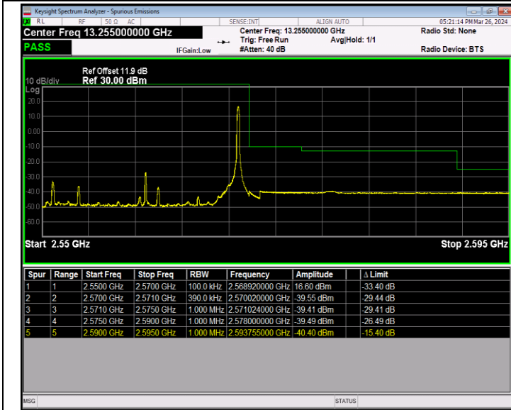
Band7_20MHz_64QAM_21350_1RB#99
