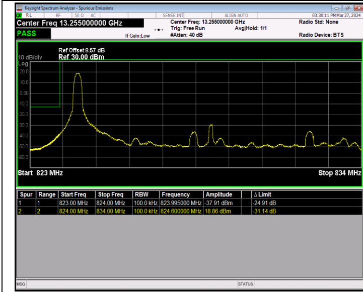
Band5_10MHz_16QAM_20450_1RB#0
