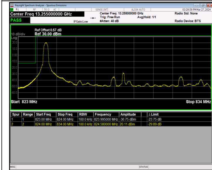
Band5_10MHz_QPSK_20450_1RB#0
