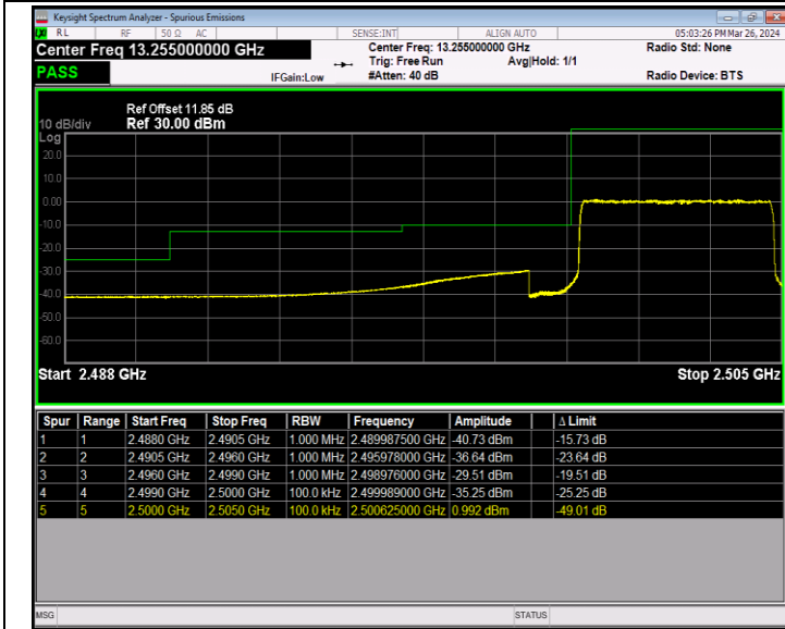
Band7_5MHz_64QAM_20775_25RB#0
