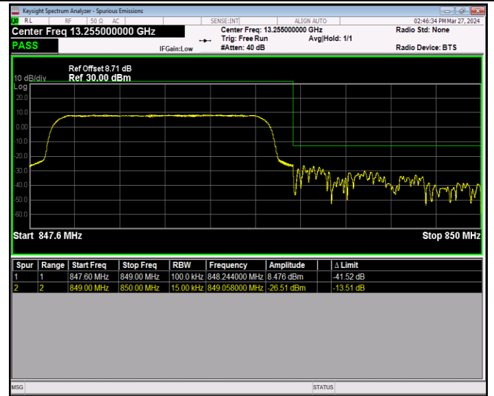
Band5_1.4MHz_16QAM_20643_6RB#0
