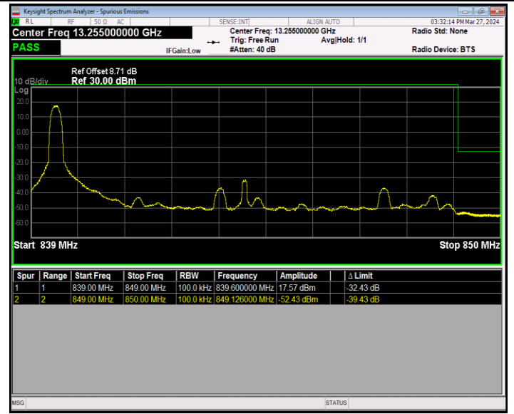
Band5_10MHz_64QAM_20600_1RB#0
