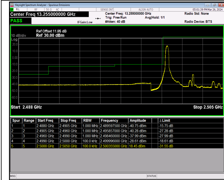
Band7_5MHz_16QAM_20775_1RB#0
