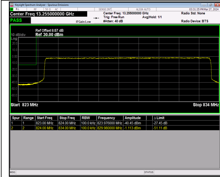
Band5_10MHz_64QAM_20450_50RB#0
