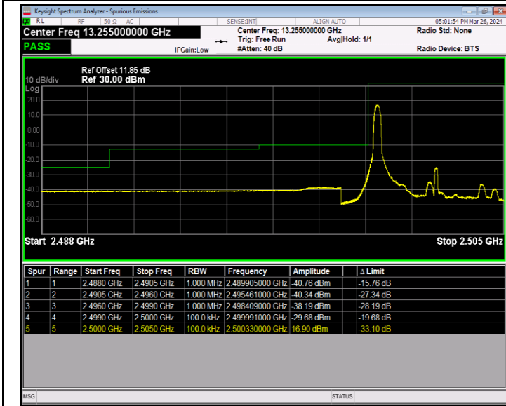
Band7_5MHz_64QAM_20775_1RB#0
