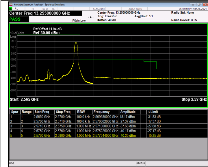
Band7_5MHz_16QAM_21425_1RB#24
