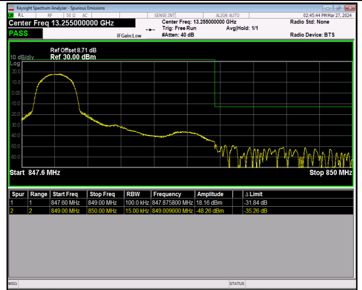
Band5_1.4MHz_64QAM_20643_1RB#0
