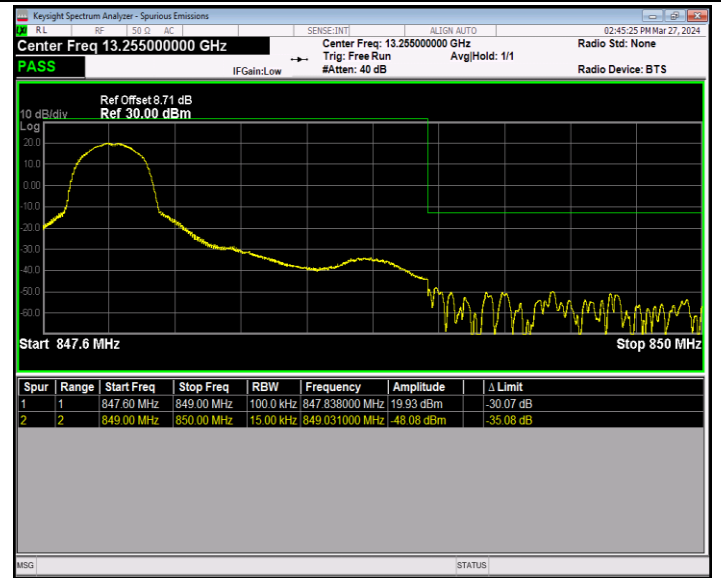
Band5_1.4MHz_QPSK_20643_1RB#0
