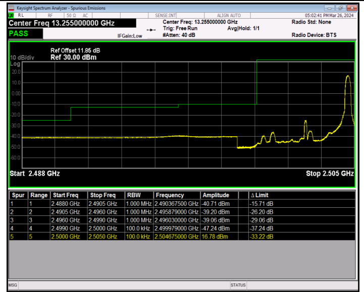
Band7_5MHz_64QAM_20775_1RB#24
