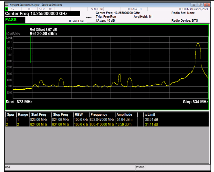
Band5_10MHz_16QAM_20450_1RB#49
