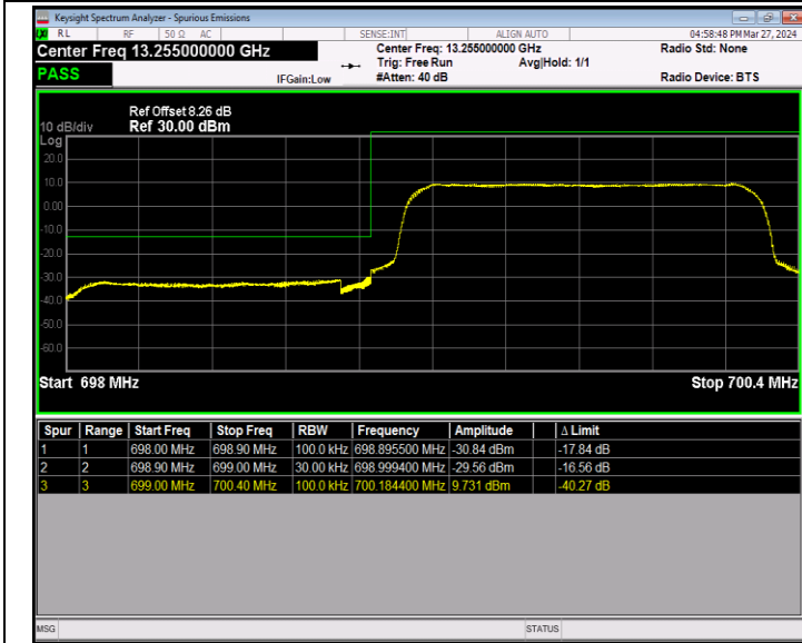
Band12_1.4MHz_QPSK_23017_6RB#0
