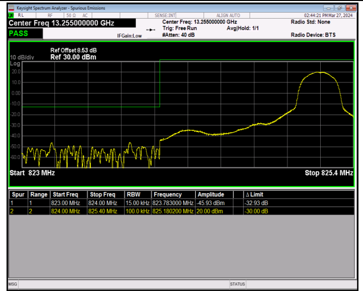
Band5_1.4MHz_QPSK_20407_1RB#5
