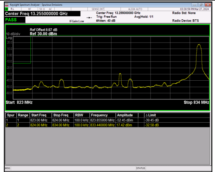
Band5_10MHz_64QAM_20450_1RB#49
