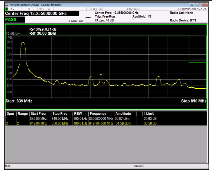
Band5_10MHz_QPSK_20600_1RB#0
