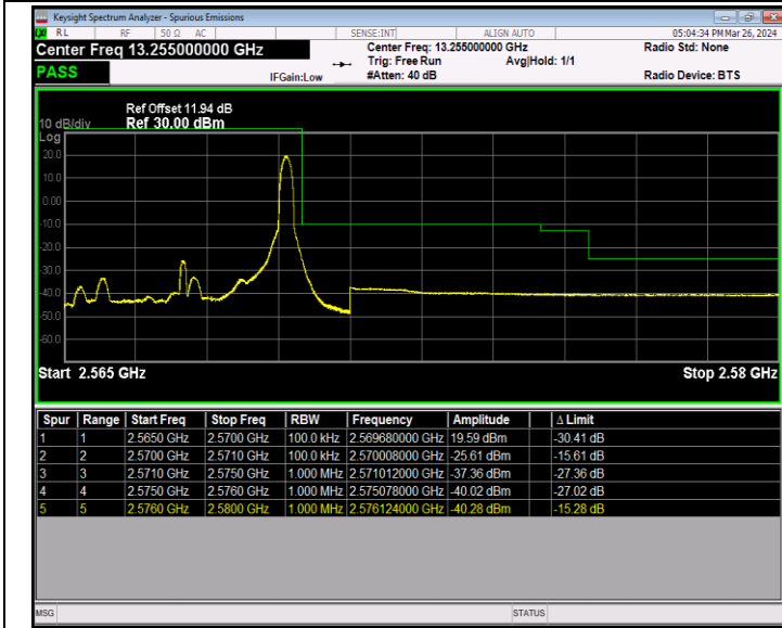
Band7_5MHz_QPSK_21425_1RB#24
