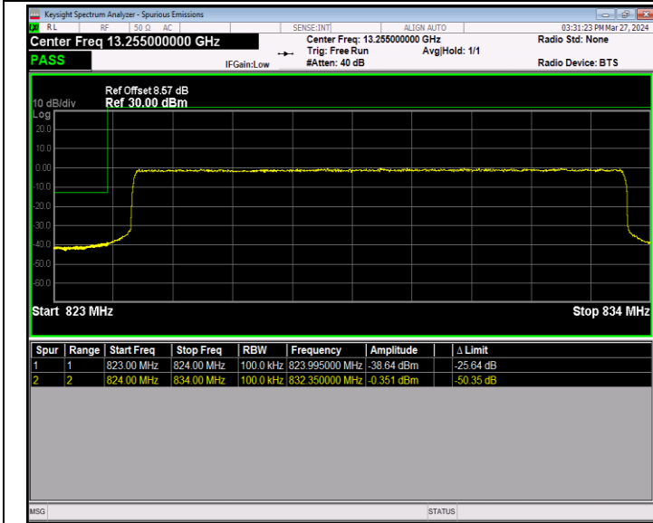
Band5_10MHz_16QAM_20450_50RB#0
