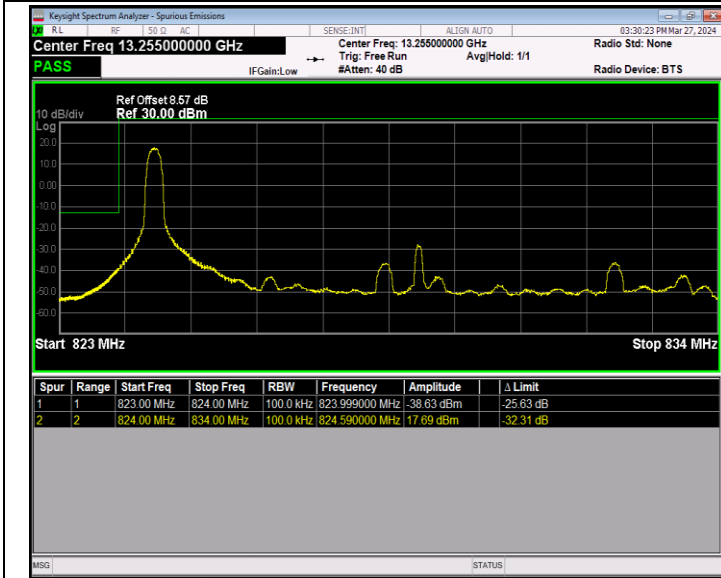
Band5_10MHz_64QAM_20450_1RB#0
