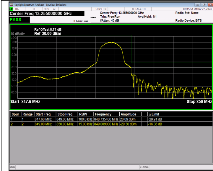
Band5_1.4MHz_QPSK_20643_1RB#5
