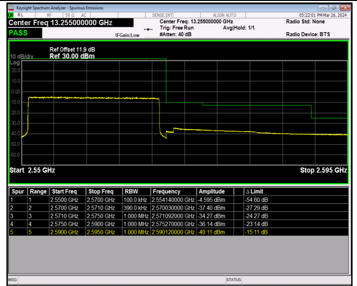
Band7_20MHz_64QAM_21350_100RB#0
