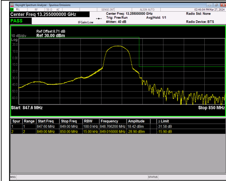
Band5_1.4MHz_16QAM_20643_1RB#5
