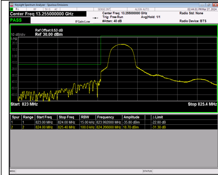
Band5_1.4MHz_16QAM_20407_1RB#0
