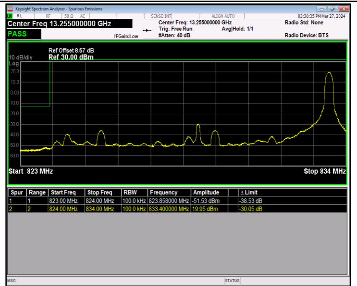
Band5_10MHz_QPSK_20450_1RB#49
