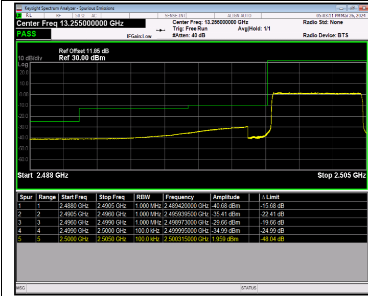
Band7_5MHz_16QAM_20775_25RB#0
