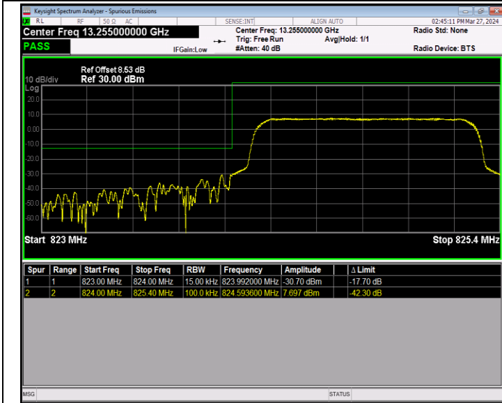
Band5_1.4MHz_64QAM_20407_6RB#0
