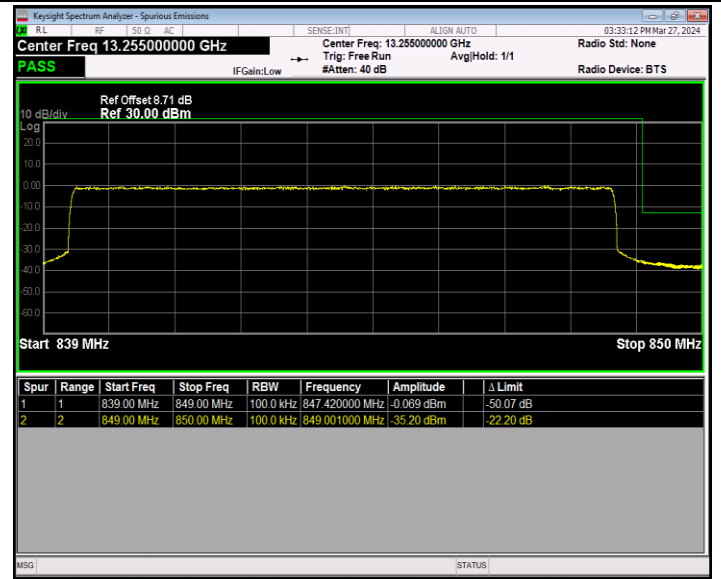
Band5_10MHz_16QAM_20600_50RB#0
