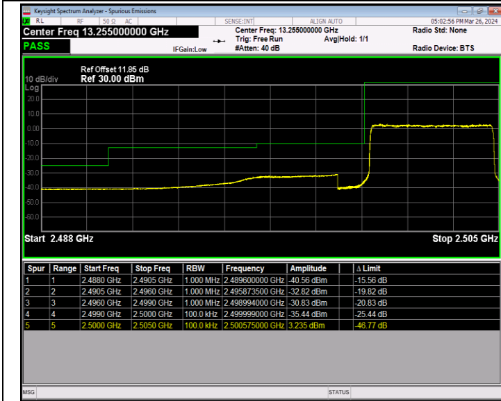
Band7_5MHz_QPSK_20775_25RB#0
