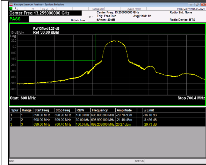
Band12_1.4MHz_QPSK_23017_1RB#0
