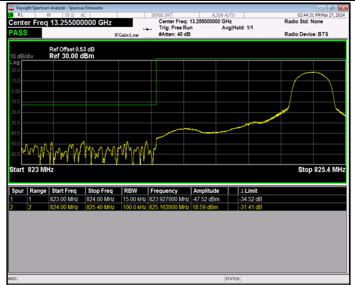
Band5_1.4MHz_16QAM_20407_1RB#5
