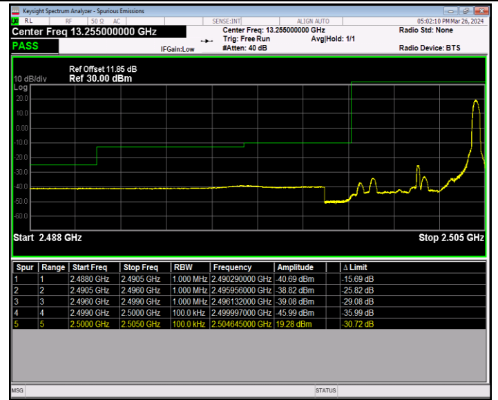
Band7_5MHz_QPSK_20775_1RB#24
