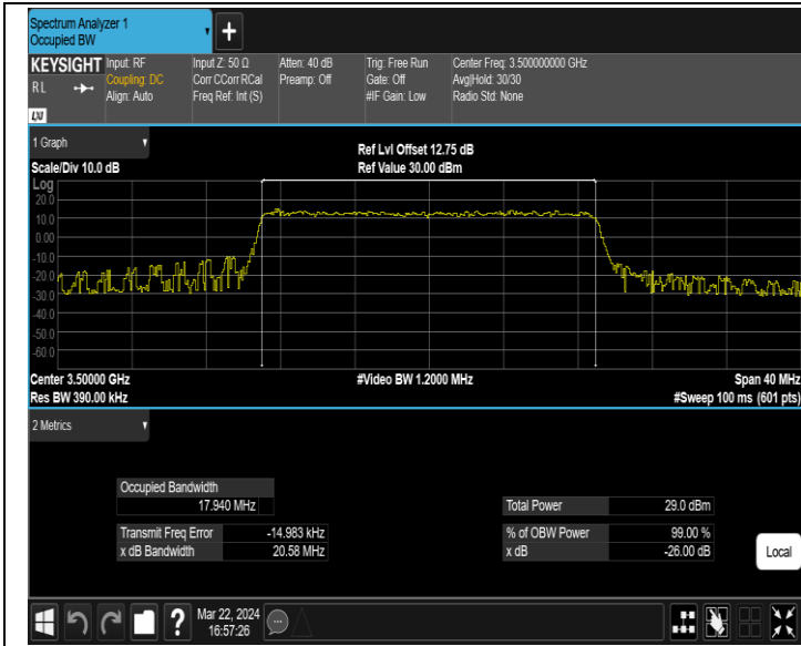
42(3450-3550)-20MHz-64QAM-42590-100RB#0-PASS
