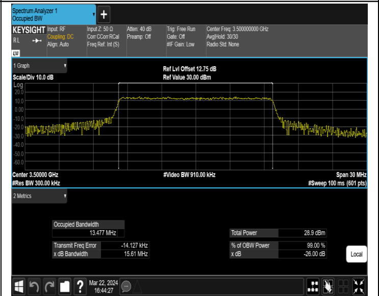
42(3450-3550)-15MHz-64QAM-42590-75RB#0-PASS
