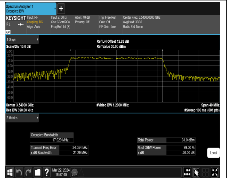
42(3450-3550)-20MHz-QPSK-42990-100RB#0-PASS
