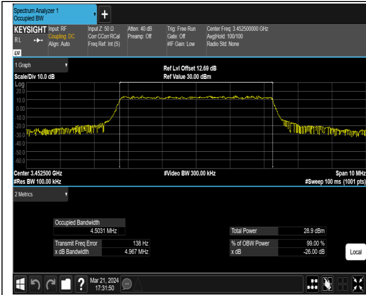
42(3450-3550)-5MHz-64QAM-42115-25RB#0-PASS
