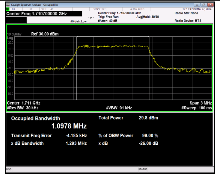
Band66-1.4MHz-16QAM-131979-6RB#0-PASS
