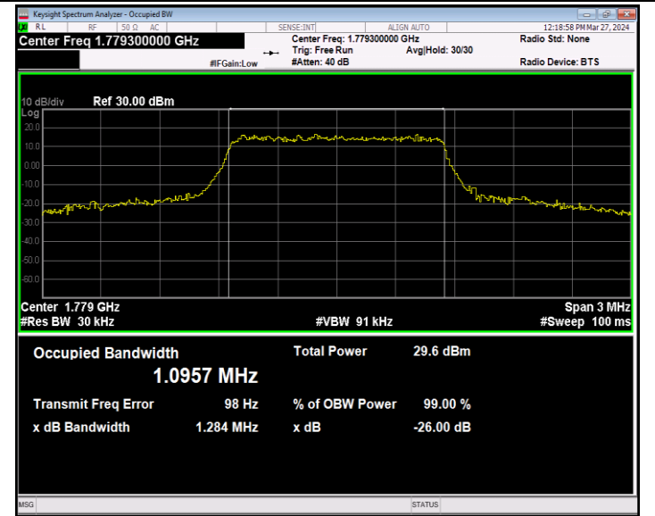
Band66-1.4MHz-16QAM-132665-6RB#0-PASS
