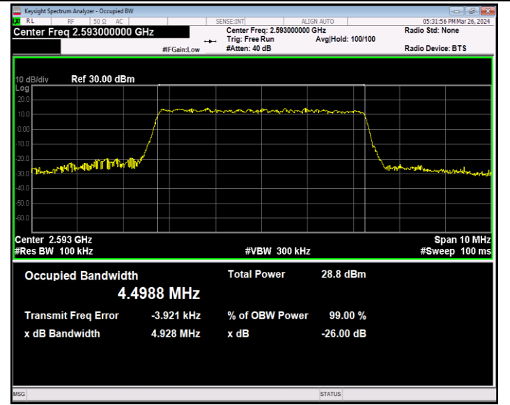
Band41-5MHz-64QAM-40620-25RB#0-PASS
