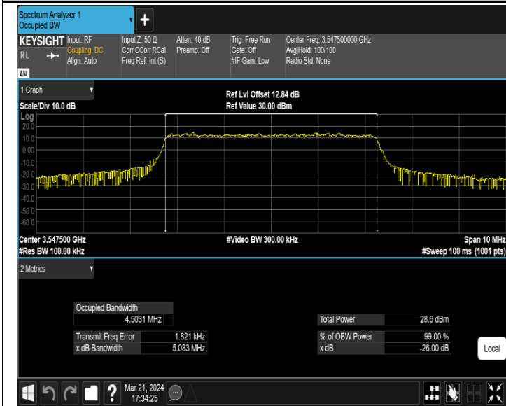
42(3450-3550)-5MHz-64QAM-43065-25RB#0-PASS
