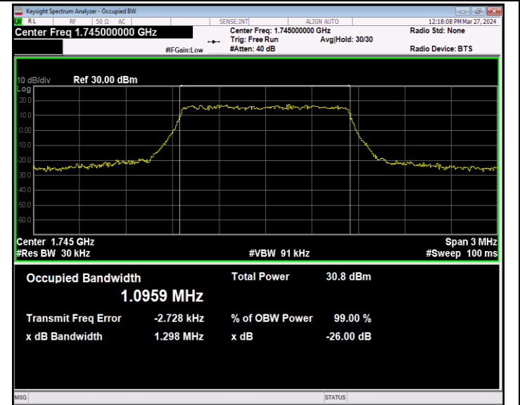
Band66-1.4MHz-QPSK-132322-6RB#0-PASS
