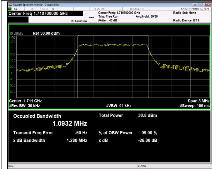
Band66-1.4MHz-QPSK-131979-6RB#0-PASS
