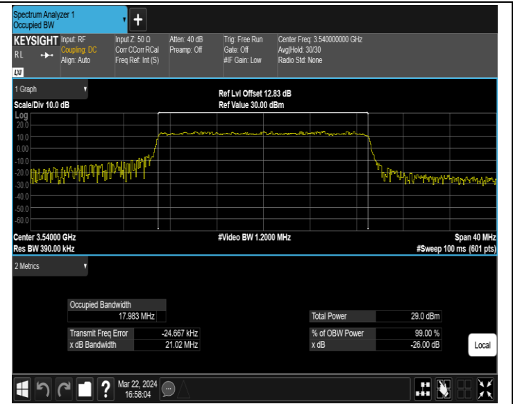
42(3450-3550)-20MHz-64QAM-42990-100RB#0-PASS
