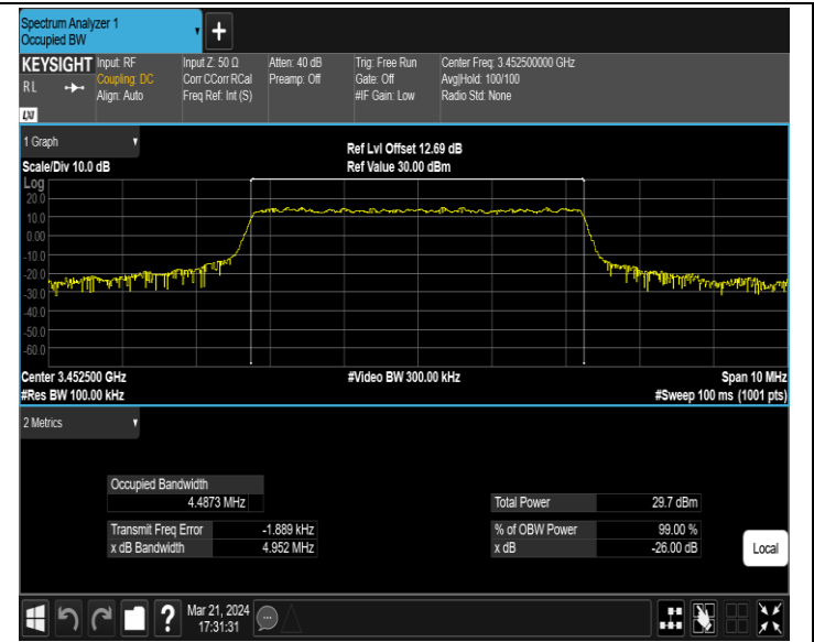
42(3450-3550)-5MHz-16QAM-42115-25RB#0-PASS
