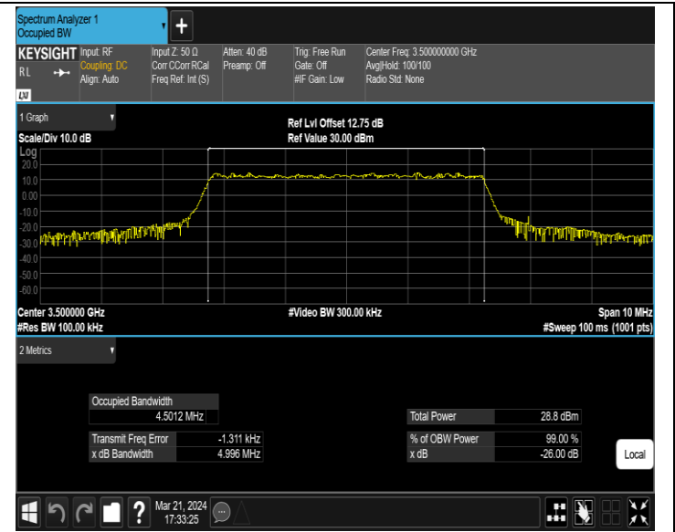
42(3450-3550)-5MHz-64QAM-42590-25RB#0-PASS
