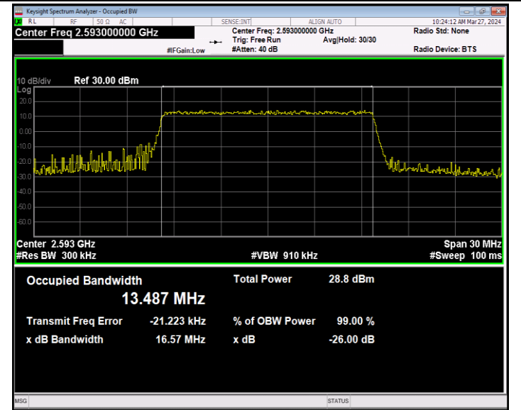
Band41-15MHz-64QAM-40620-75RB#0-PASS
