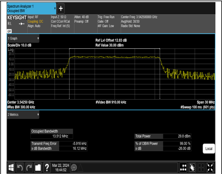
42(3450-3550)-15MHz-16QAM-43015-75RB#0-PASS
