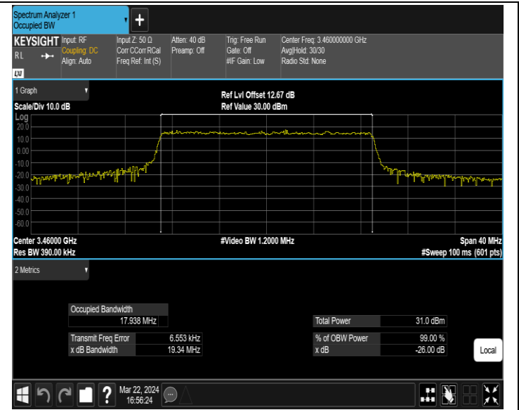
42(3450-3550)-20MHz-QPSK-42190-100RB#0-PASS
