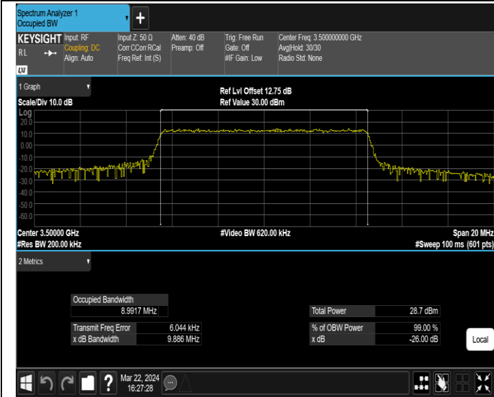
42(3450-3550)-10MHz-64QAM-42590-50RB#0-PASS
