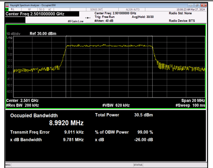
Band41-10MHz-QPSK-39700-50RB#0-PASS
