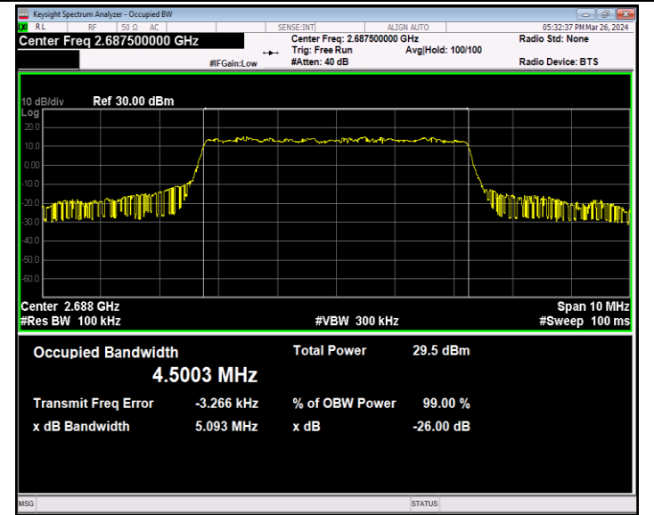
Band41-5MHz-16QAM-41565-25RB#0-PASS
