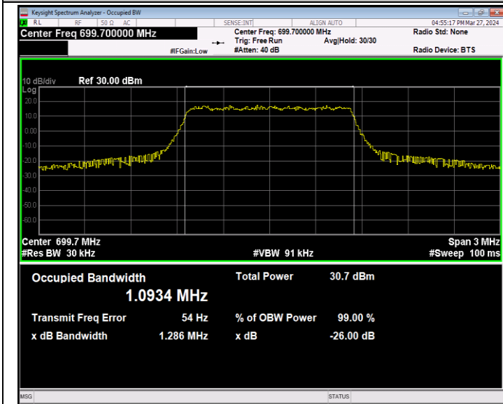
Band12-1.4MHz-QPSK-23017-6RB#0-PASS
