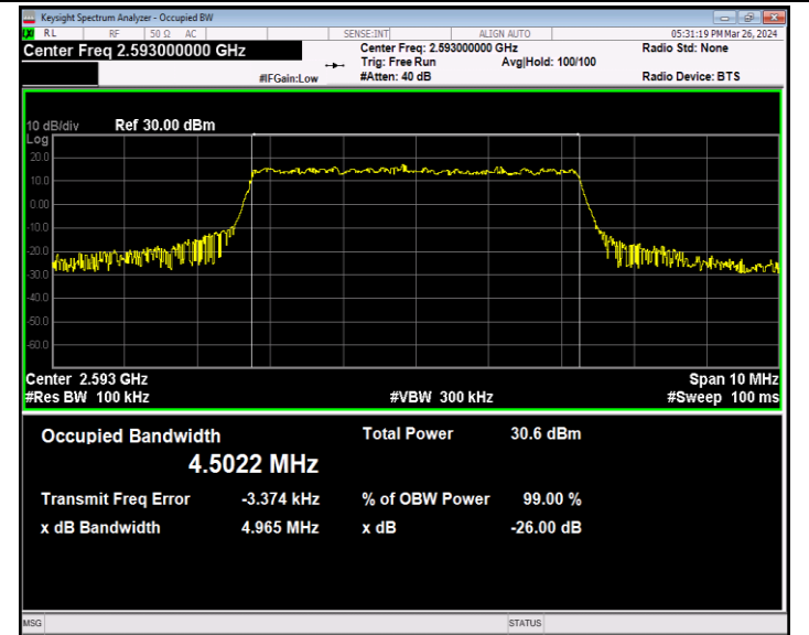
Band41-5MHz-QPSK-40620-25RB#0-PASS
