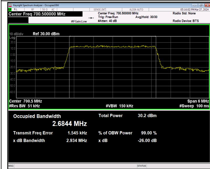
Band12-3MHz-16QAM-23025-15RB#0-PASS
