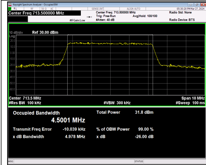
Band12-5MHz-QPSK-23155-25RB#0-PASS
