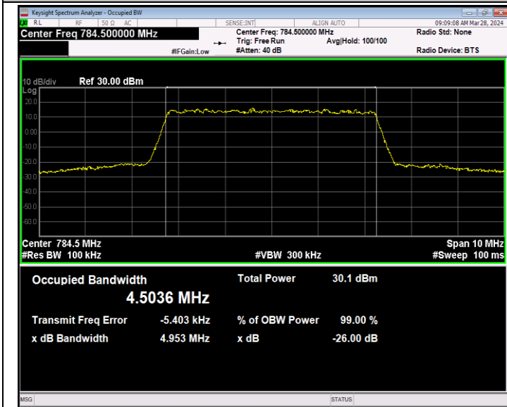
Band13-5MHz-64QAM-23255-25RB#0-PASS
