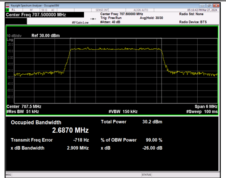
Band12-3MHz-16QAM-23095-15RB#0-PASS
