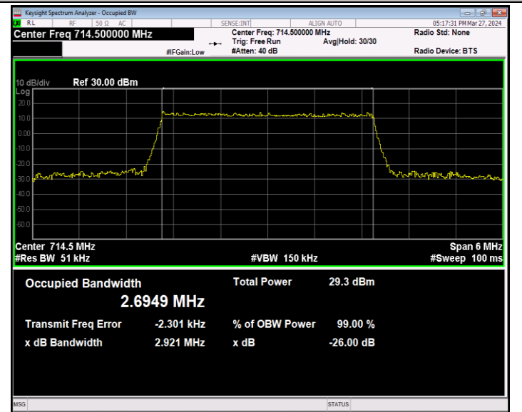
Band12-3MHz-64QAM-23165-15RB#0-PASS
