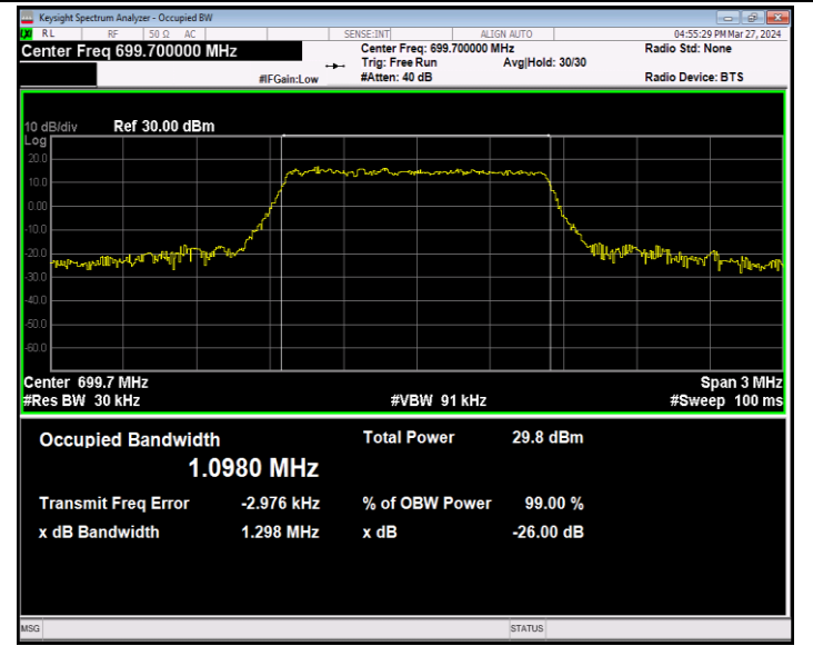
Band12-1.4MHz-16QAM-23017-6RB#0-PASS
