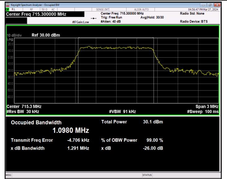
Band12-1.4MHz-16QAM-23173-6RB#0-PASS
