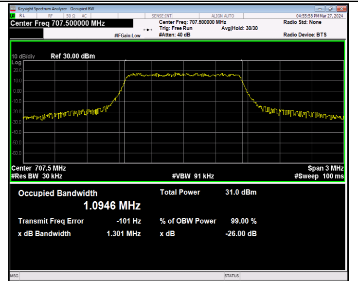
Band12-1.4MHz-QPSK-23095-6RB#0-PASS
