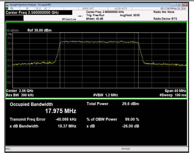
Band7-20MHz-64QAM-21350-100RB#0-PASS
