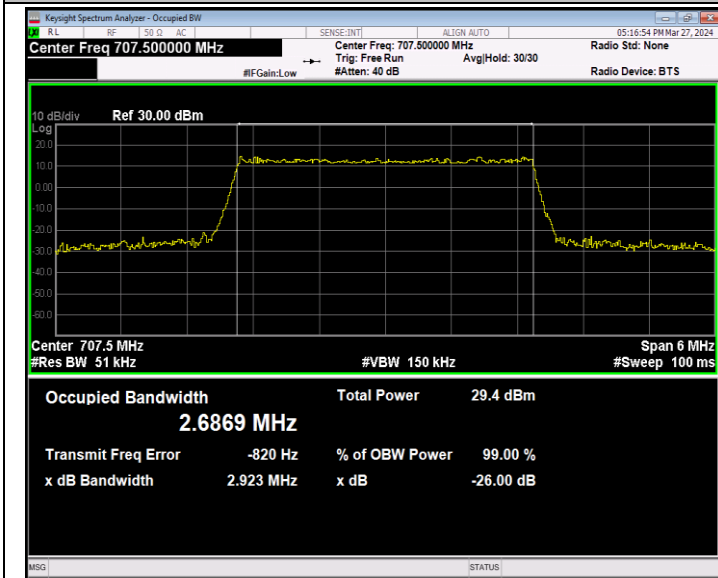
Band12-3MHz-64QAM-23095-15RB#0-PASS
