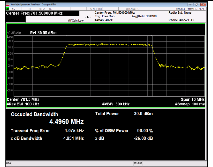
Band12-5MHz-16QAM-23035-25RB#0-PASS
