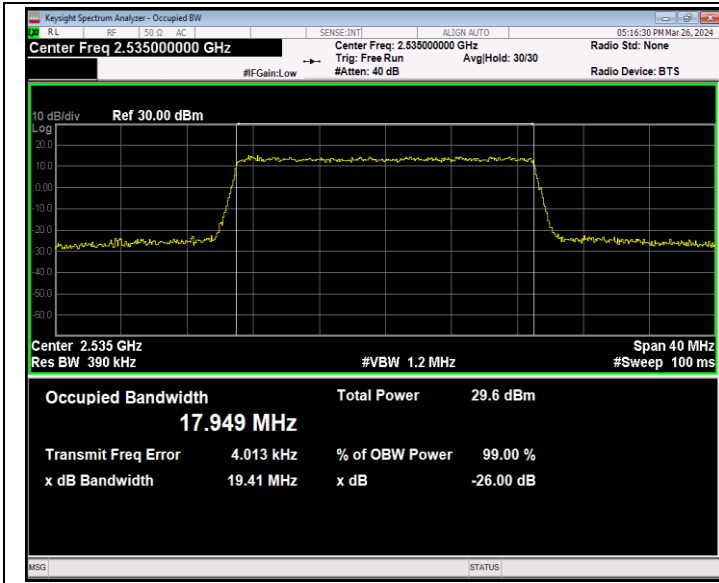
Band7-20MHz-64QAM-21100-100RB#0-PASS
