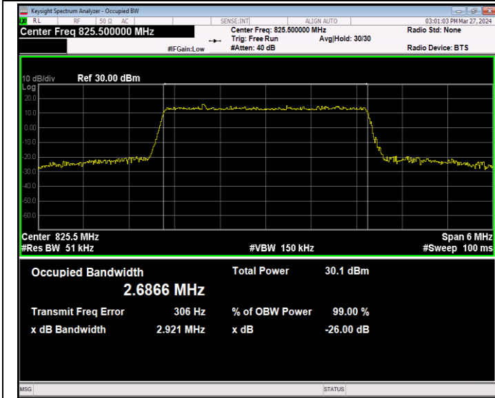
Band5-3MHz-16QAM-20415-15RB#0-PASS
