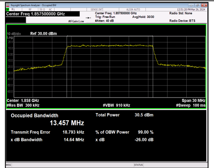
Band2-15MHz-16QAM-18675-75RB#0-PASS
