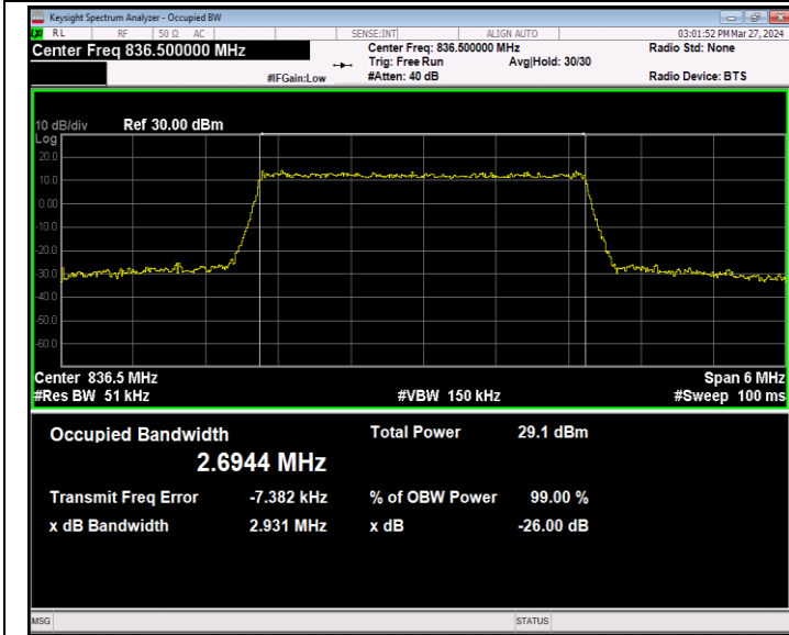
Band5-3MHz-64QAM-20525-15RB#0-PASS
