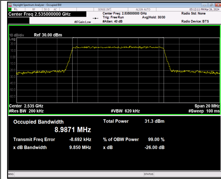
Band7-10MHz-QPSK-21100-50RB#0-PASS
