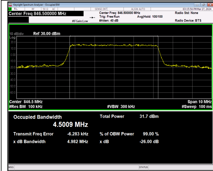
Band5-5MHz-QPSK-20625-25RB#0-PASS
