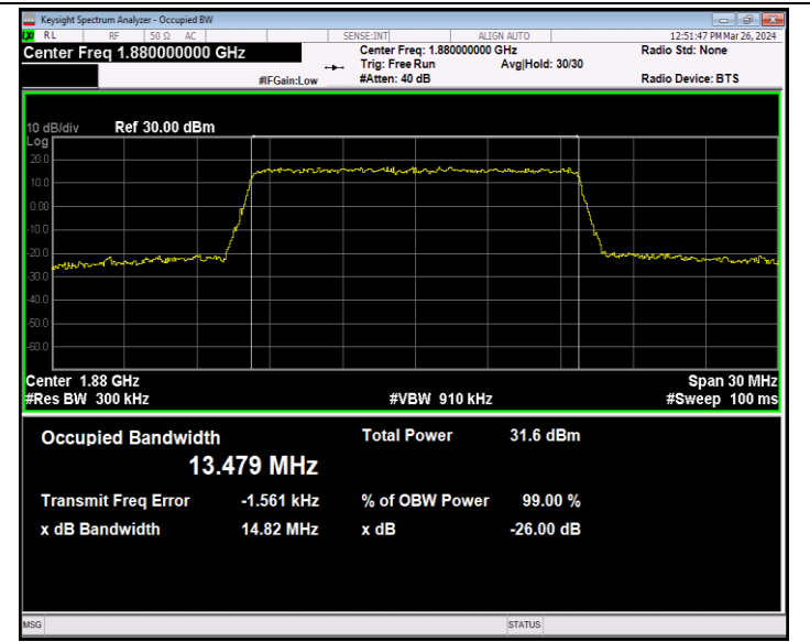
Band2-15MHz-QPSK-18900-75RB#0-PASS
