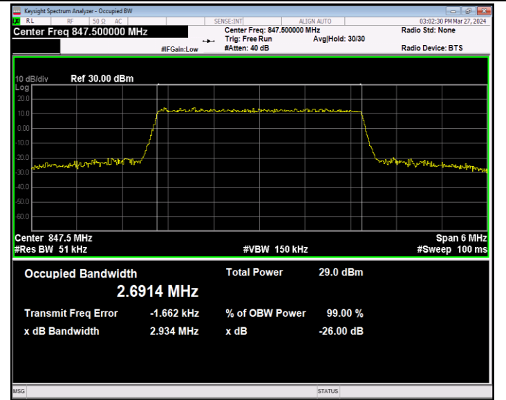
Band5-3MHz-64QAM-20635-15RB#0-PASS
