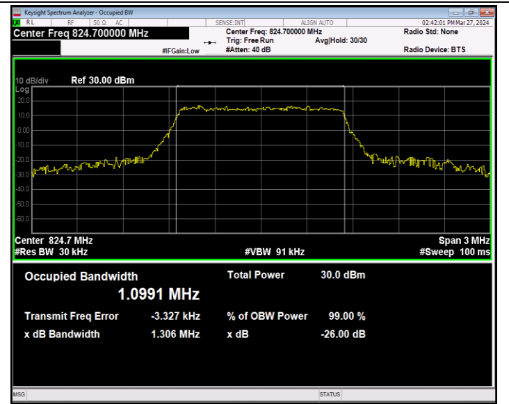
Band5-1.4MHz-16QAM-20407-6RB#0-PASS
