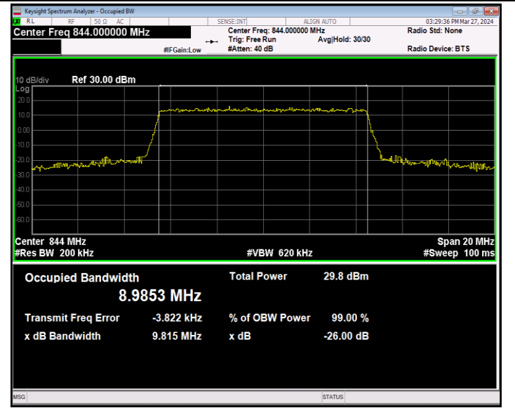
Band5-10MHz-64QAM-20600-50RB#0-PASS
