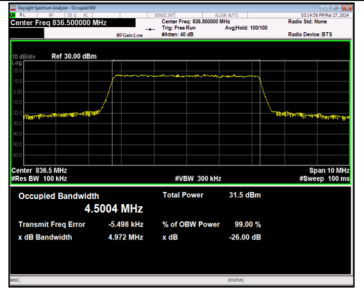
Band5-5MHz-QPSK-20525-25RB#0-PASS
