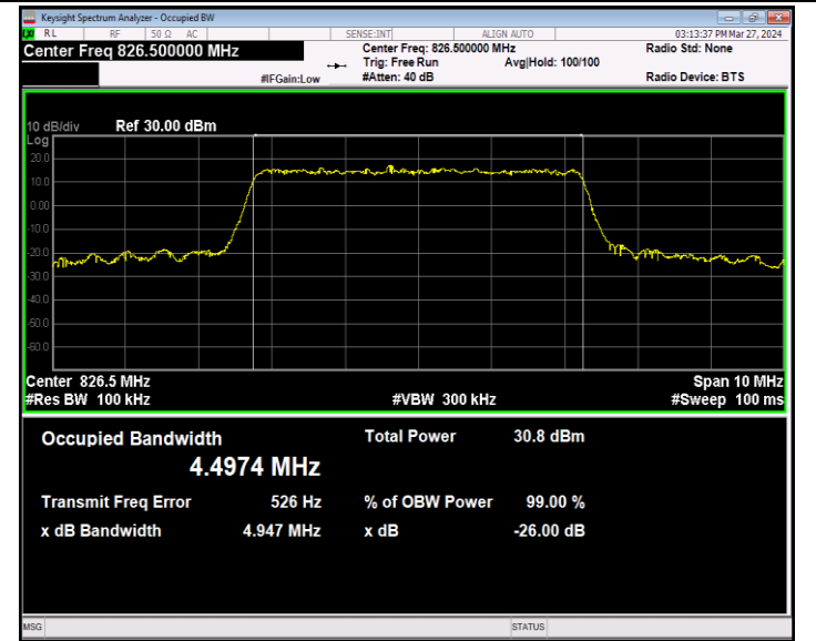
Band5-5MHz-16QAM-20425-25RB#0-PASS
