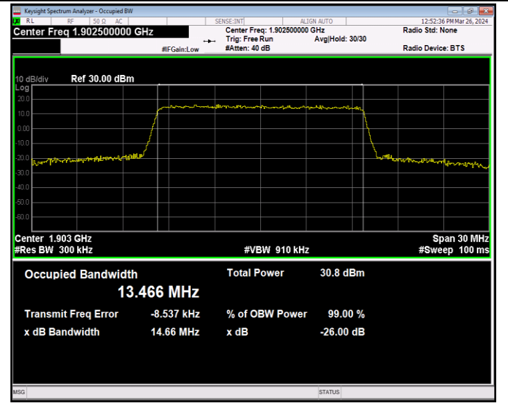
Band2-15MHz-16QAM-19125-75RB#0-PASS
