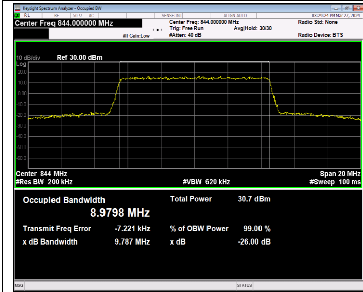
Band5-10MHz-16QAM-20600-50RB#0-PASS
