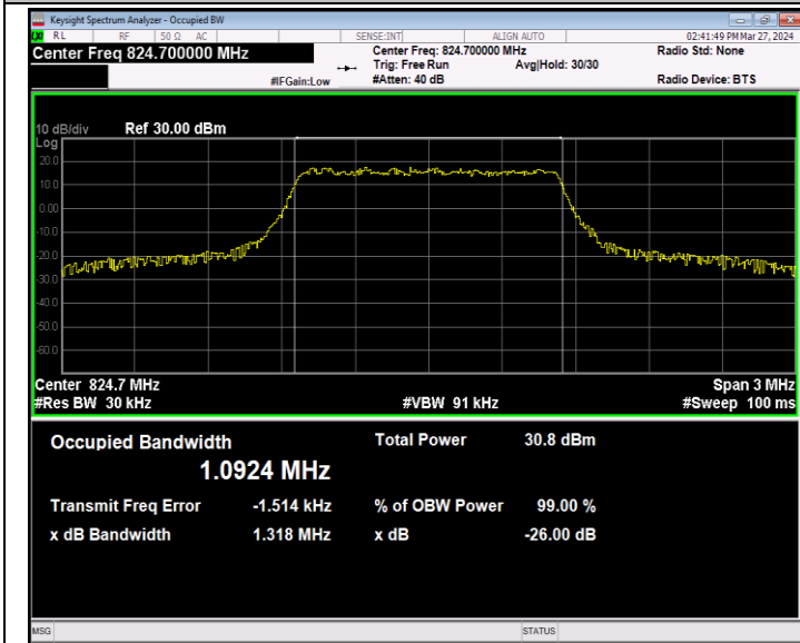
Band5-1.4MHz-QPSK-20407-6RB#0-PASS
