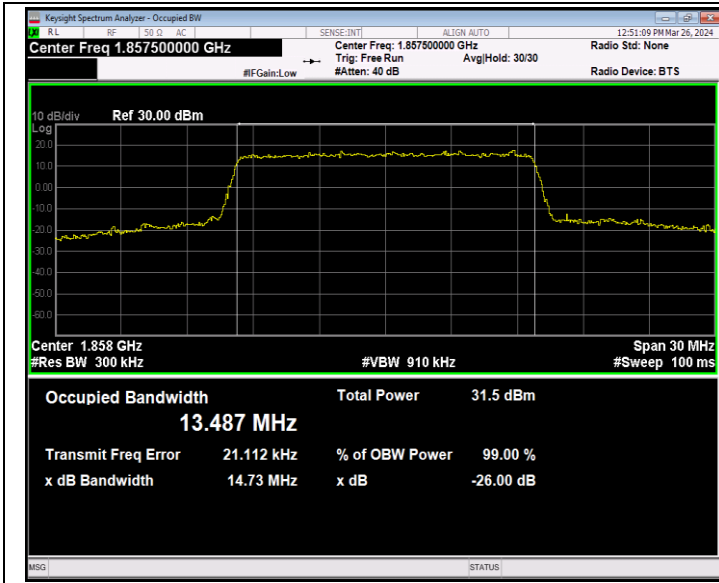
Band2-15MHz-QPSK-18675-75RB#0-PASS
