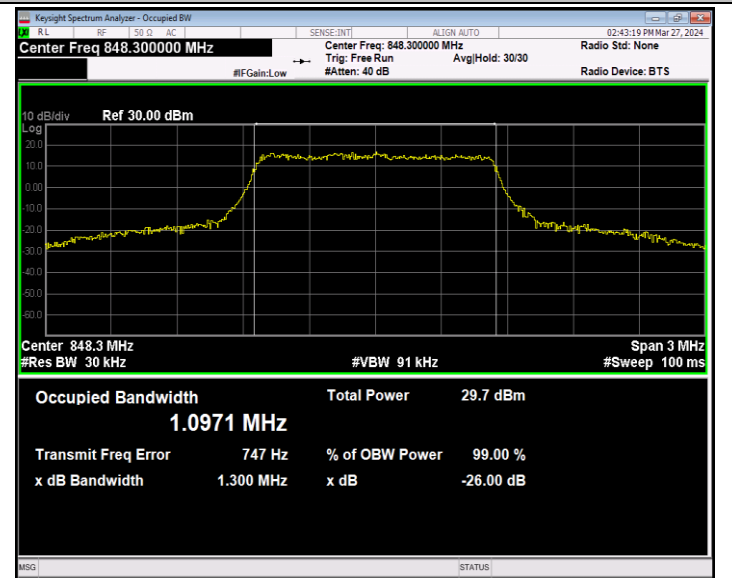
Band5-1.4MHz-16QAM-20643-6RB#0-PASS
