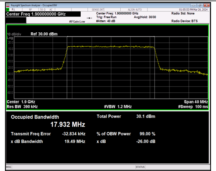
Band2-20MHz-64QAM-19100-100RB#0-PASS
