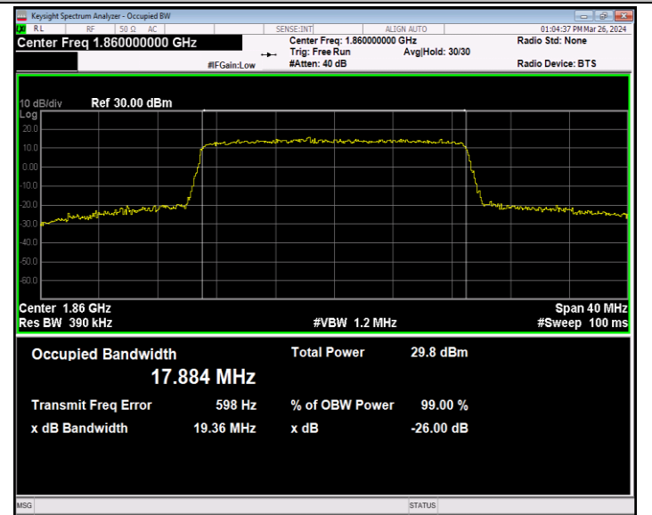
Band2-20MHz-64QAM-18700-100RB#0-PASS
