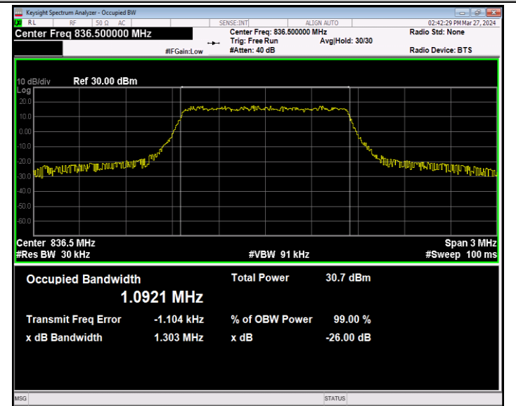
Band5-1.4MHz-QPSK-20525-6RB#0-PASS
