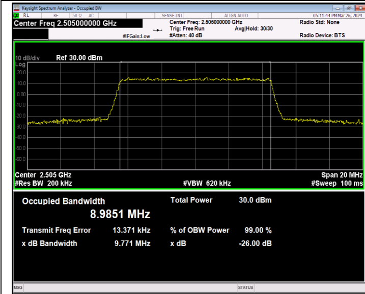
Band7-10MHz-16QAM-20800-50RB#0-PASS
