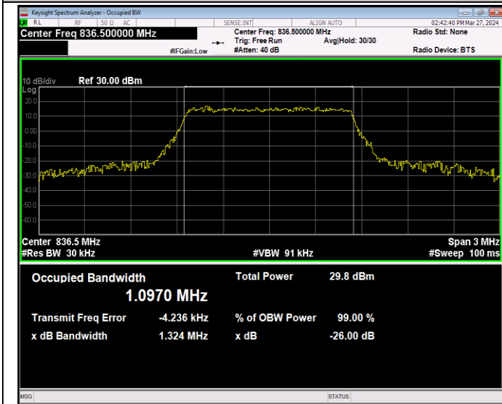
Band5-1.4MHz-16QAM-20525-6RB#0-PASS
