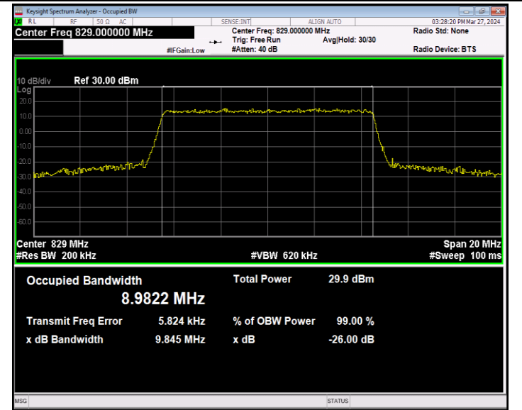
Band5-10MHz-64QAM-20450-50RB#0-PASS
