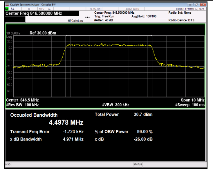
Band5-5MHz-16QAM-20625-25RB#0-PASS
