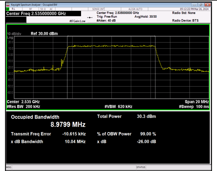
Band7-10MHz-16QAM-21100-50RB#0-PASS
