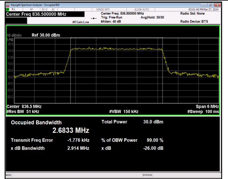
Band5-3MHz-16QAM-20525-15RB#0-PASS
