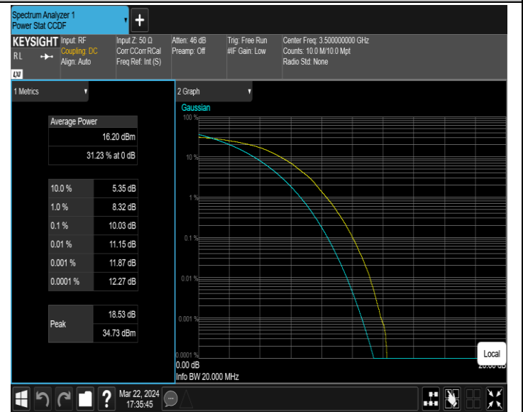
42(3450-3550)-20MHz-64QAM-42590-100RB#0-PASS
