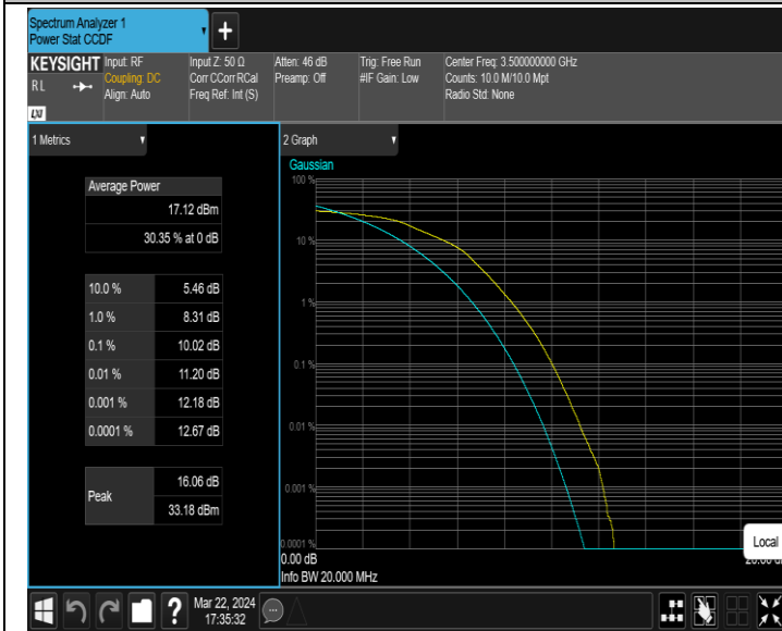
42(3450-3550)-20MHz-16QAM-42590-100RB#0-PASS
