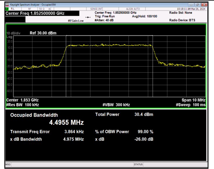
Band2-5MHz-16QAM-18625-25RB#0-PASS
