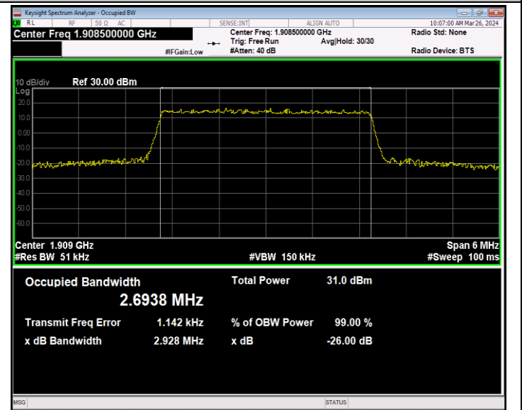
Band2-3MHz-QPSK-19185-15RB#0-PASS
