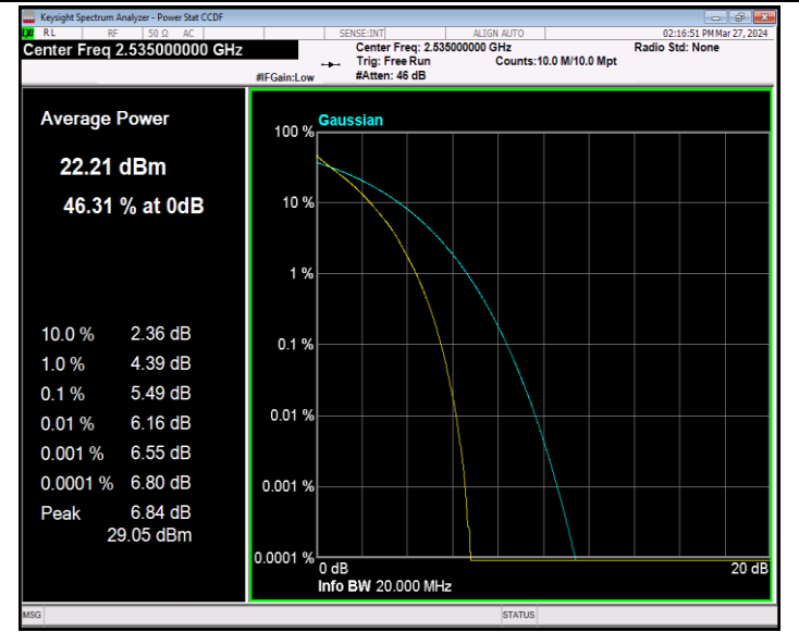
Band7-20MHz-QPSK-21100-100RB#0-PASS
