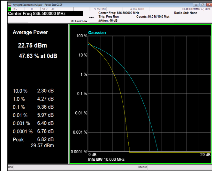
Band5-10MHz-QPSK-20525-50RB#0-PASS
