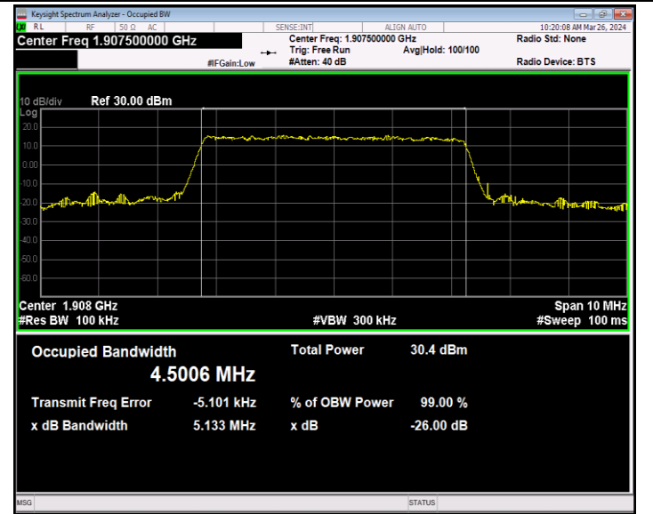
Band2-5MHz-16QAM-19175-25RB#0-PASS
