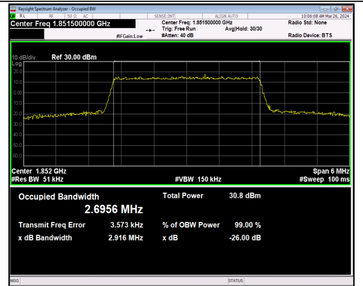
Band2-3MHz-64QAM-18615-15RB#0-PASS
