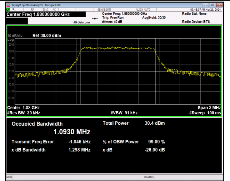
Band2-1.4MHz-64QAM-18900-6RB#0-PASS
