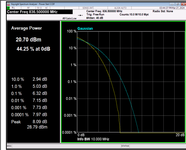
Band5-10MHz-64QAM-20525-50RB#0-PASS
