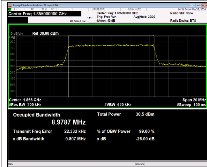
Band2-10MHz-16QAM-18650-50RB#0-PASS
