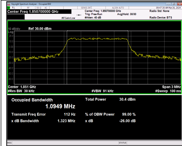
Band2-1.4MHz-64QAM-18607-6RB#0-PASS
