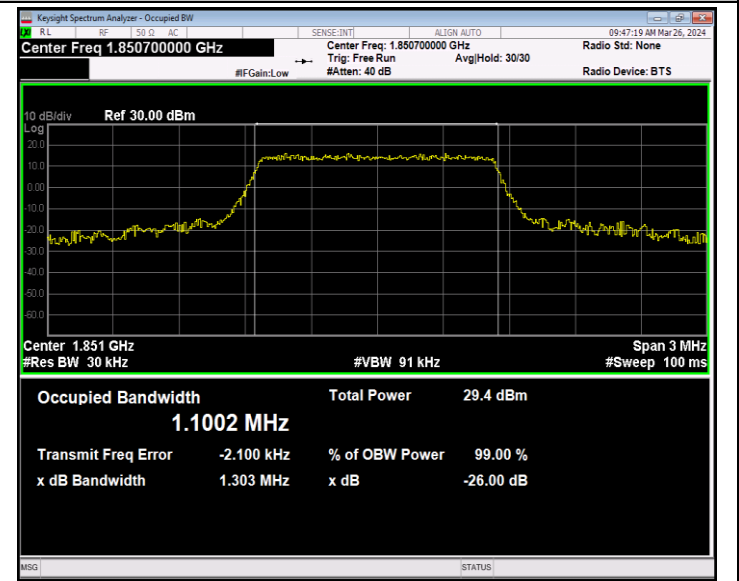
Band2-1.4MHz-16QAM-18607-6RB#0-PASS
