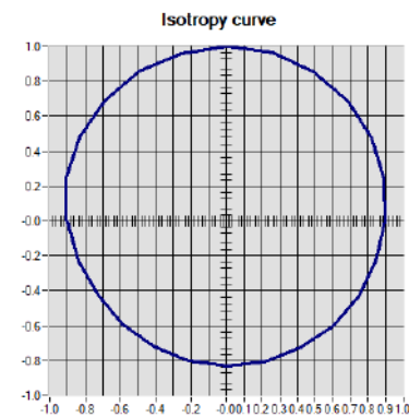
Isotropy +/-0.34% (+/-0.43dB)
