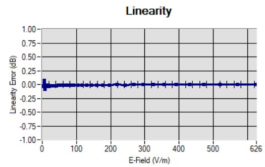
Linearity: +/-1.87% (+/-0.08dB)
