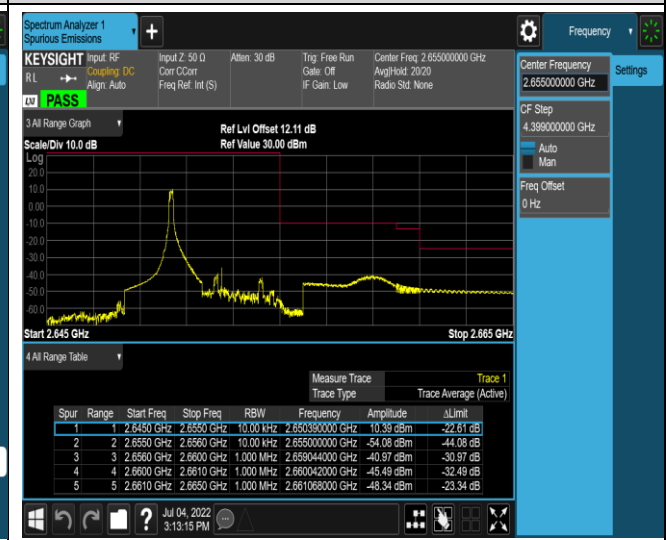
Band41-5MHz-16QAM-41215-25RB#0
