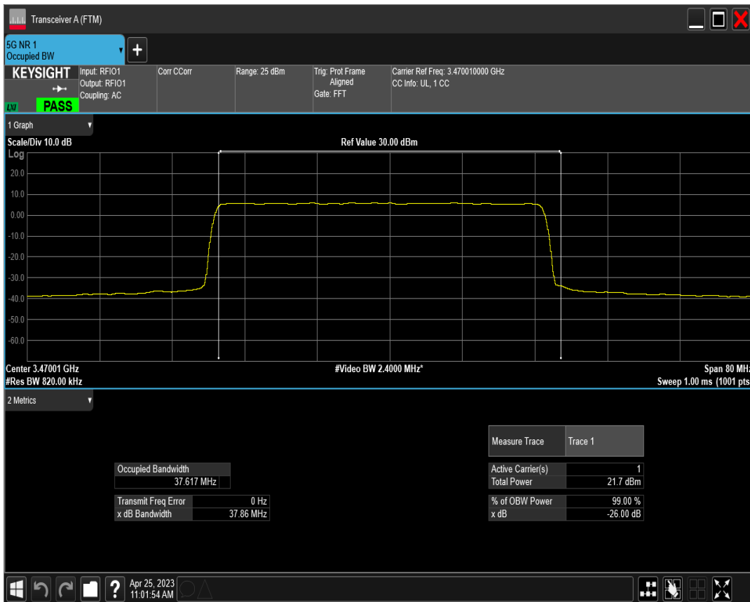
n77(3450-3550) SCS=30kHz CP_QPSK BW=40MHz Channel=631334 RB=106@0
