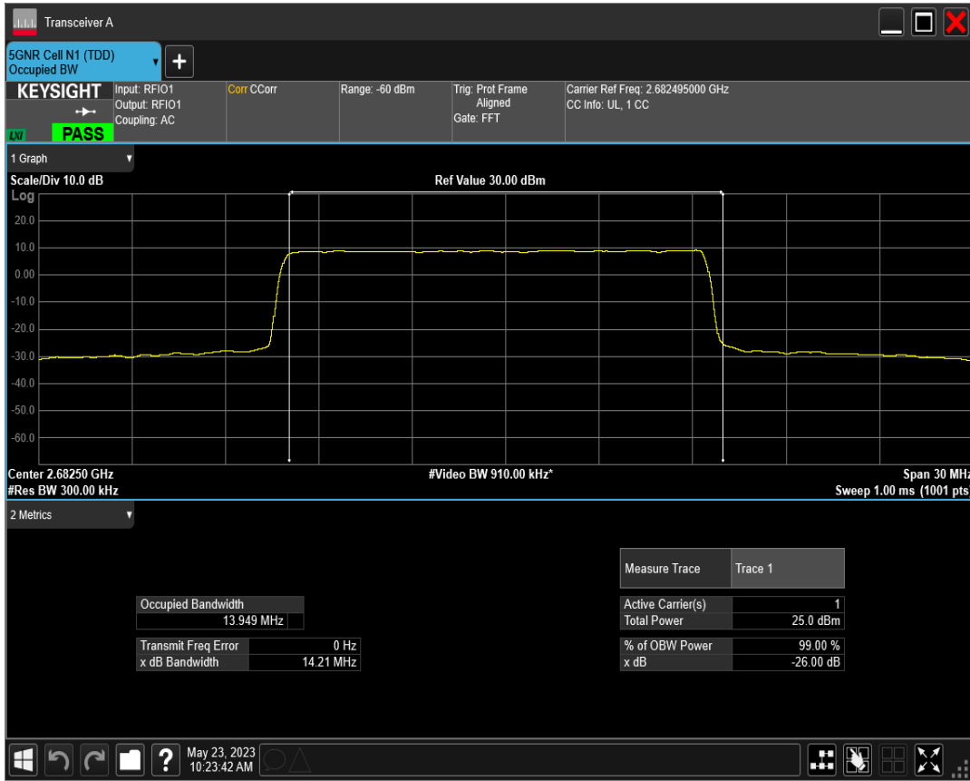
n41 SCS=15kHz DFT_QAM16 BW=15MHz Channel=536499 RB=75@0
