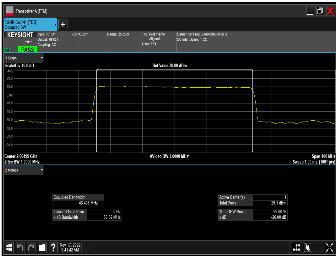
n41 SCS=15kHz DFT_QPSK BW=50MHz Channel=532998 RB=270@0
