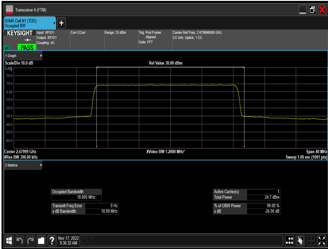
n41 SCS=15kHz DFT_QAM64 BW=20MHz Channel=535998 RB=100@0
