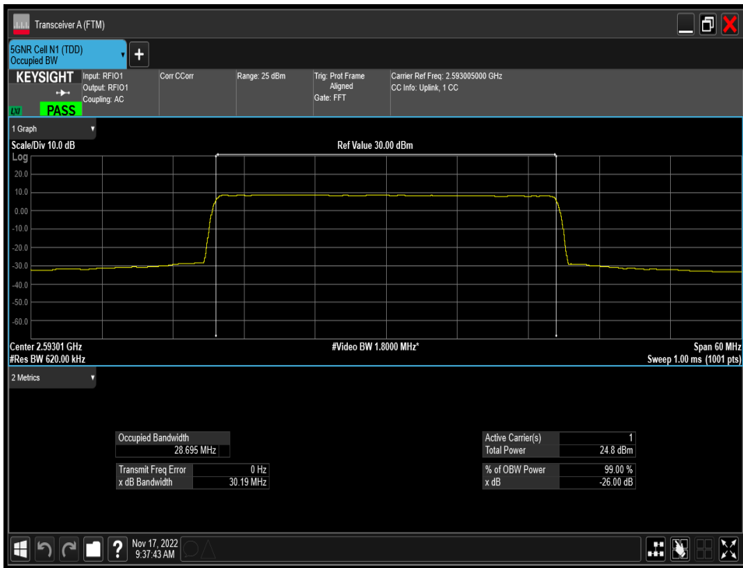
n41 SCS=15kHz DFT_QAM64 BW=30MHz Channel=518601 RB=160@0
