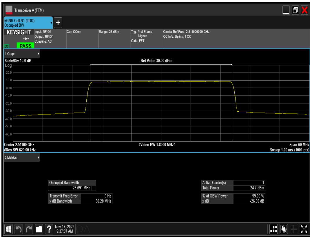
n41 SCS=15kHz DFT_QAM64 BW=30MHz Channel=502200 RB=160@0
