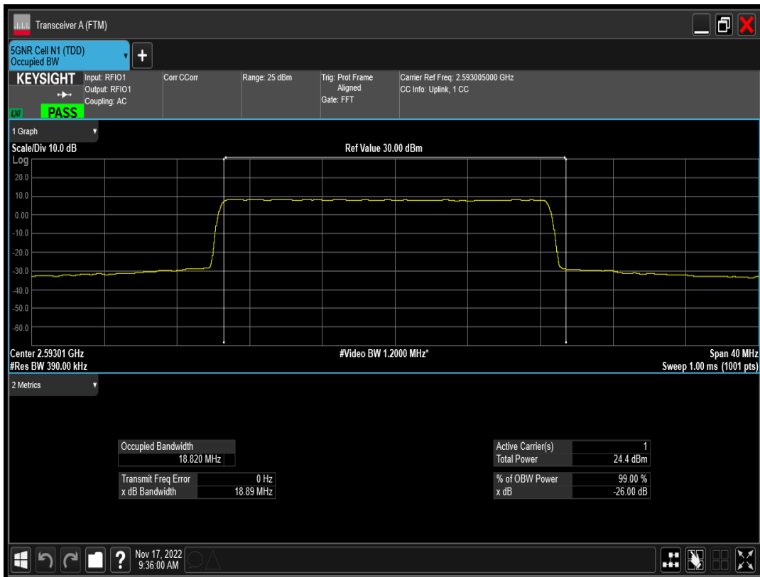
n41 SCS=15kHz DFT_QAM64 BW=20MHz Channel=518601 RB=100@0
