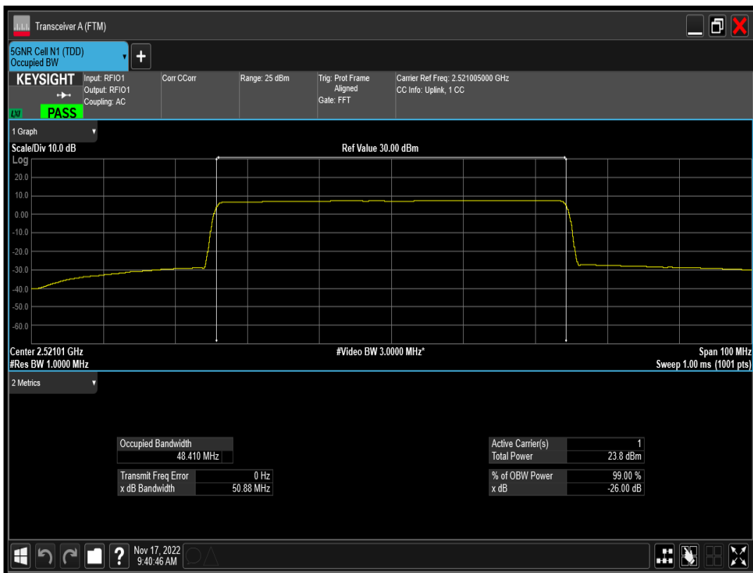
n41 SCS=15kHz CP_QPSK BW=50MHz Channel=504201 RB=270@0
