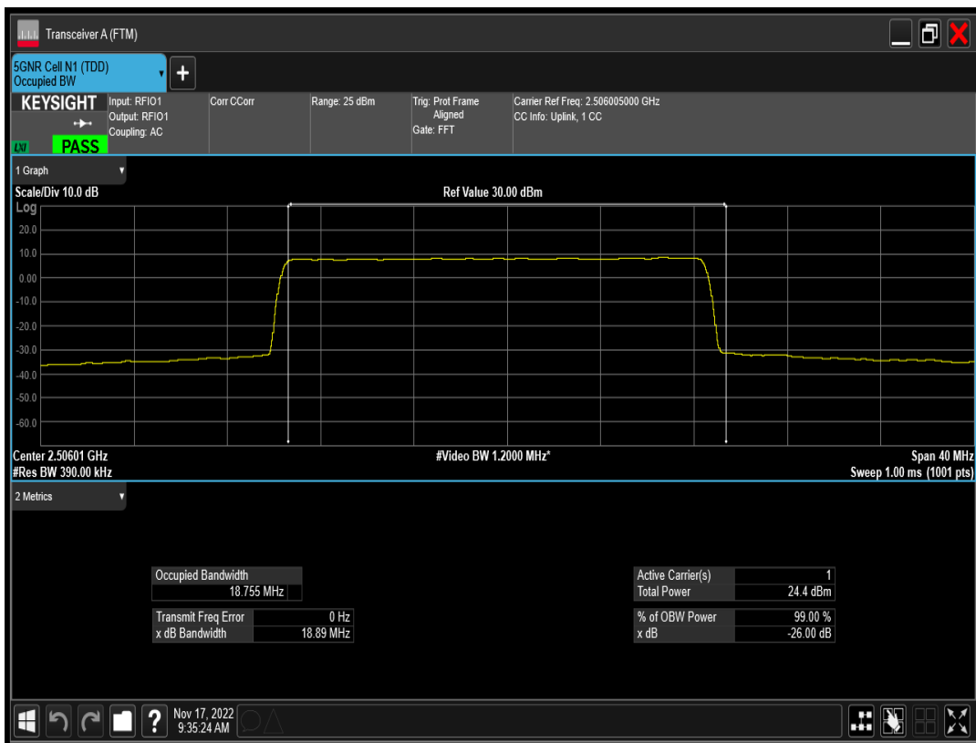
n41 SCS=15kHz DFT_QAM64 BW=20MHz Channel=501201 RB=100@0
