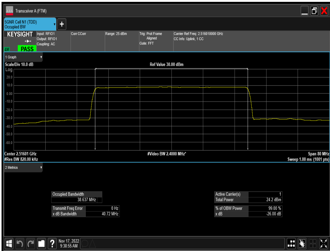
n41 SCS=15kHz DFT_QAM64 BW=40MHz Channel=503202 RB=216@0
