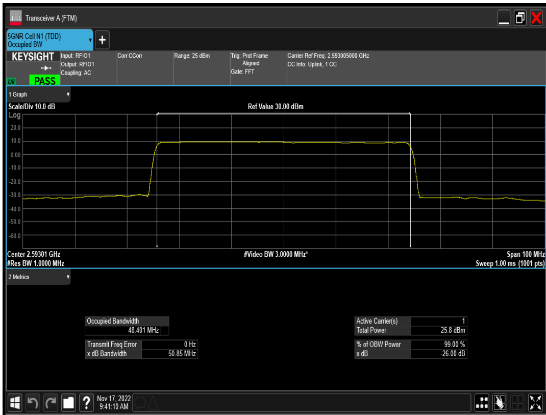
n41 SCS=15kHz DFT_QPSK BW=50MHz Channel=518601 RB=270@0
