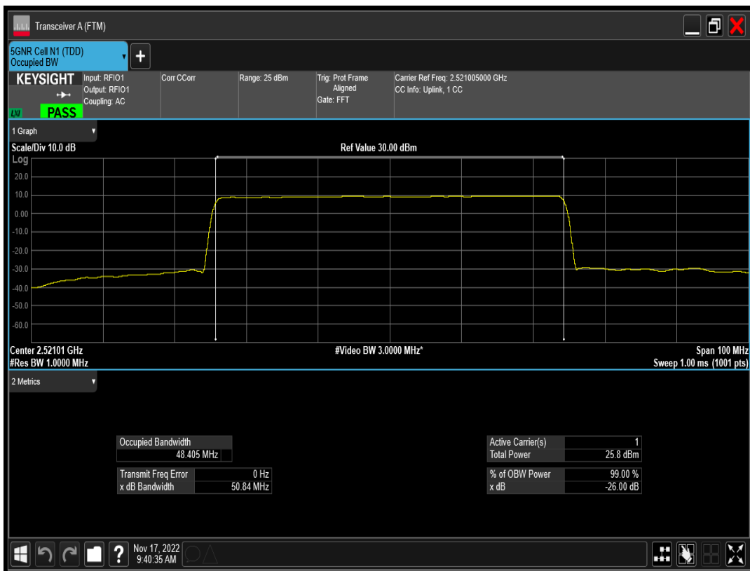
n41 SCS=15kHz DFT_QPSK BW=50MHz Channel=504201 RB=270@0
