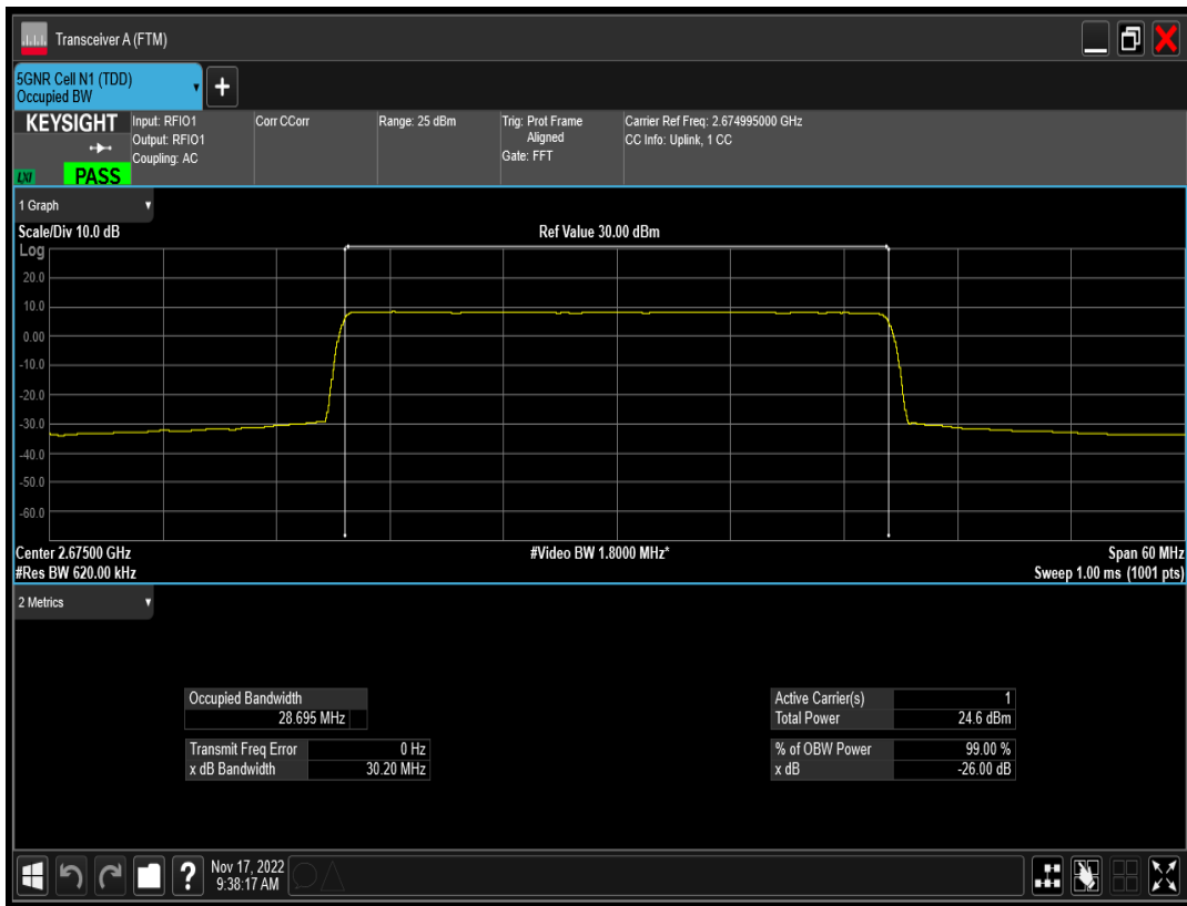
n41 SCS=15kHz DFT_QAM64 BW=30MHz Channel=534999 RB=160@0
