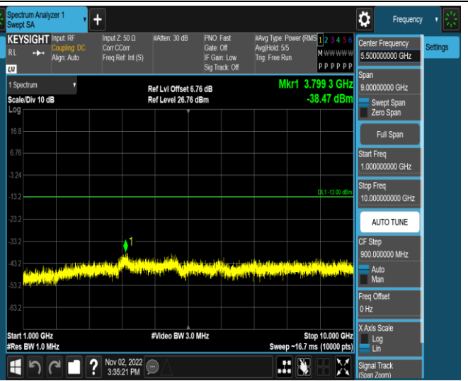
Band5-10MHz-QPSK-20600-1RB#0-Range2:1000~10000MHz
