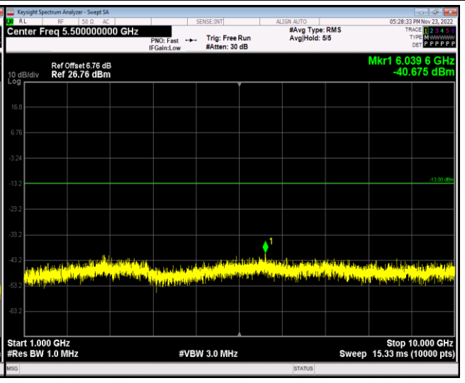
Band5-10MHz-64QAM-20525-1RB#0-Range2:1000~10000MHz
