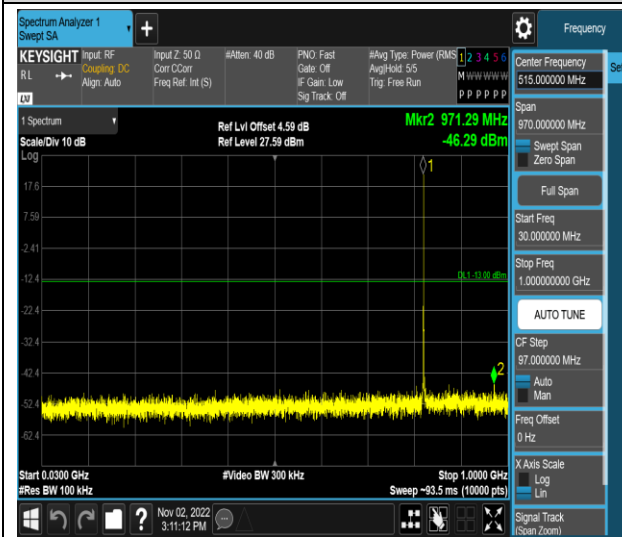
Band5-1.4MHz-QPSK-20525-1RB#0-Range1:30~1000MHz
