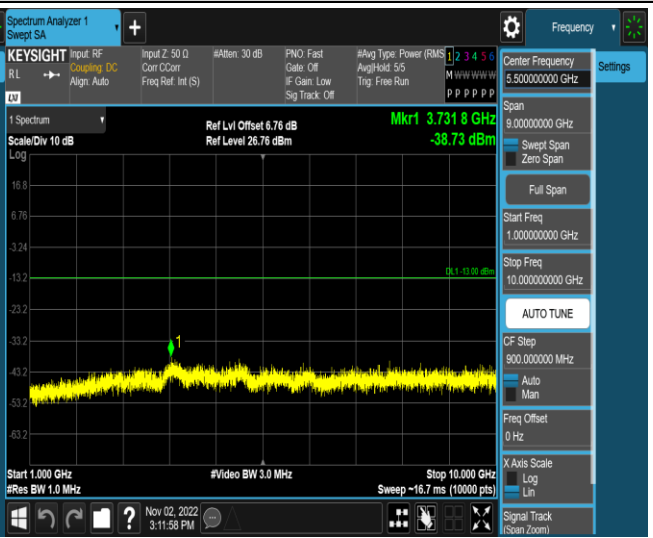
Band5-1.4MHz-QPSK-20525-1RB#0-Range2:1000~10000MHz
