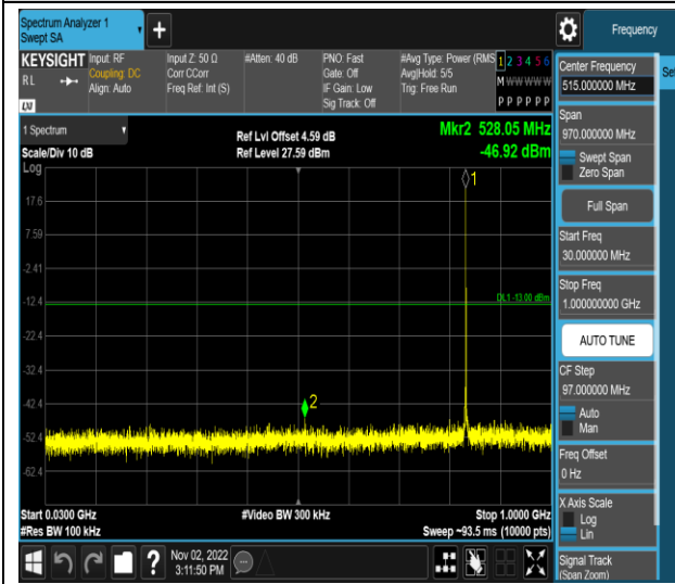
Band5-1.4MHz-QPSK-20525-1RB#0-Range1:30~1000MHz
