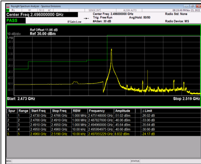
Band41-20MHz-64QAM-39750-100RB#0
