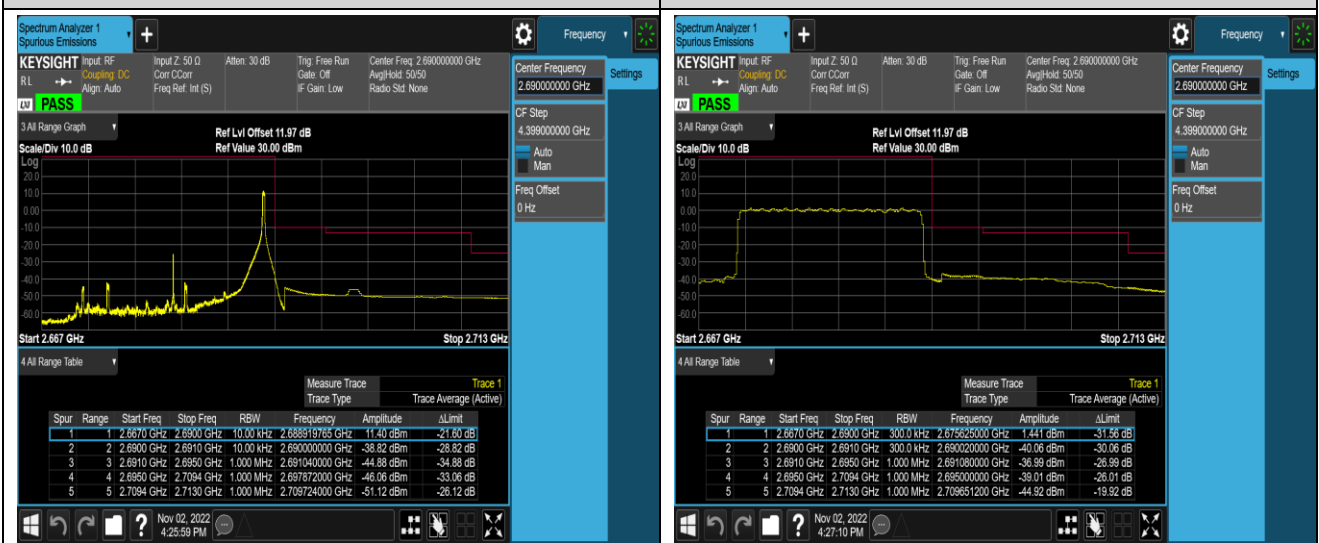
Band41-20MHz-64QAM-39750-1RB#0
