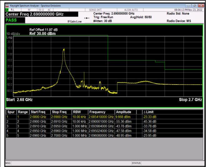
Band41-5MHz-64QAM-41565-25RB#0
