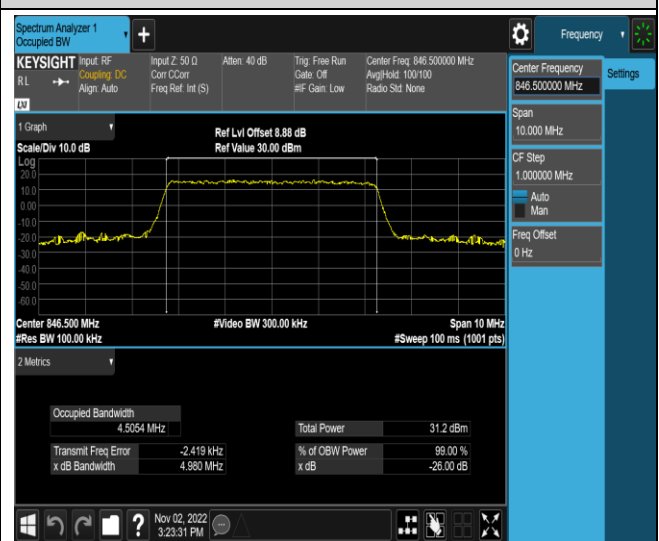
Band5-5MHz-64QAM-20525-25RB#0
