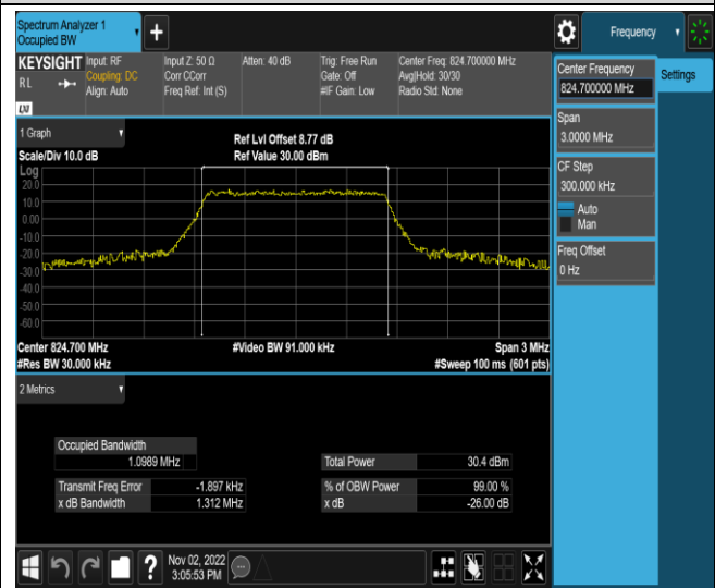
Band5-1.4MHz-16QAM-20643-6RB#0
