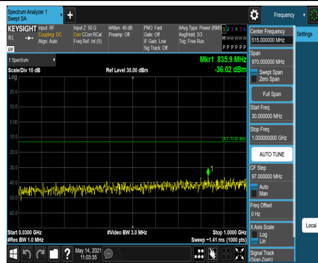
Band2-20MHz-16QAM-19100-1RB#0-Range1:30~1
