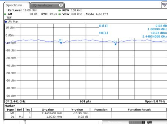
8-DPSK
