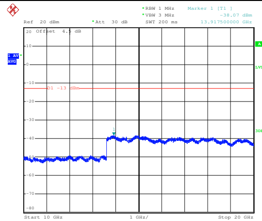
QPSK Middle channel-10GHz~20GHz
