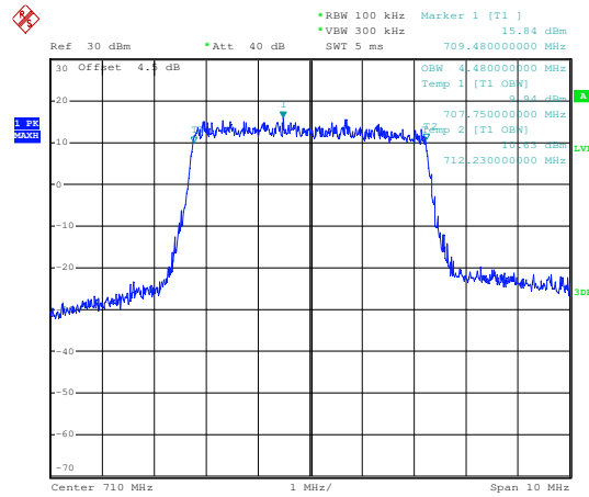
16QAM High channel
