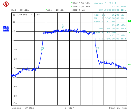
16QAM Middle channel
