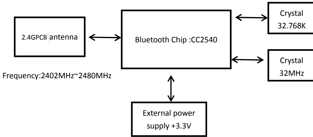
ZX_BLE_A3block diagram:
