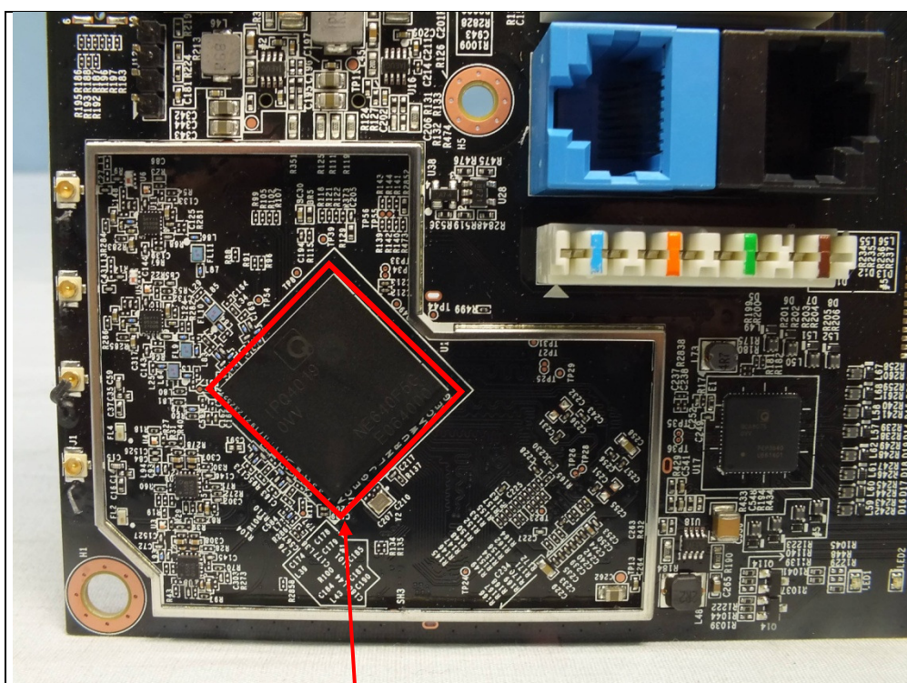
Chip (For WLAN)
