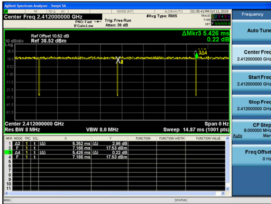
802.11n(HT20)_MCS0
