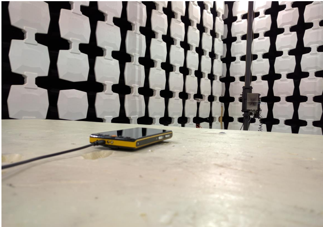
Radiated Spurious Measurement (Above 1GHz) Setup
