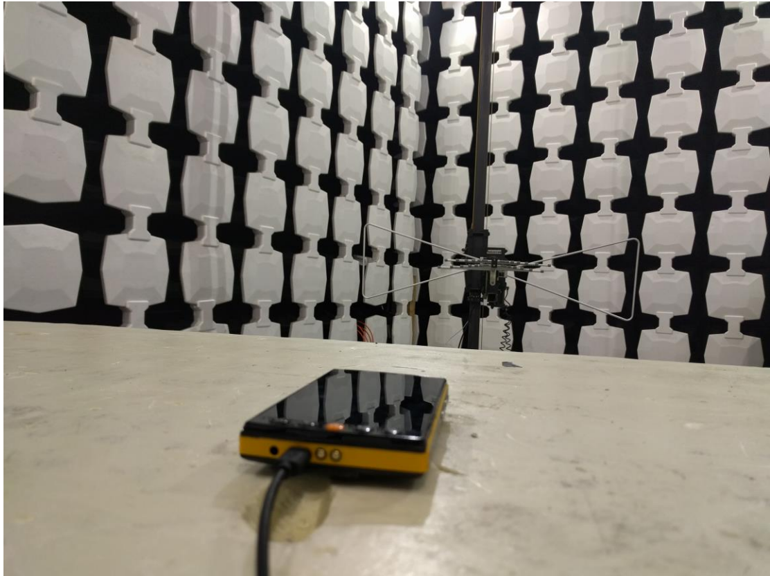
Radiated Spurious Measurement(30MHz to 1GHz) Setup
