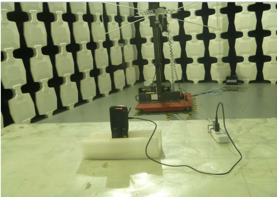
Radiated Spurious Measurement(30MHz to 1GHz) Setup
