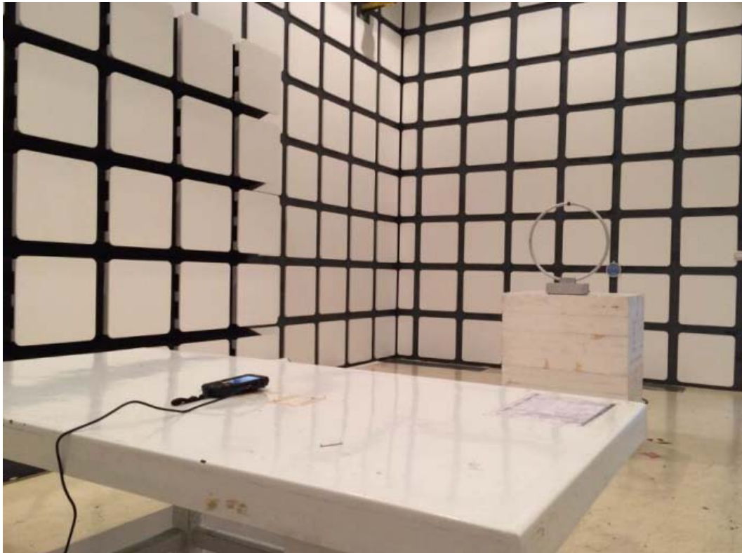
Radiated Spurious Measurement(Blow 30MHz) Setup
