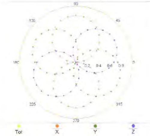
f=600 MHz,TEM
