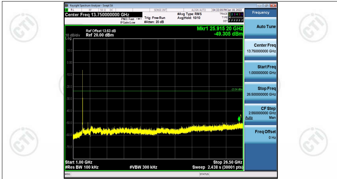
11G_Ant1_2437_1000~26500
