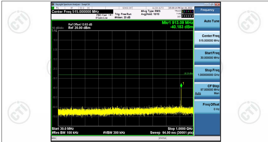
11N20SISO_Ant1_2437_30~1000
