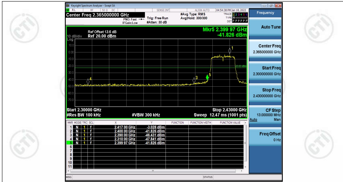
11N20SISO_Ant1_Low_2412
