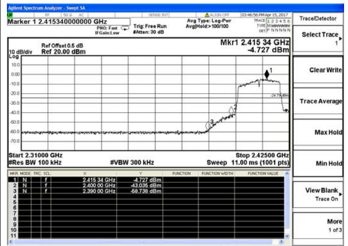
Channel 1 / 2412 MHz
