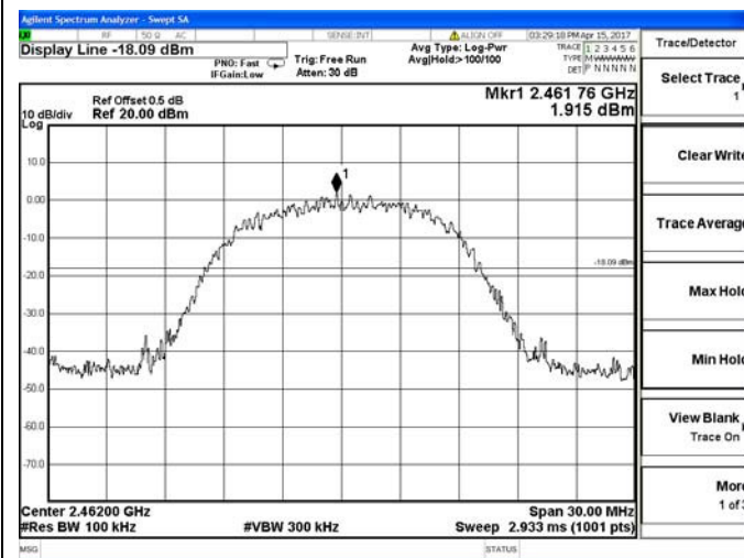
Channel 11 / 2462 MHz
