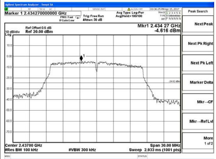
Channel 6 / 2437 MHz
