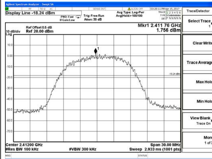
Channel 1 / 2412 MHz
