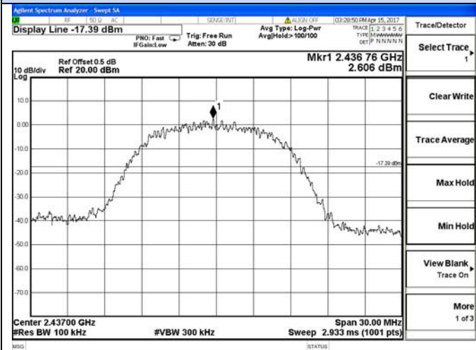
2422 – 2452 MHz
