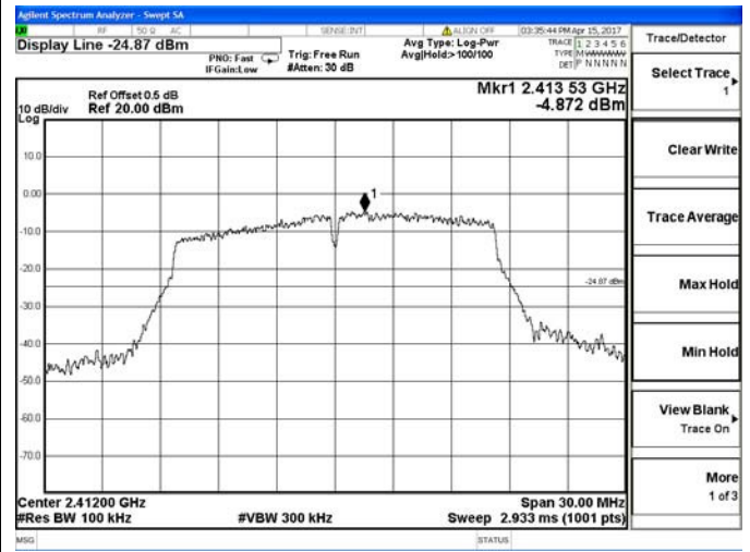
Channel 1 / 2412 MHz
