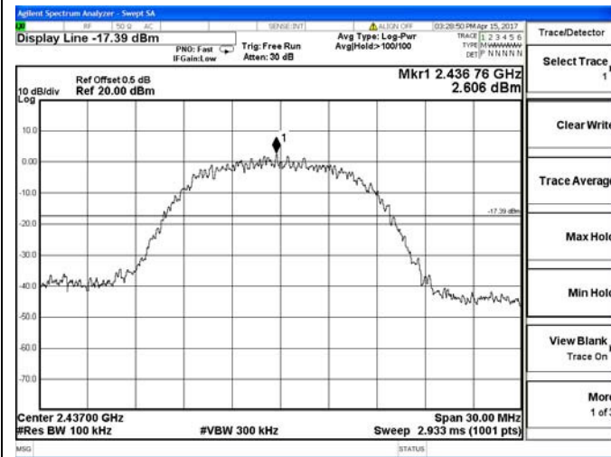
Channel 6 / 2437 MHz
