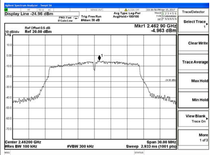
Channel 11 / 2462 MHz
