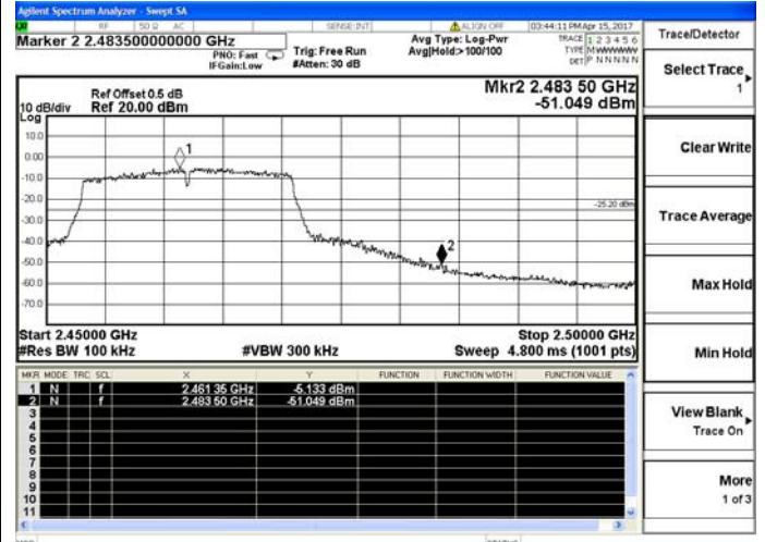
Channel 11 / 2462 MHz
