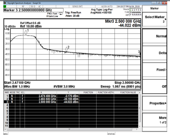
2474 MHz – Peak
