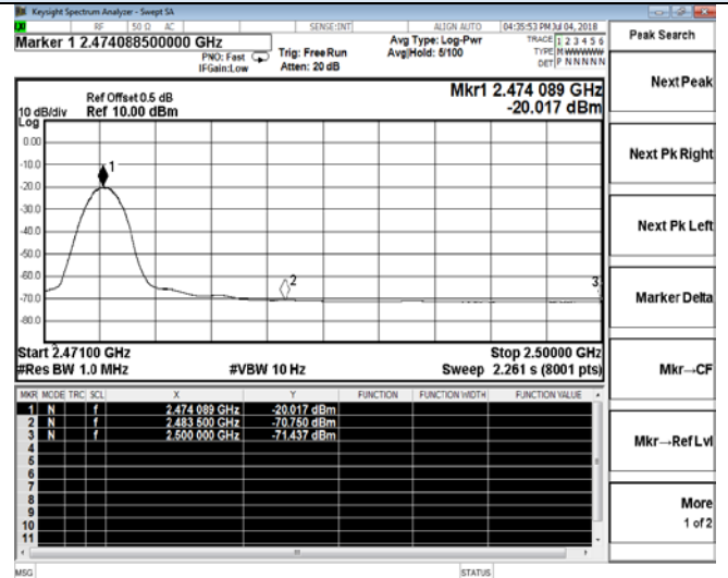
2474 MHz – Average
