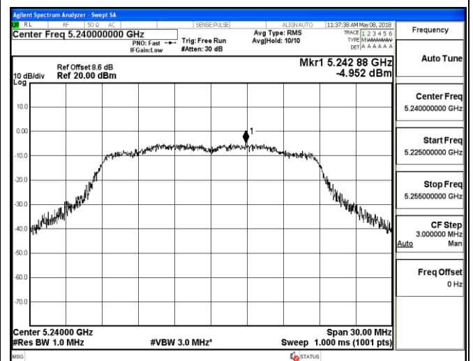
Channel 48 / 5240 MHz
