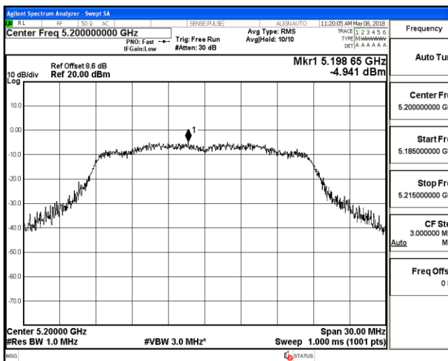
Channel 40 / 5200 MHz
