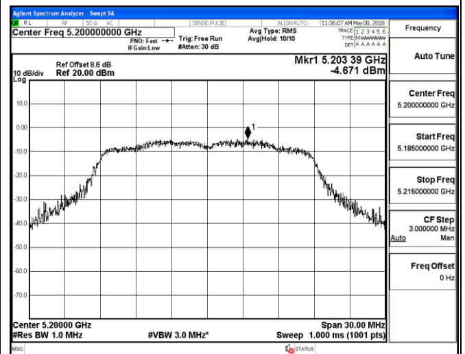
Channel 40 / 5200 MHz
