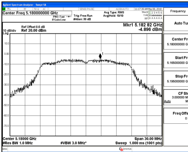
Channel 36 / 5180 MHz
