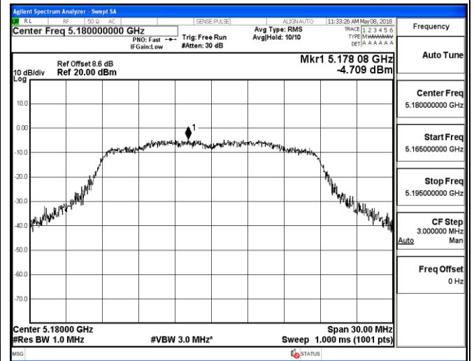
Channel 36 / 5180 MHz
