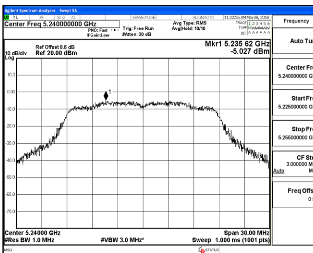
Channel 48 / 5240 MHz
