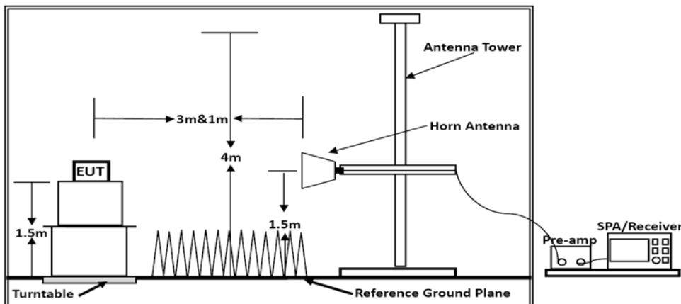
Above 1GHz
