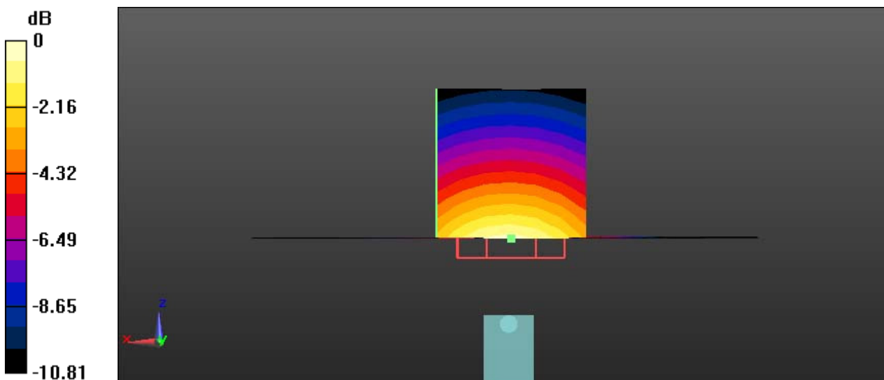
0 dB = 10.4 W/kg = 10.17 dBW/kg
