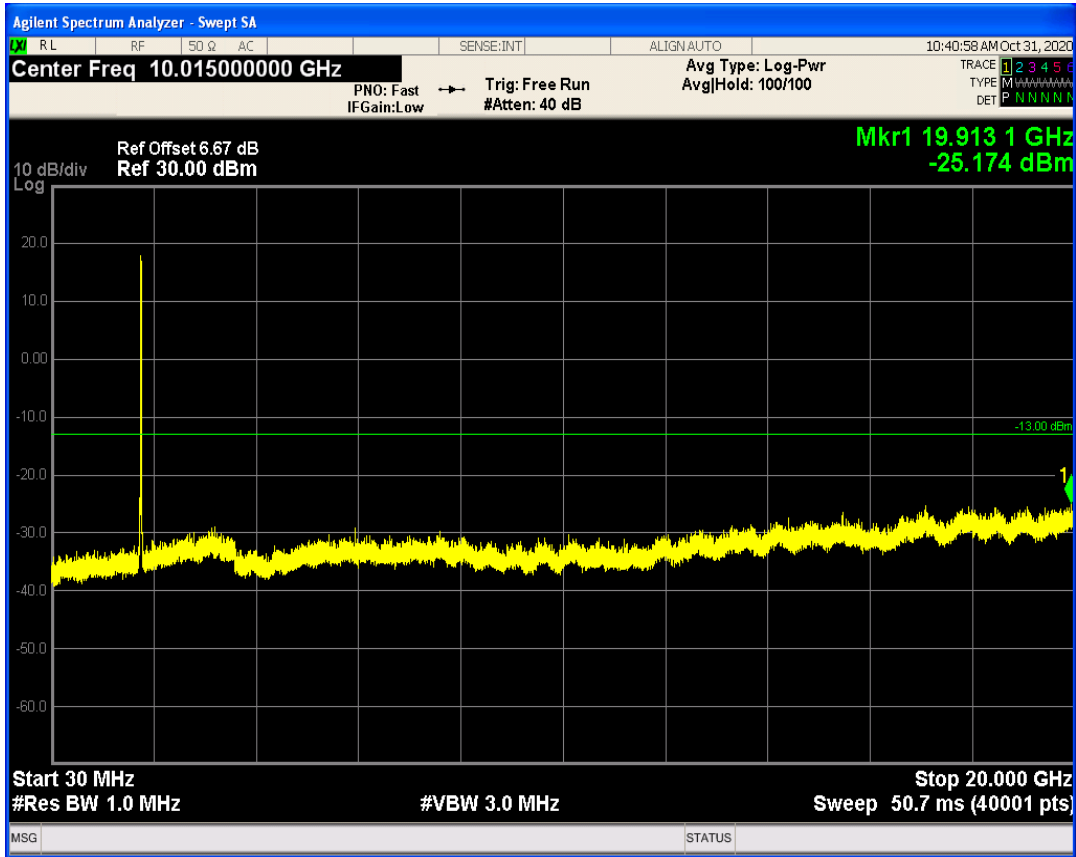
LTE Band41 QPSK BW=5MHz Channel=39675 RB Size=1 Position=#0
