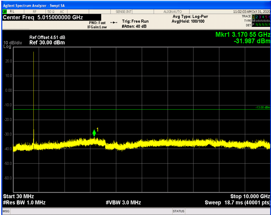
LTE Band26 QAM16 BW=5MHz Channel=26815 RB Size=1 Position=#0
