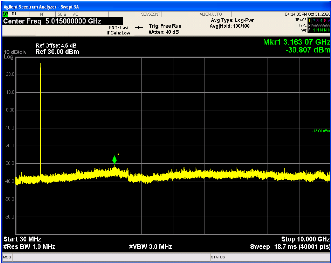
LTE Band26 QAM16 BW=3MHz Channel=26775 RB Size=15 Position=#0
