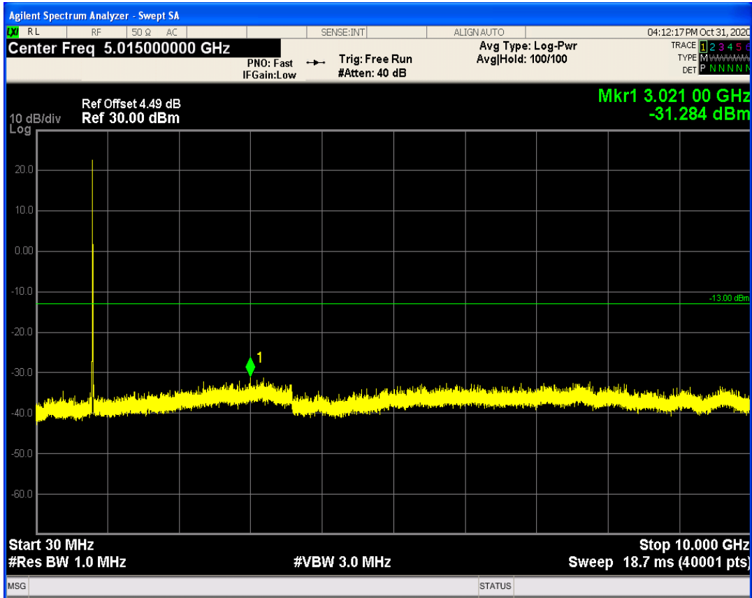
LTE Band26 QPSK BW=5MHz Channel=26715 RB Size=25 Position=#0
