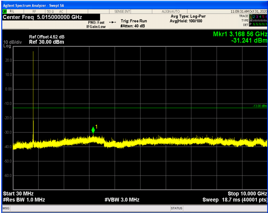
LTE Band26 QPSK BW=15MHz Channel=26965 RB Size=1 Position=#0
