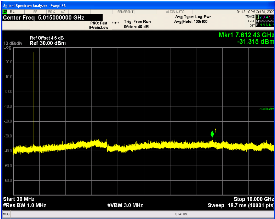
LTE Band26 QPSK BW=3MHz Channel=26775 RB Size=15 Position=#0
