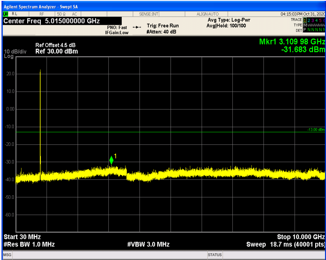
LTE Band26 QAM16 BW=5MHz Channel=26765 RB Size=25 Position=#0
