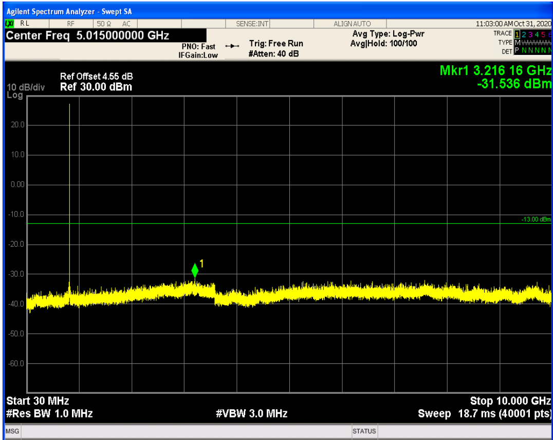
LTE Band26 QPSK BW=5MHz Channel=27015 RB Size=1 Position=#0
