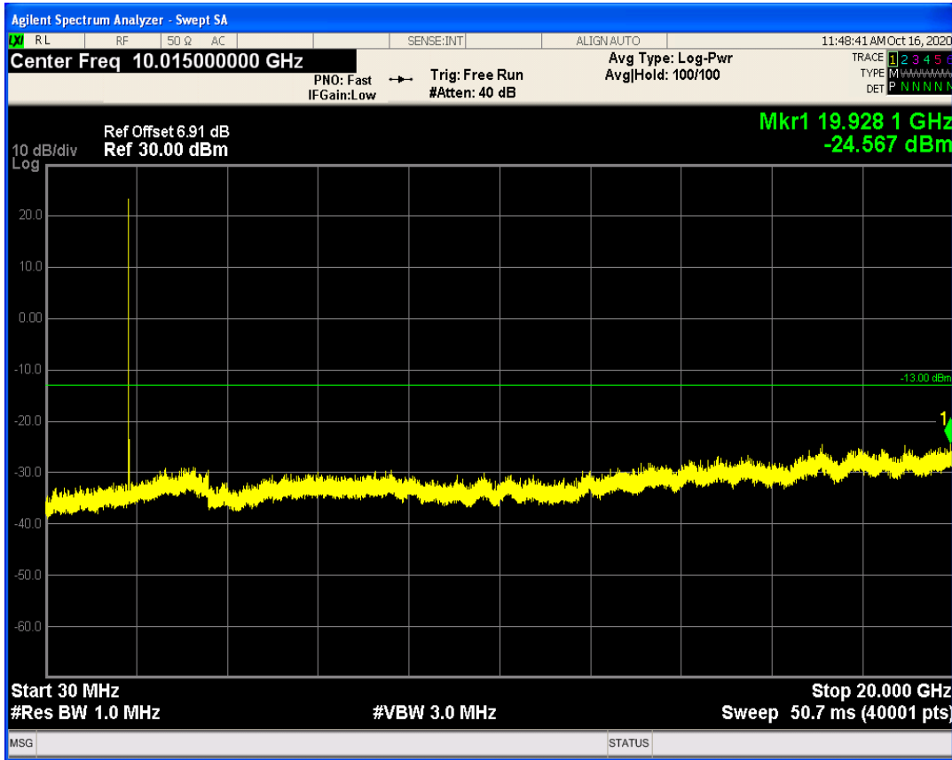
LTE Band25 QAM16 BW=3MHz Channel=26055 RB Size=1 Position=#0
