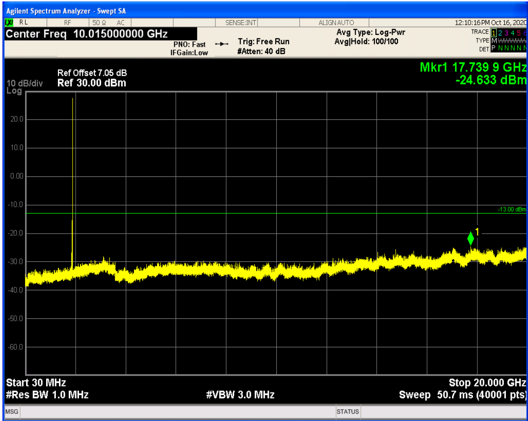
LTE Band25 QAM16 BW=15MHz Channel=26615 RB Size=1 Position=#0
