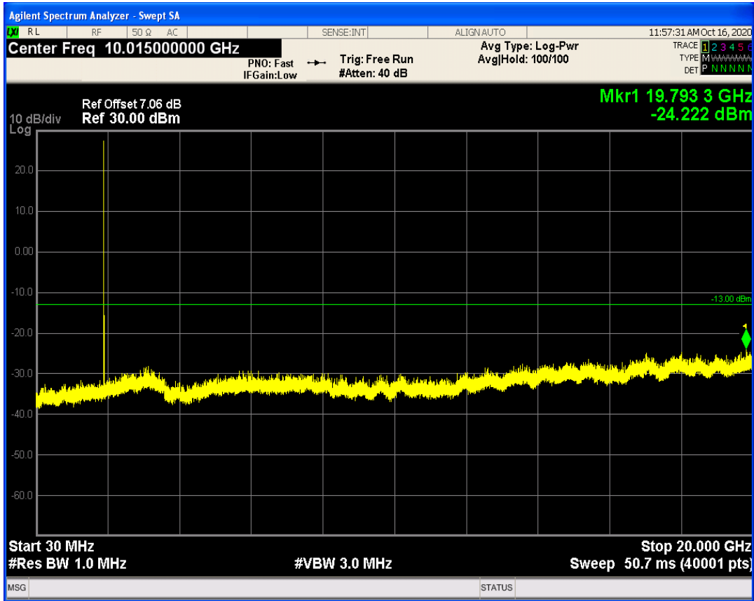
LTE Band25 QAM16 BW=5MHz Channel=26665 RB Size=1 Position=#0
