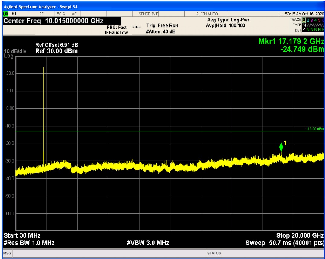
LTE Band25 QPSK BW=3MHz Channel=26675 RB Size=1 Position=#0
