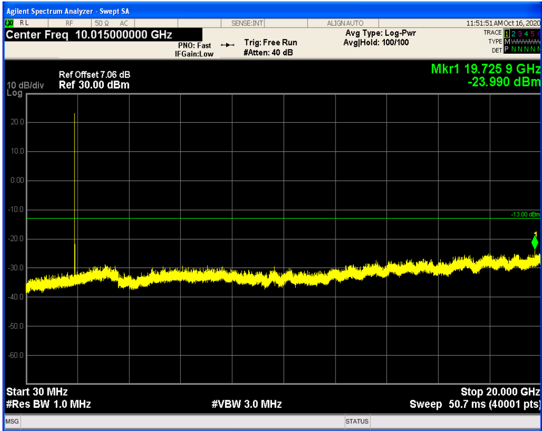
LTE Band25 QAM16 BW=3MHz Channel=26675 RB Size=1 Position=#0
