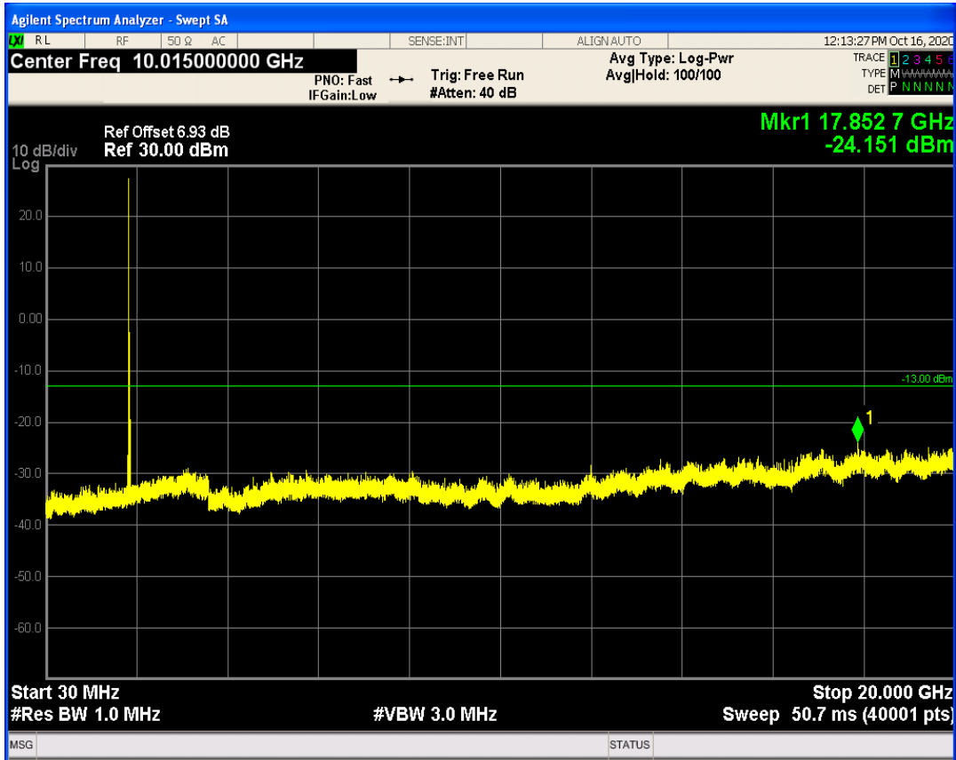
LTE Band25 QPSK BW=20MHz Channel=26140 RB Size=1 Position=#0
