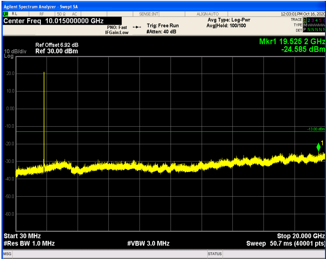
LTE Band25 QAM16 BW=10MHz Channel=26090 RB Size=50 Position=#0
