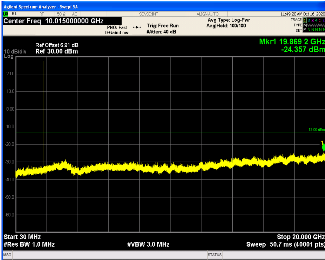
LTE Band25 QAM16 BW=3MHz Channel=26055 RB Size=1 Position=#0
