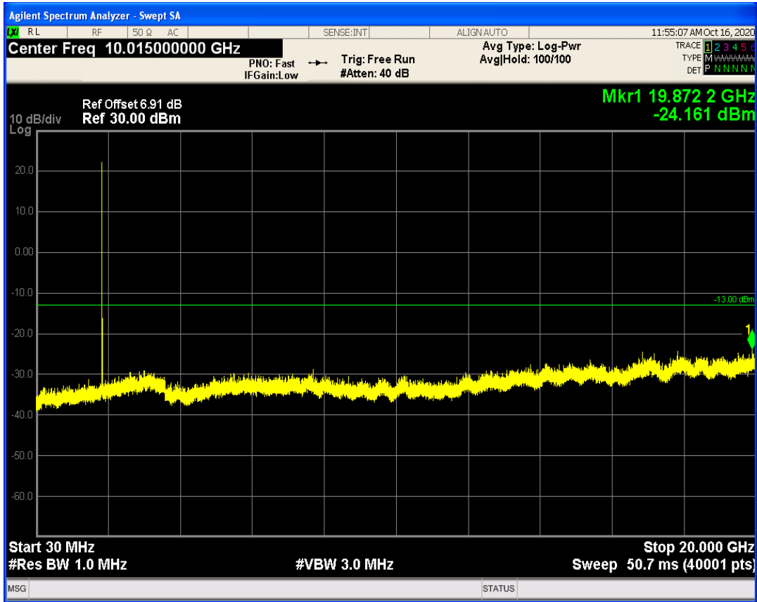
LTE Band25 QAM16 BW=5MHz Channel=26065 RB Size=1 Position=#0
