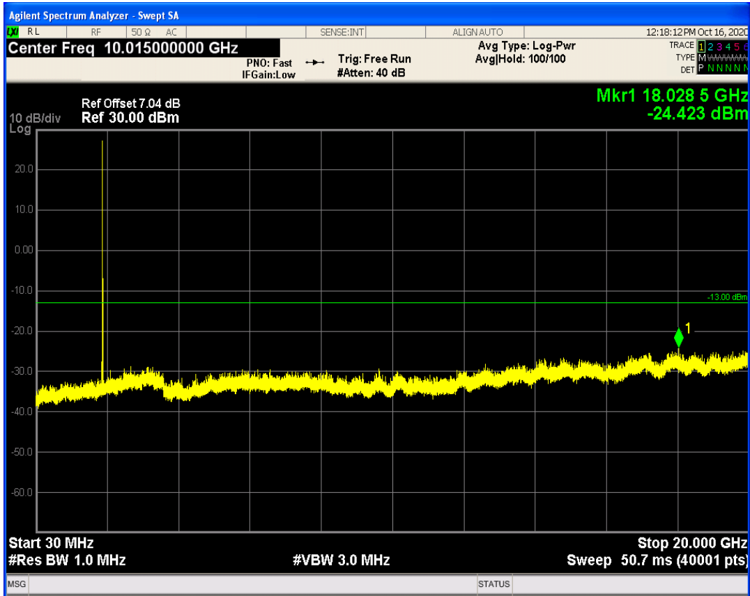
LTE Band25 QAM16 BW=20MHz Channel=26590 RB Size=1 Position=#0
