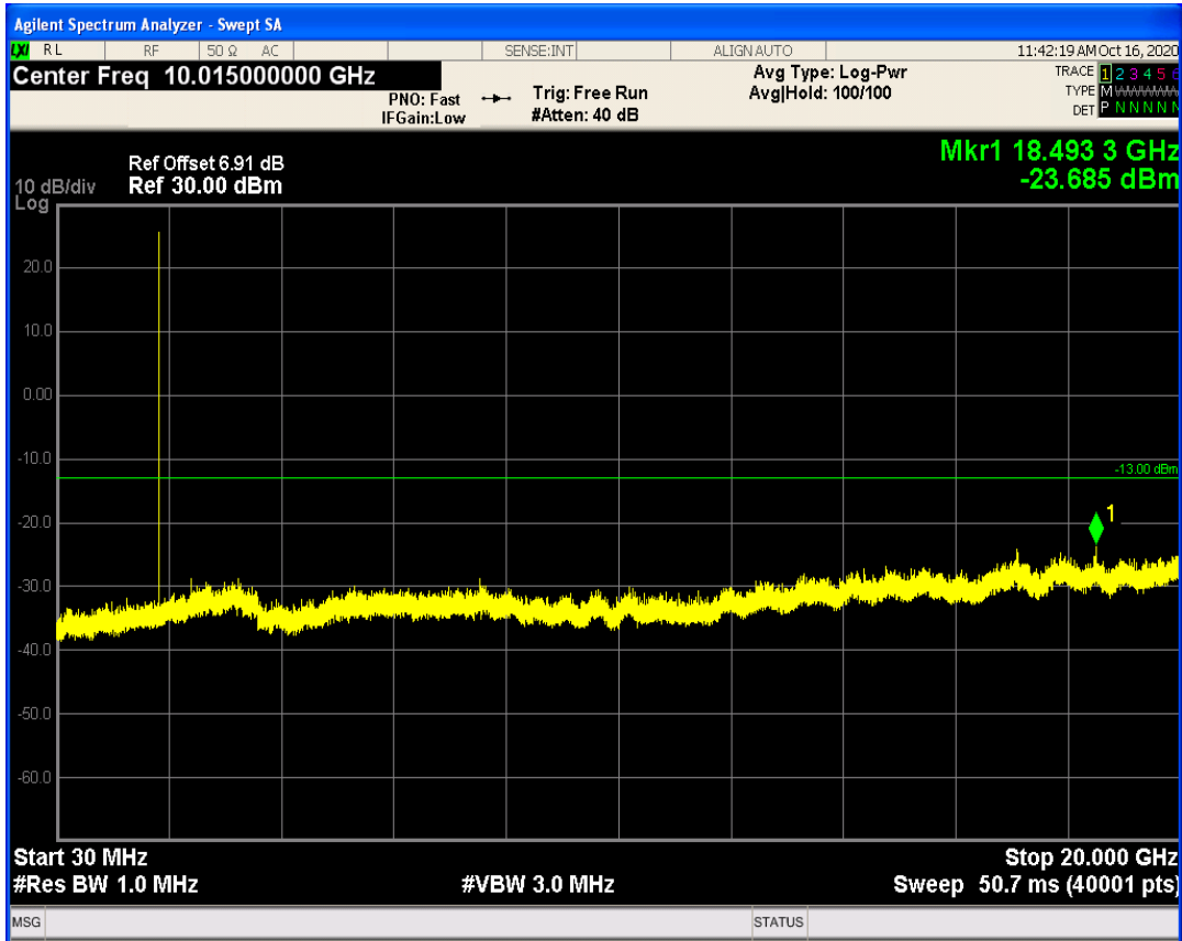
LTE Band25 QPSK BW=1.4MHz Channel=26047 RB Size=6 Position=#0
