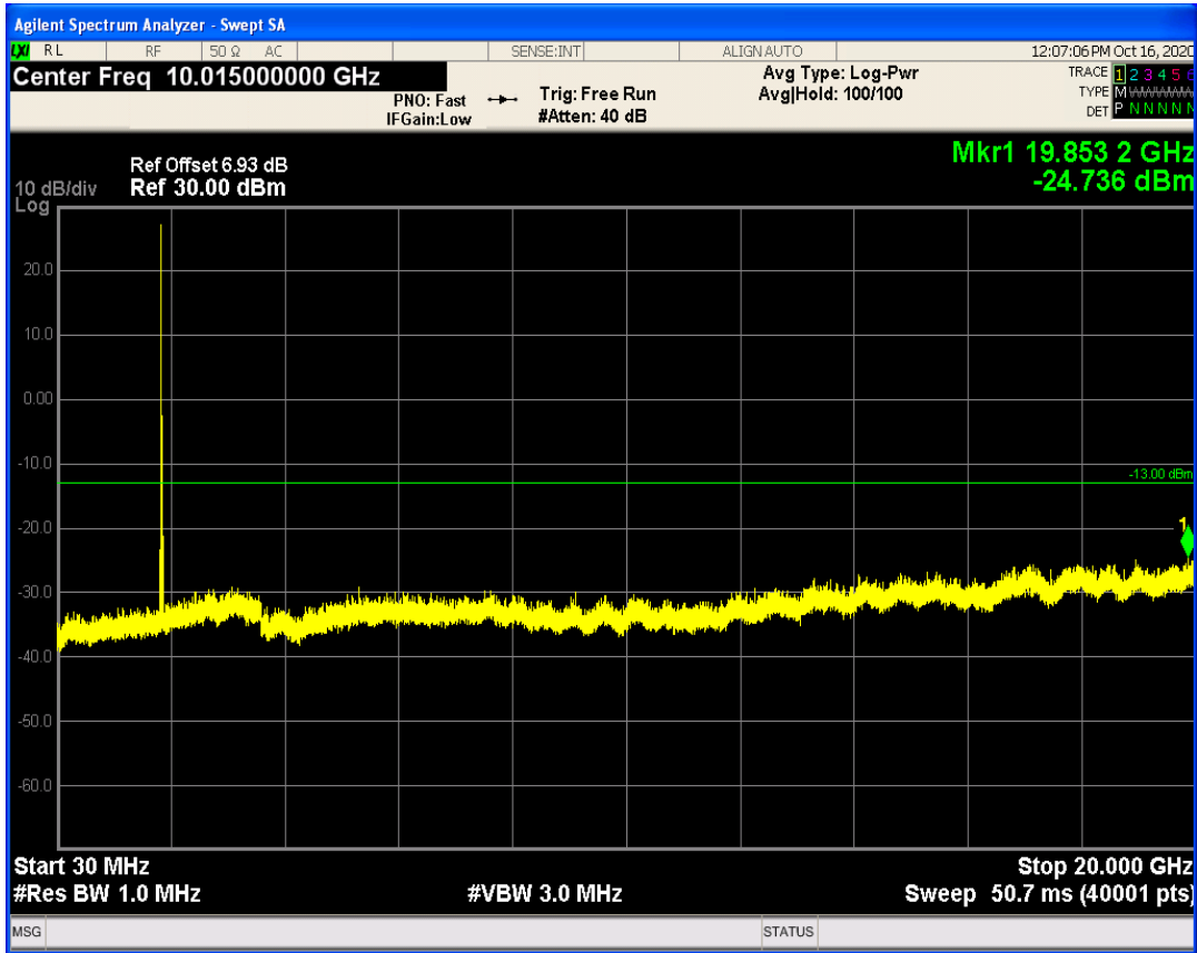
LTE Band25 QAM16 BW=10MHz Channel=26640 RB Size=50 Position=#0
