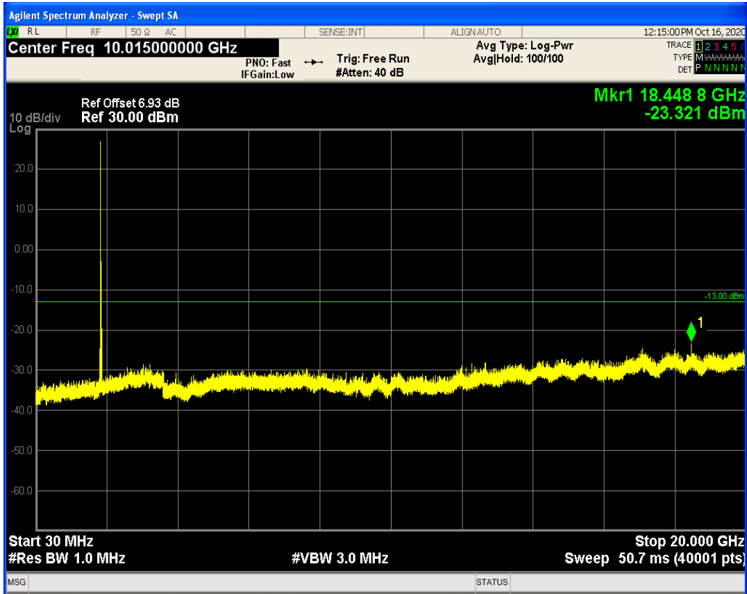
LTE Band25 QAM16 BW=20MHz Channel=26140 RB Size=1 Position=#0
