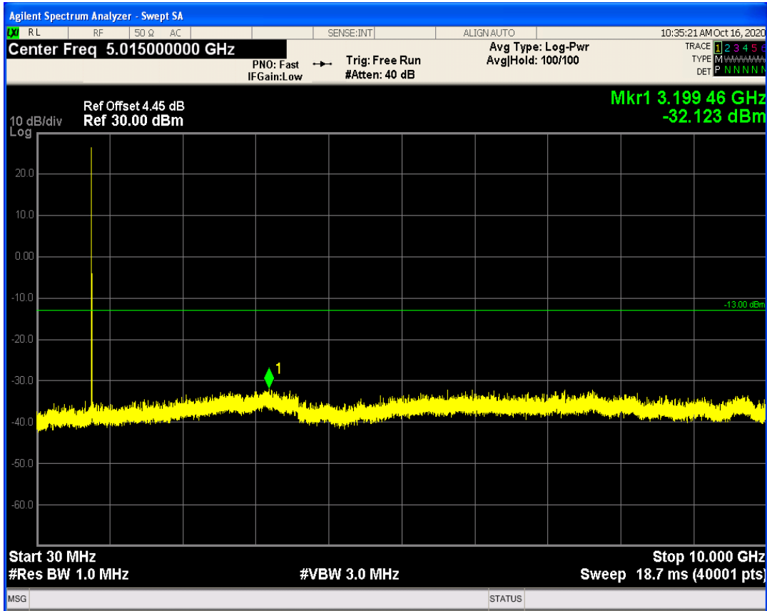
LTE Band13 QAM16 BW=10MHz Channel=23230 RB Size=1 Position=#0
