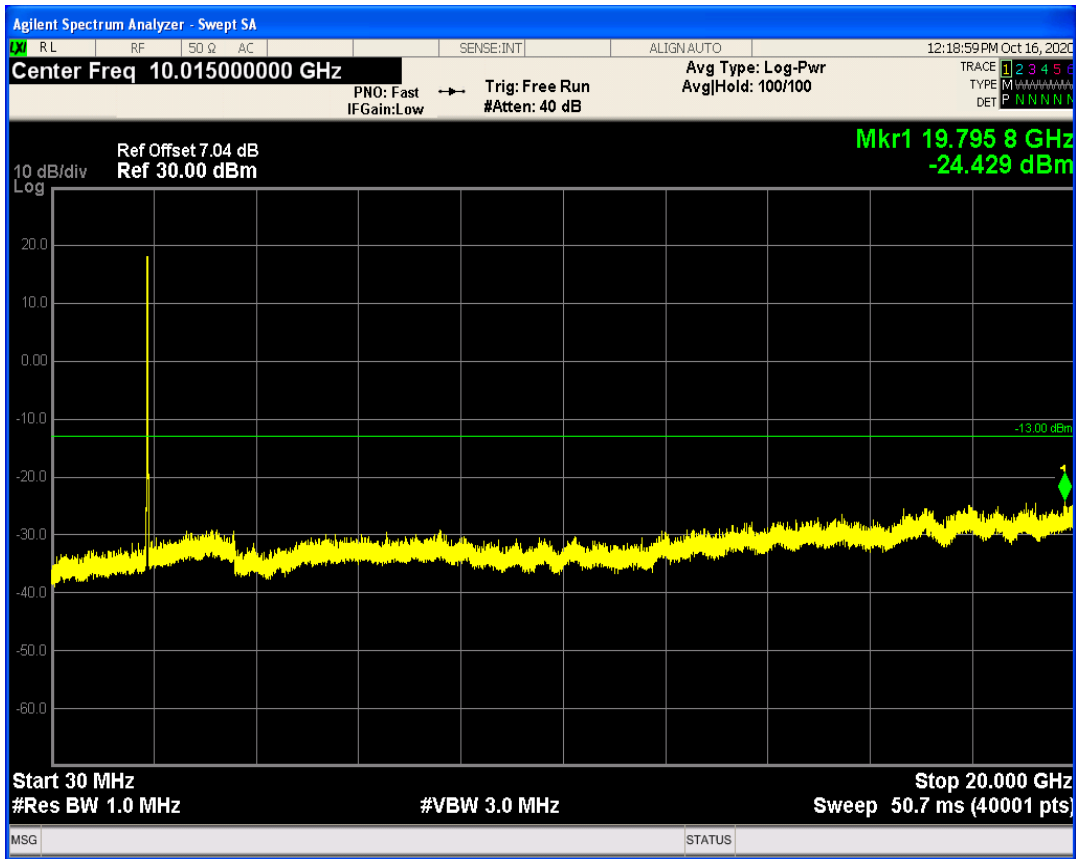
LTE Band26 QPSK BW=1.4MHz Channel=26797 RB Size=6 Position=#0
