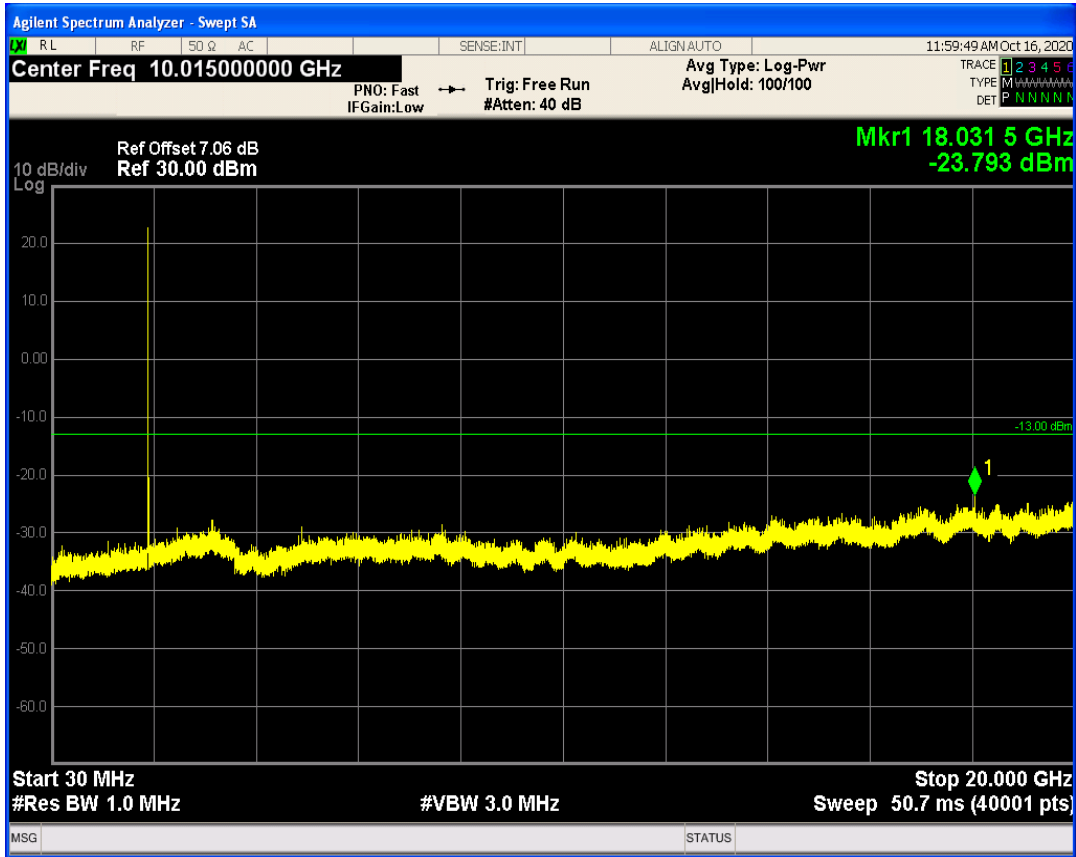
LTE Band25 QPSK BW=10MHz Channel=26090 RB Size=1 Position=#0
