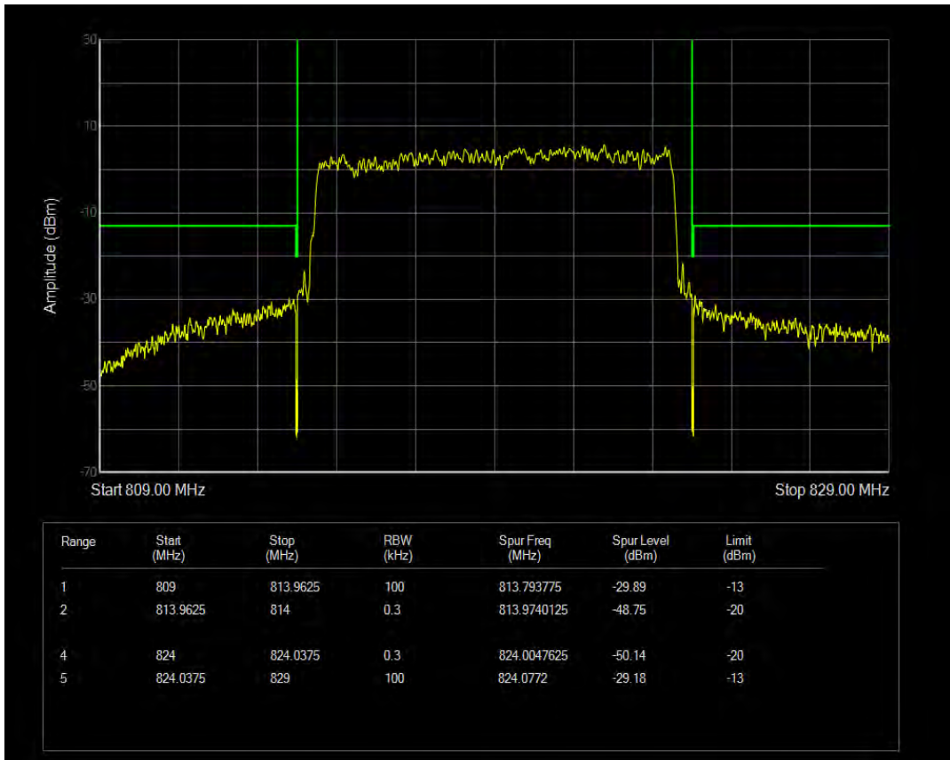
LTE Band26 QPSK BW=10MHz Channel=26740 RB Size=50 Position=#0
