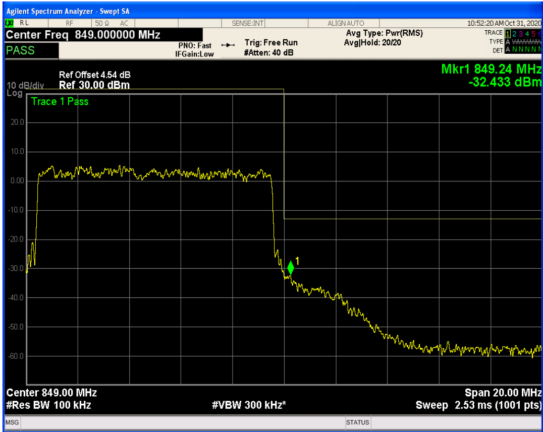
LTE Band26 QAM16 BW=10MHz Channel=26990 RB Size=1 Position=#0
