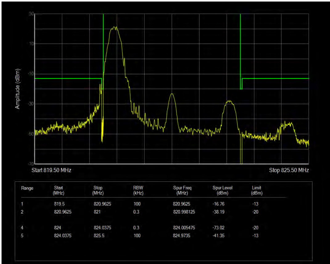
LTE Band26 QPSK BW=3MHz Channel=26775 RB Size=1 Position=#0
