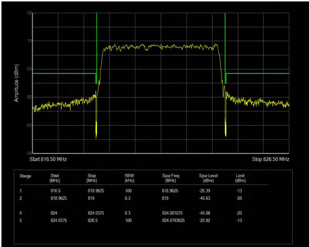
LTE Band26 QPSK BW=5MHz Channel=26765 RB Size=25 Position=#0
