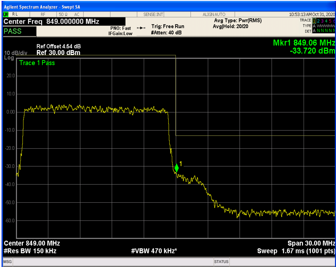
LTE Band26 QAM16 BW=15MHz Channel=26965 RB Size=75 Position=#0
