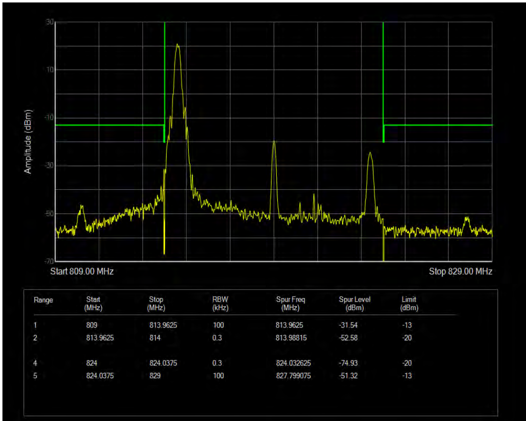
LTE Band26 QPSK BW=10MHz Channel=26740 RB Size=1 Position=#0
