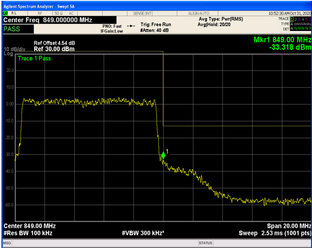
LTE Band26 QAM16 BW=10MHz Channel=26990 RB Size=50 Position=#0
