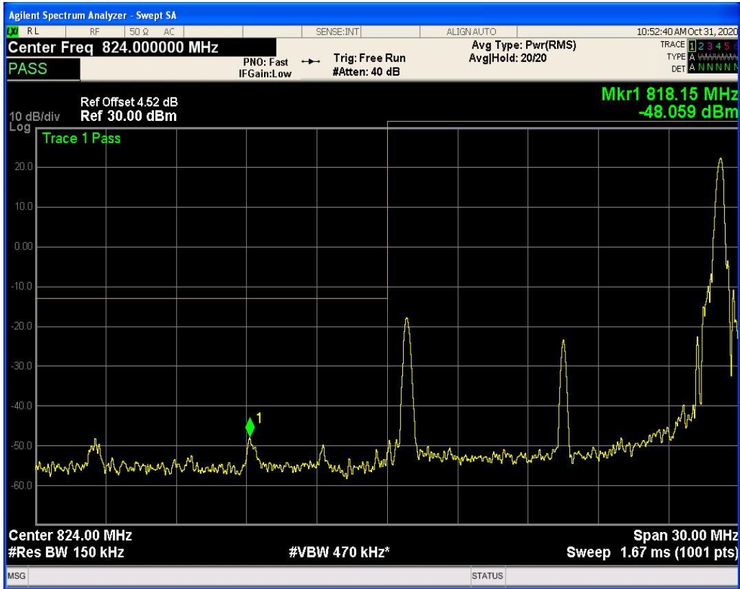
LTE Band26 QPSK BW=15MHz Channel=26865 RB Size=1 Position=#0
