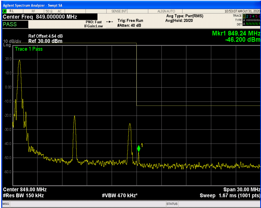
LTE Band26 QAM16 BW=15MHz Channel=26965 RB Size=1 Position=#0
