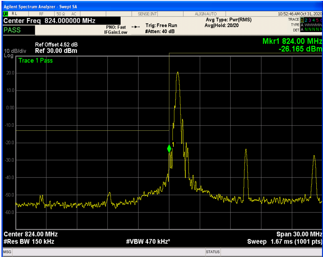
LTE Band26 QAM16 BW=15MHz Channel=26865 RB Size=1 Position=#0
