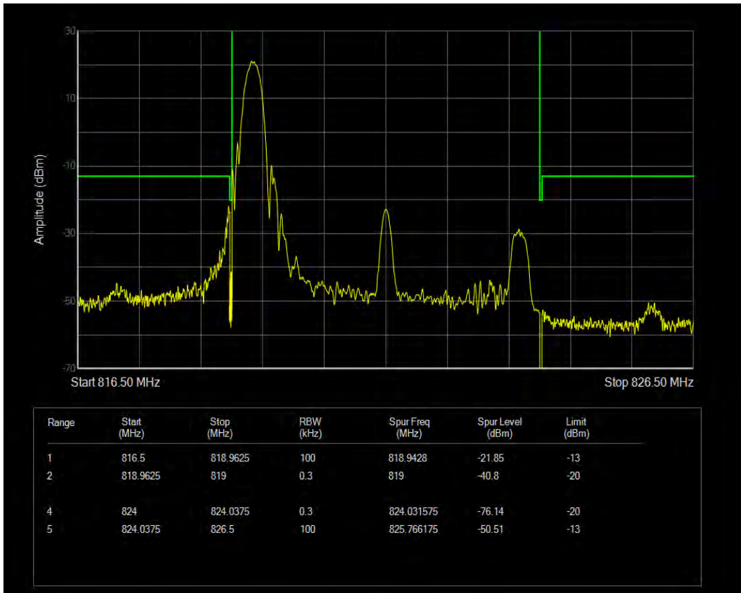
LTE Band26 QPSK BW=5MHz Channel=26765 RB Size=1 Position=#0
