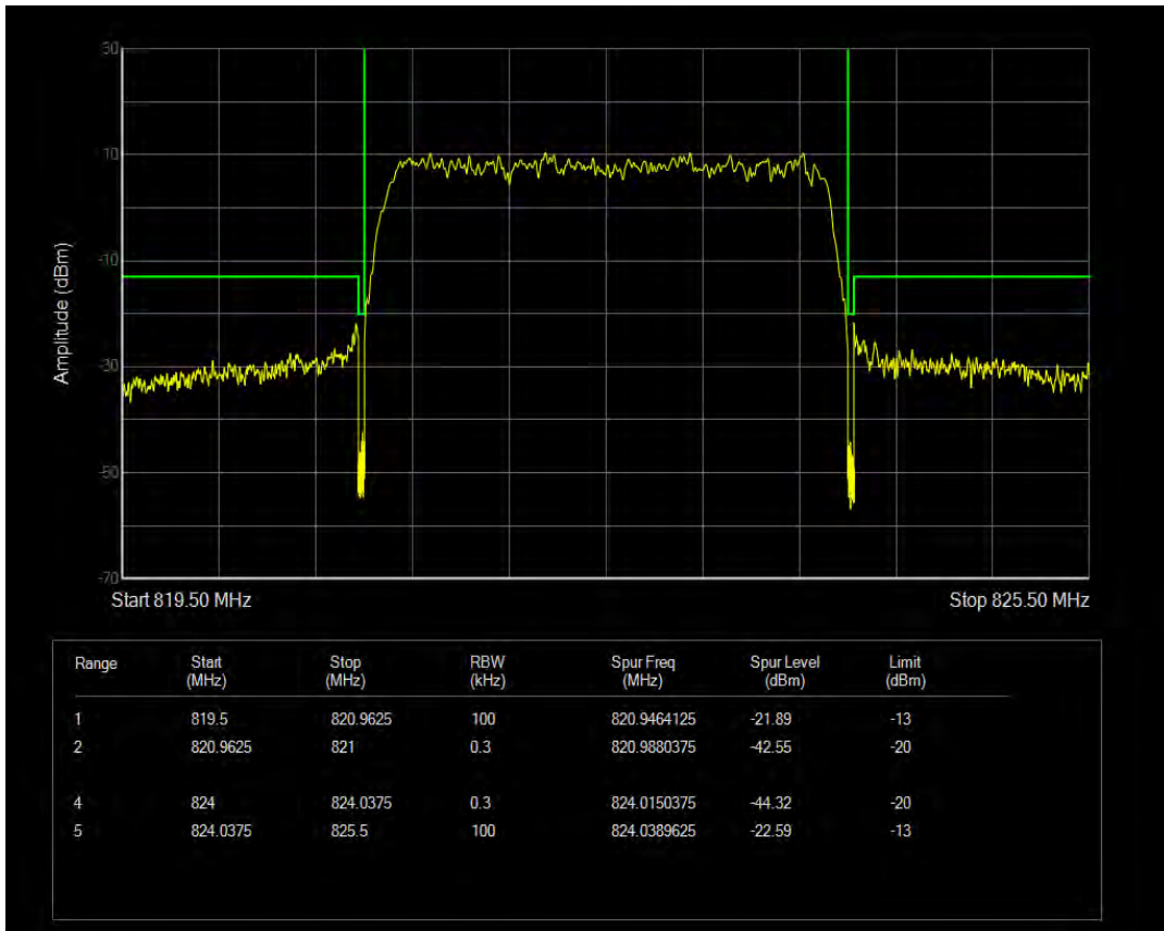
LTE Band26 QPSK BW=3MHz Channel=26775 RB Size=15 Position=#0
