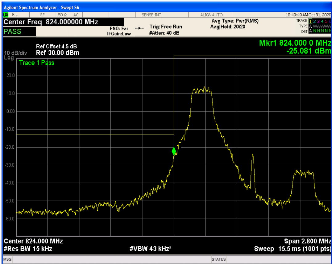
LTE Band26 QAM16 BW=1.4MHz Channel=26797 RB Size=1 Position=#0
