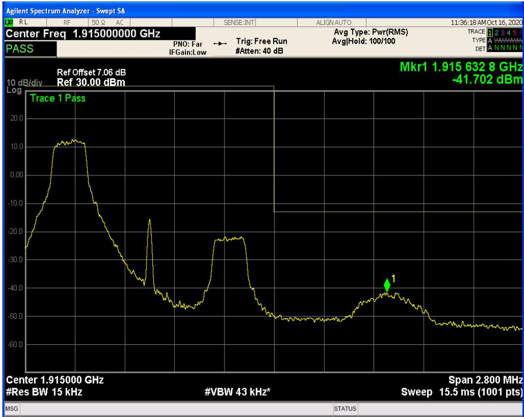
LTE Band25 QAM16 BW=1.4MHz Channel=26683 RB Size=1 Position=#0
