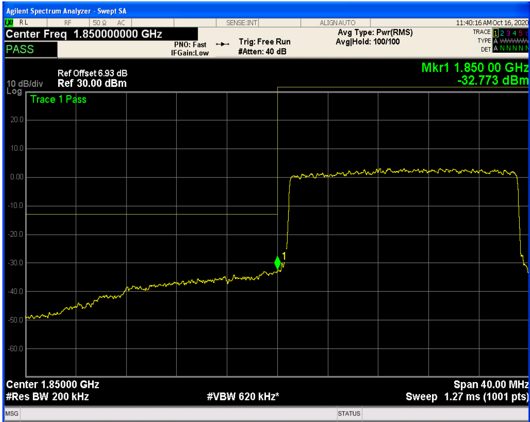
LTE Band25 QAM16 BW=20MHz Channel=26140 RB Size=100 Position=#0
