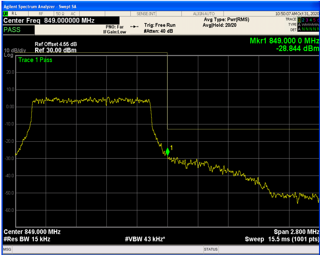
LTE Band26 QAM16 BW=1.4MHz Channel=27033 RB Size=1 Position=#0
