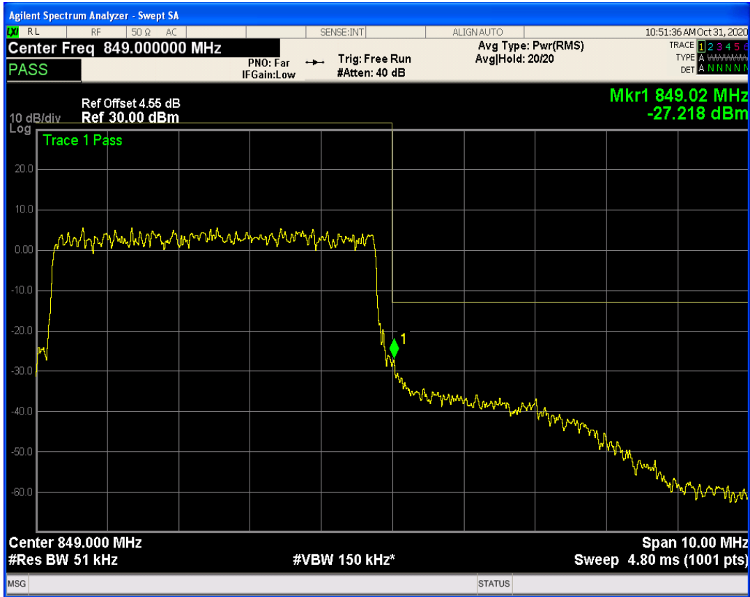
LTE Band26 QAM16 BW=5MHz Channel=27015 RB Size=1 Position=#0
