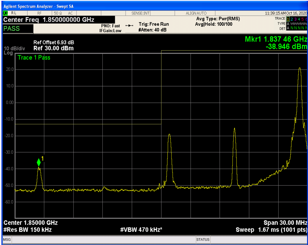
LTE Band25 QPSK BW=15MHz Channel=26115 RB Size=1 Position=#0
