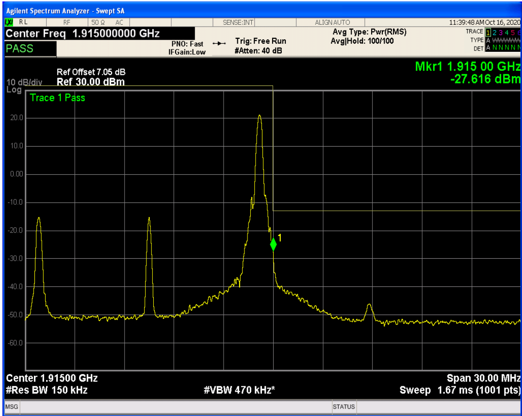
LTE Band25 QAM16 BW=15MHz Channel=26615 RB Size=75 Position=#0
