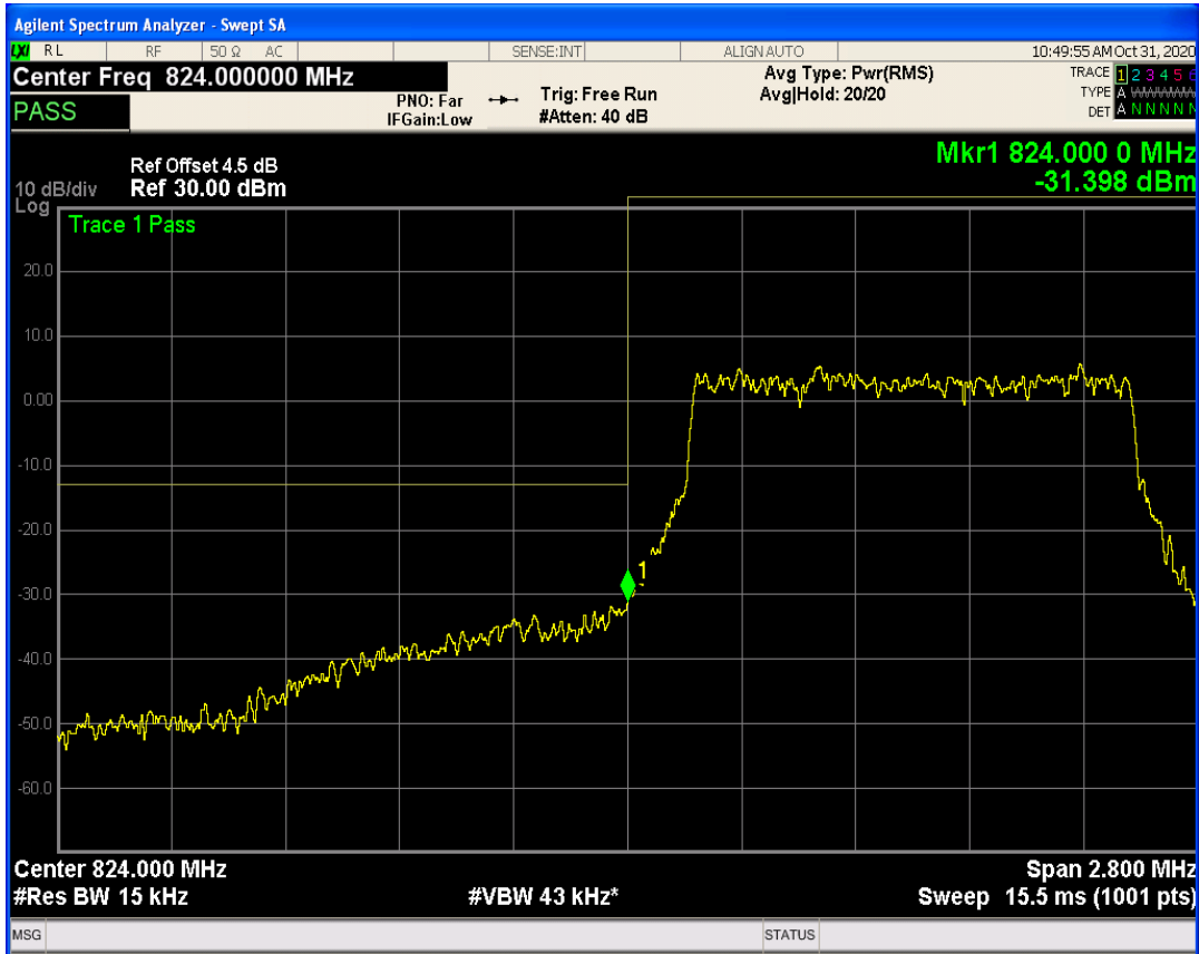
LTE Band26 QAM16 BW=1.4MHz Channel=26797 RB Size=6 Position=#0
