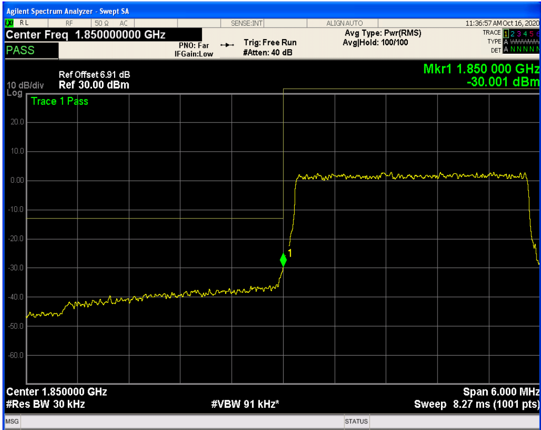
LTE Band25 QAM16 BW=3MHz Channel=26055 RB Size=15 Position=#0
