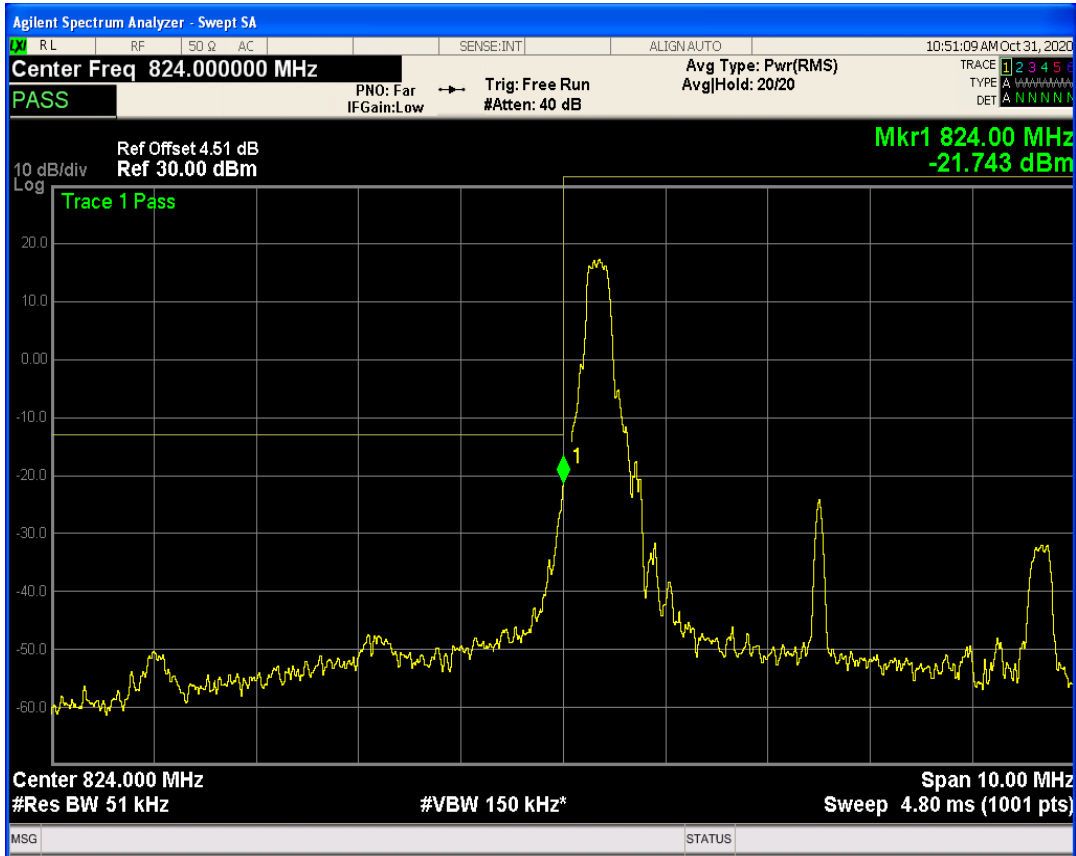
LTE Band26 QPSK BW=5MHz Channel=26815 RB Size=1 Position=#0
