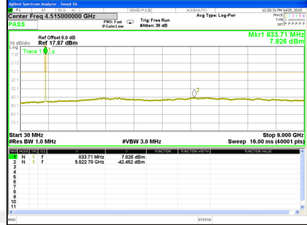
B26_Q16_10M_High_CDT_Spurious
