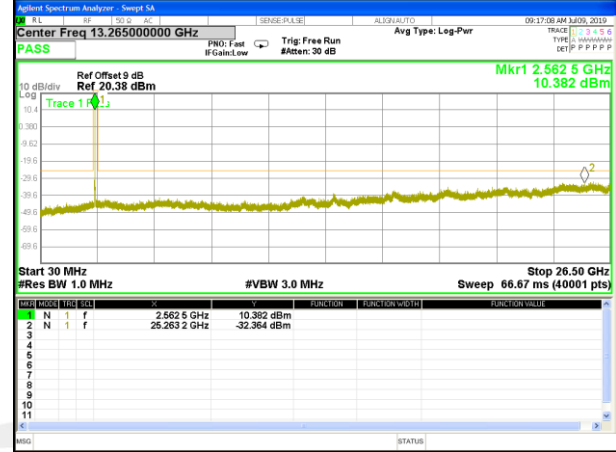
B41_Q16_15M_Mid_CDT_Spurious
