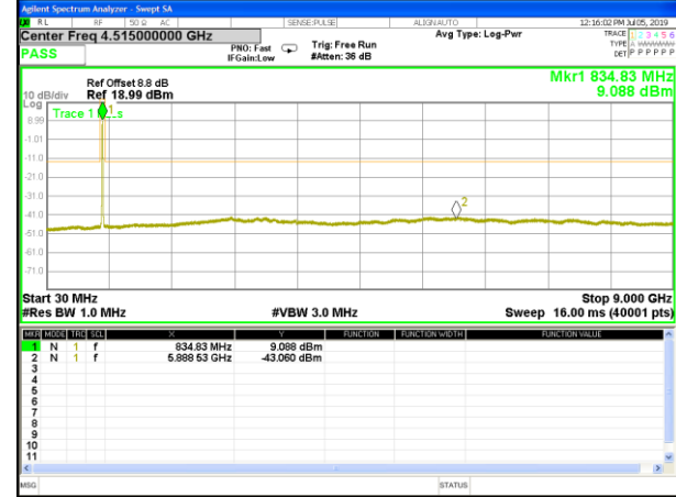
B26_QPSK_10M_High_CDT_Spurious
