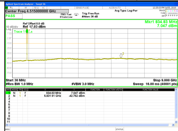
B26_QPSK_15M_Mid_CDT_Spurious
