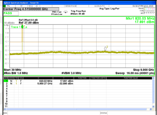
B26_Q16_5M_Mid_CDT_Spurious
