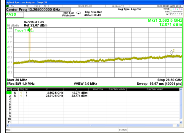
B41_QPSK_10M_Mid_CDT_Spurious
