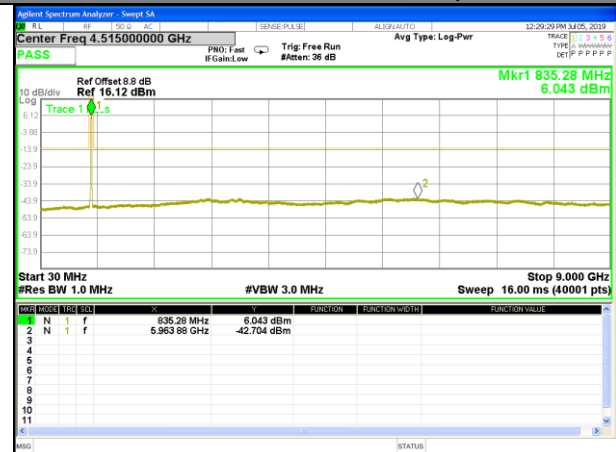
B26_Q16_15M_Mid_CDT_Spurious
