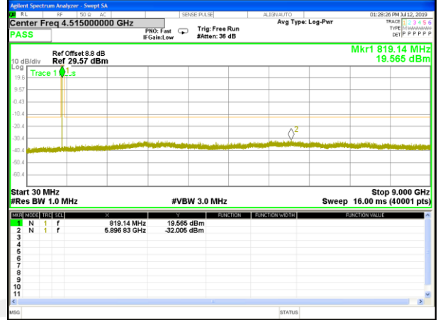
B26_Q16_3M_Mid_CDT_Spurious
