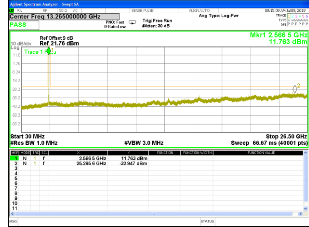
B41_QPSK_15M_Mid_CDT_Spurious
