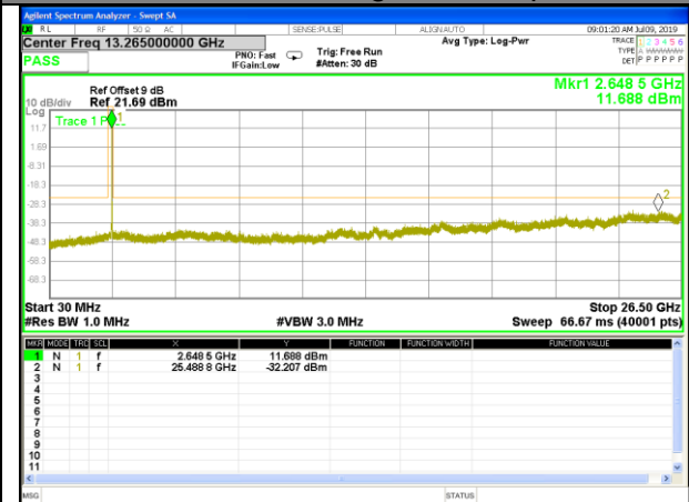
B41_QPSK_10M_High_CDT_Spurious
