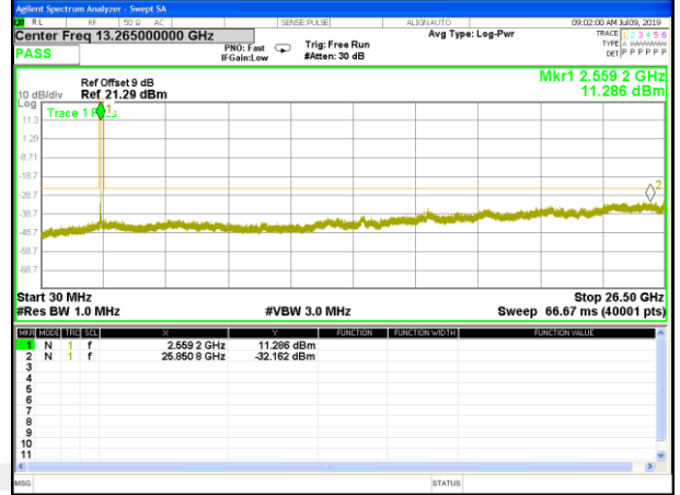
B41_Q16_10M_Mid_CDT_Spurious
