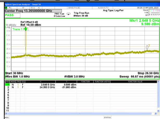
B41_QPSK_20M_High_CDT_Spurious
