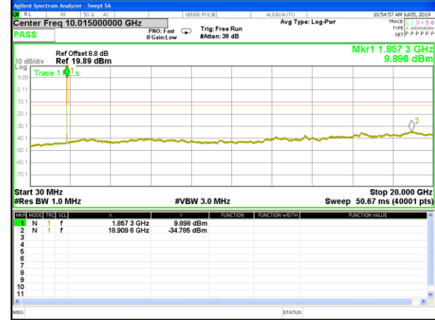
B25_QPSK_10M_Mid_CDT_Spurious
