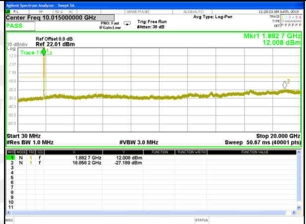
B25_Q16_20M_High_CDT_Spurious
