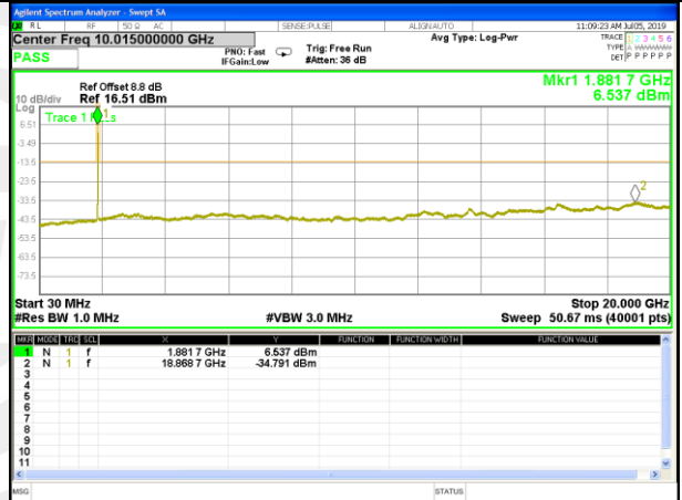
B25_Q16_15M_High_CDT_Spurious
