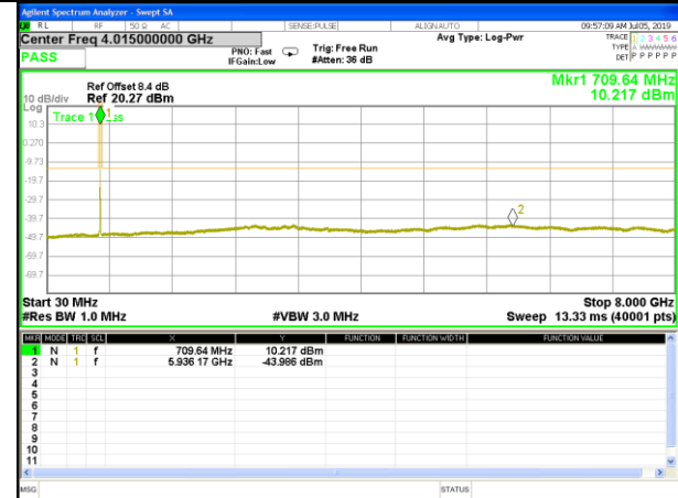
B17_QPSK_5M_High_CDT_Spurious
