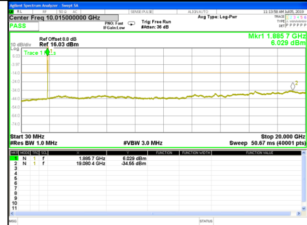
B25_QPSK_20M_High_CDT_Spurious
