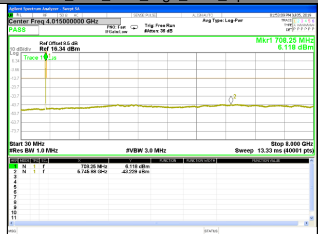
B17_Q16_10M_High_CDT_Spurious
