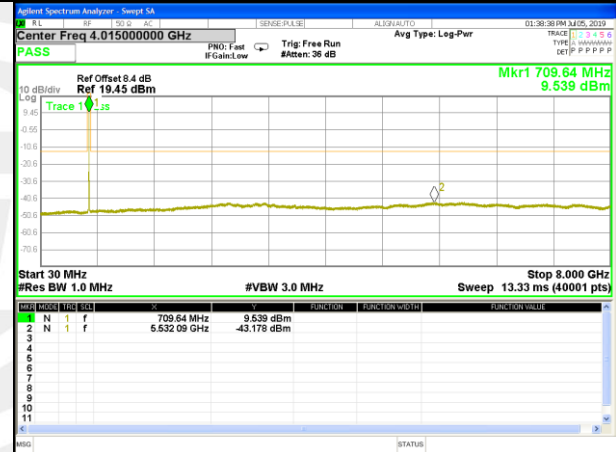
B17_Q16_5M_High_CDT_Spurious
