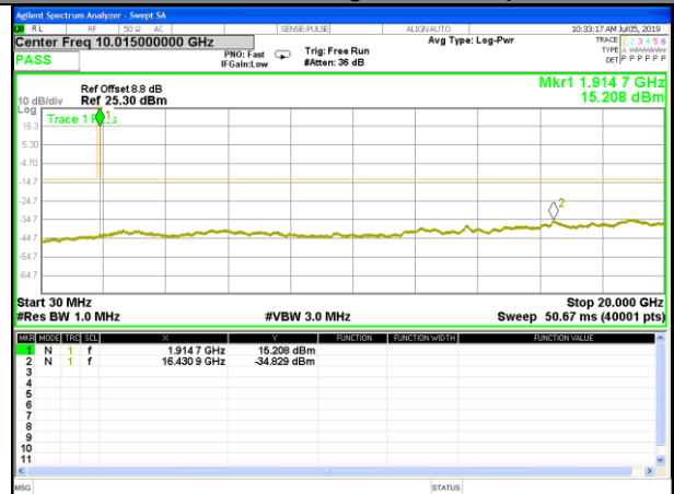
B25_Q16_1.4M_High_CDT_Spurious
