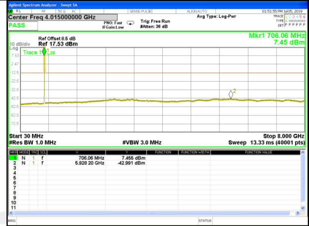
B17_Q16_10M_Mid_CDT_Spurious
