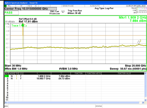
B25_QPSK_15M_High_CDT_Spurious
