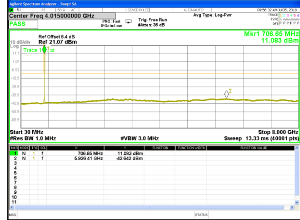
B17_QPSK_5M_Mid_CDT_Spurious
