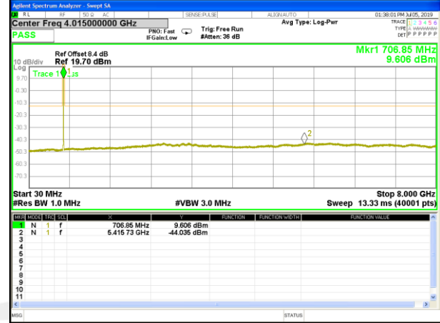
B17_Q16_5M_Mid_CDT_Spurious
