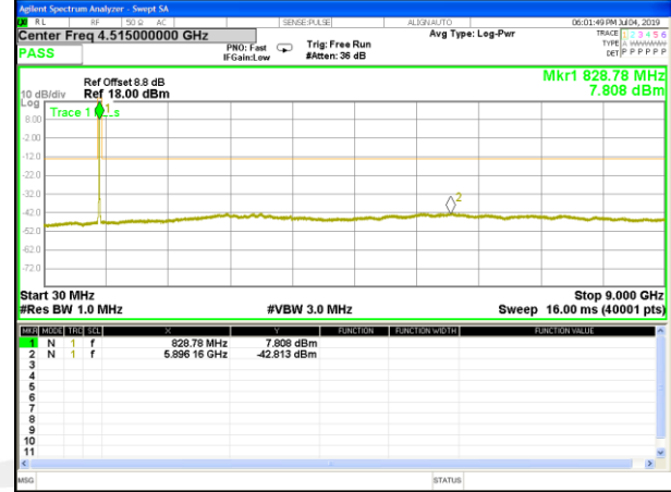
B5_Q16_10M_Mid_CDT_Spurious
