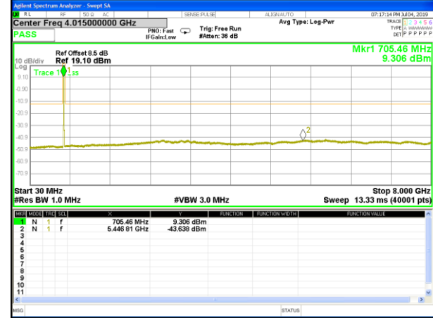
B12_QPSK_10M_Mid_CDT_Spurious
