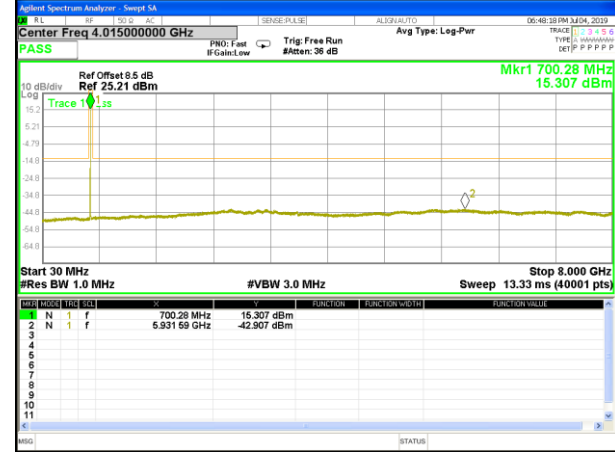
B12_QPSK_1.4M_Mid_CDT_Spurious
