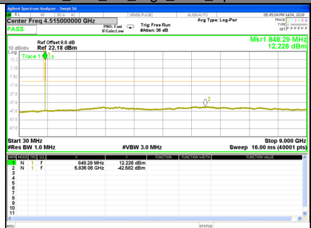
B5_Q16_3M_High_CDT_Spurious
