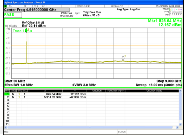
B5_Q16_3M_Mid_CDT_Spurious
