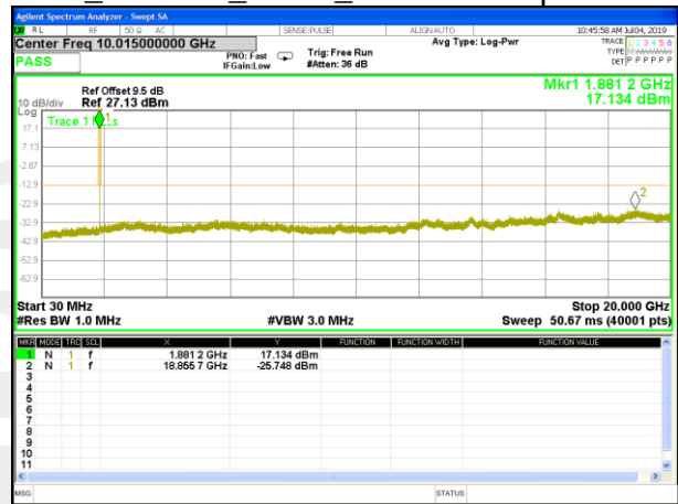
B2_WCDMA_Middle_Conducted Spurious
