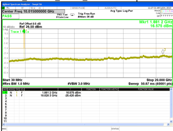
B2_HSDPA_Middle_Conducted Spurious
