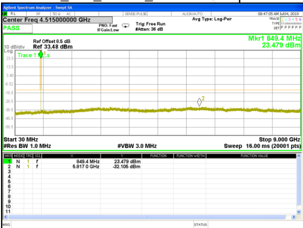
GPRS_850_Higher_Conducted Spurious
