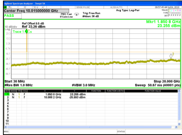
EGPRS_1900_Lower_Conducted Spurious
