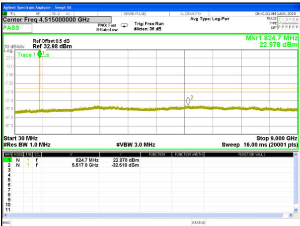
GPRS_850_Lower_Conducted Spurious
