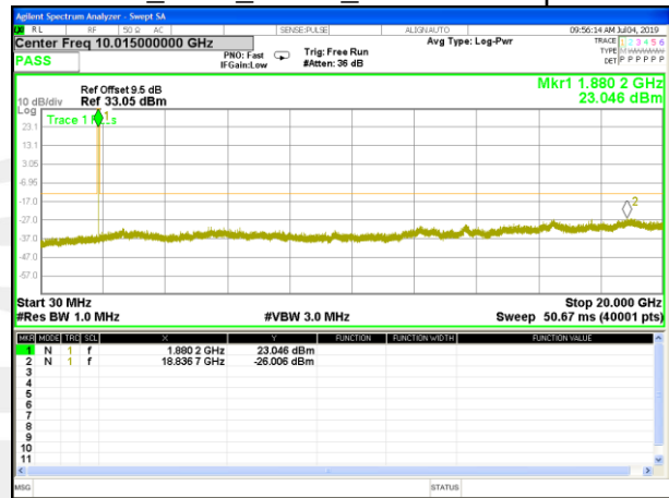
EGPRS_1900_Middle_Conducted Spurious
