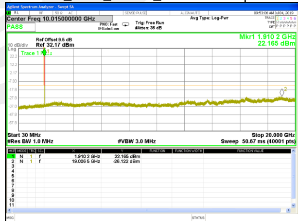
EGPRS_1900_Higher_Conducted Spurious
