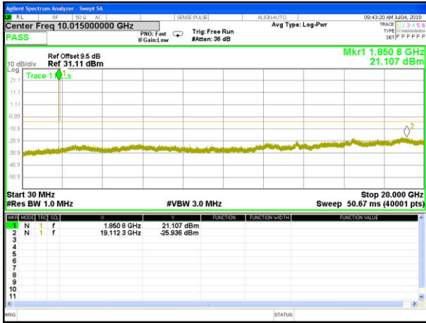
GPRS_1900_Lower_Conducted Spurious
