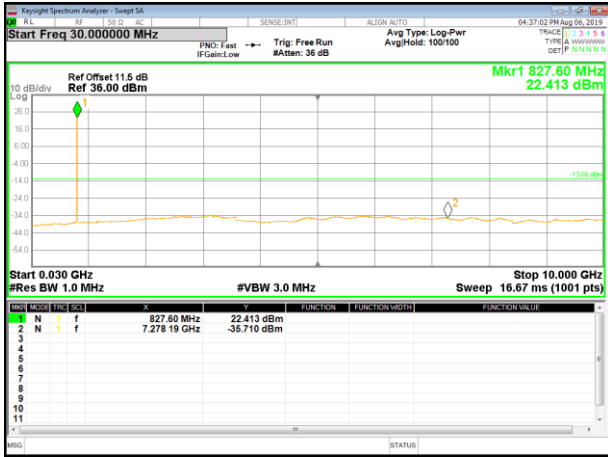
BC0_CDMA_Lower_Conducted Spurious
