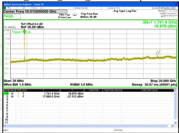
B4_HSDPA_Middle_Conducted Spurious
