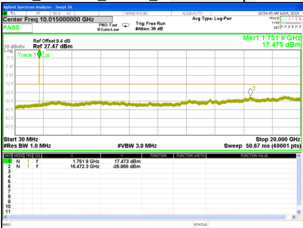
B4_WCDMA_Higher_Conducted Spurious
