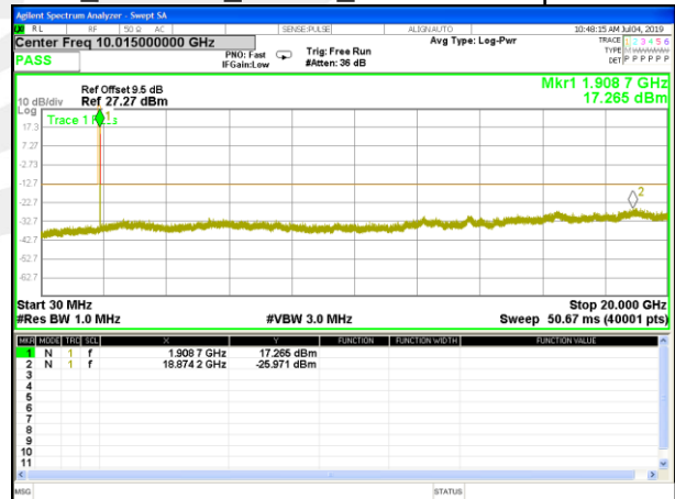
B2_WCDMA_Higher_Conducted Spurious
