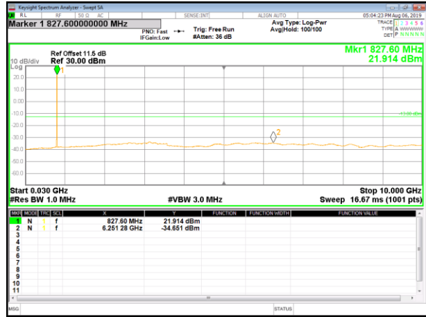
BC0_EVDO_Lower_Conducted Spurious
