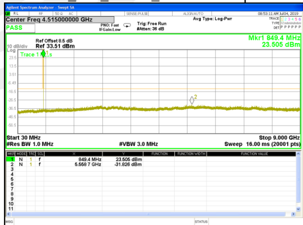
EGPRS_850_Higher_Conducted Spurious
