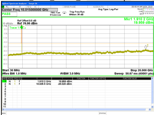
GPRS_1900_Higher_Conducted Spurious
