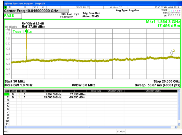
B2_WCDMA_Lower_Conducted Spurious
