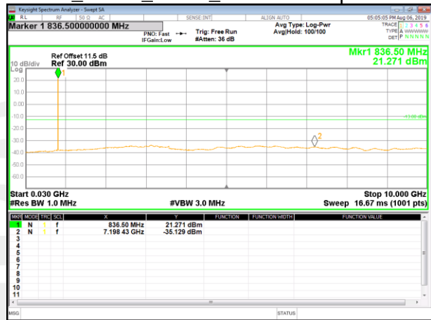
BC0_EVDO_Middle_Conducted Spurious
