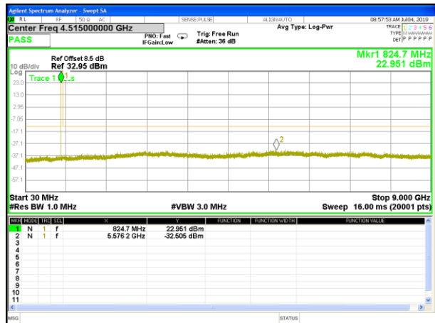
EGPRS_850_Lower_Conducted Spurious
