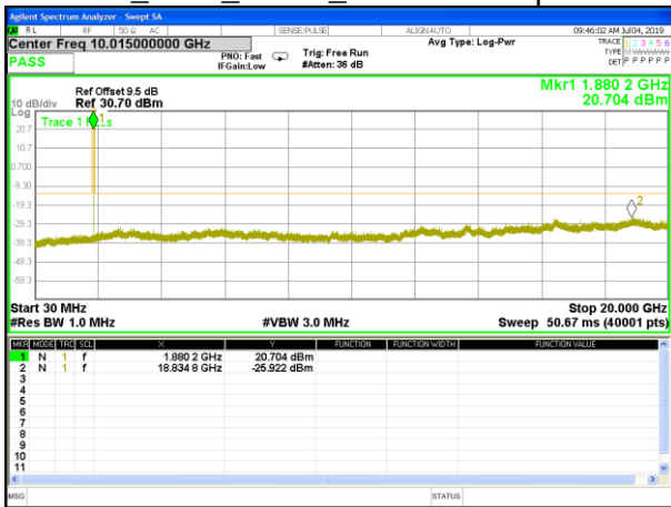
GPRS_1900_Middle_Conducted Spurious
