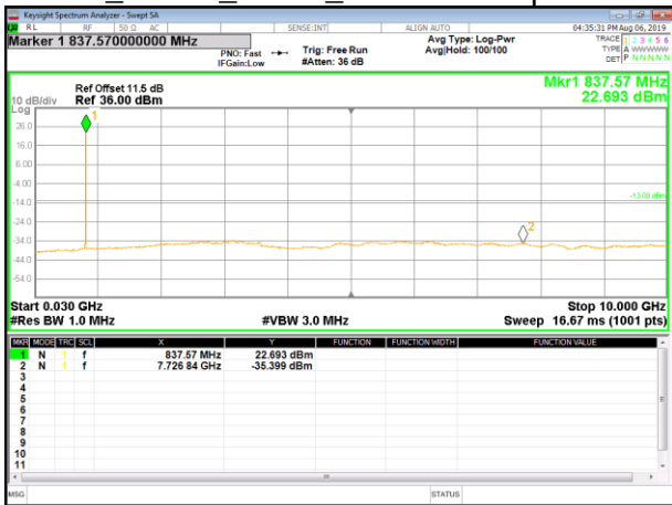
BC0_CDMA_Middle_Conducted Spurious
