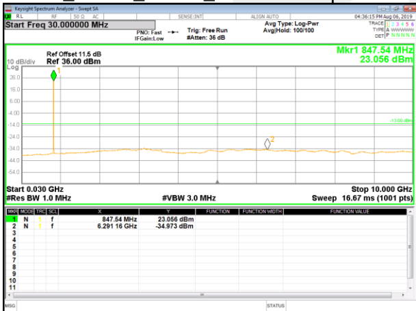
BC0_CDMA_Higher_Conducted Spurious
