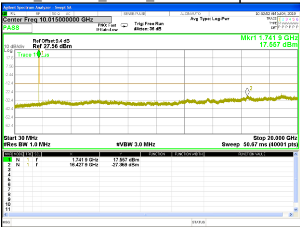
B4_WCDMA_Middle_Conducted Spurious
