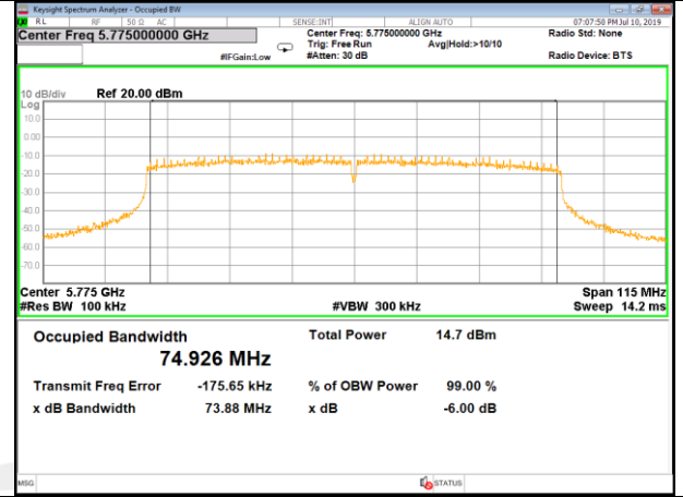
W58_11ac80_6_Bandwidth_5775M
