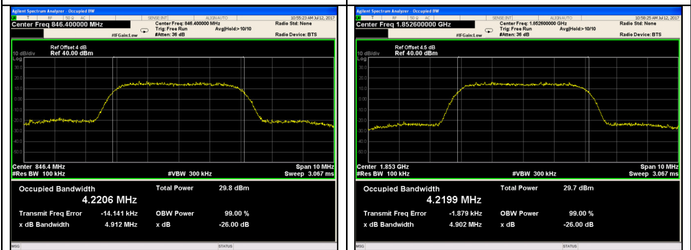
Band V BW - High CH 846.4 MHz
