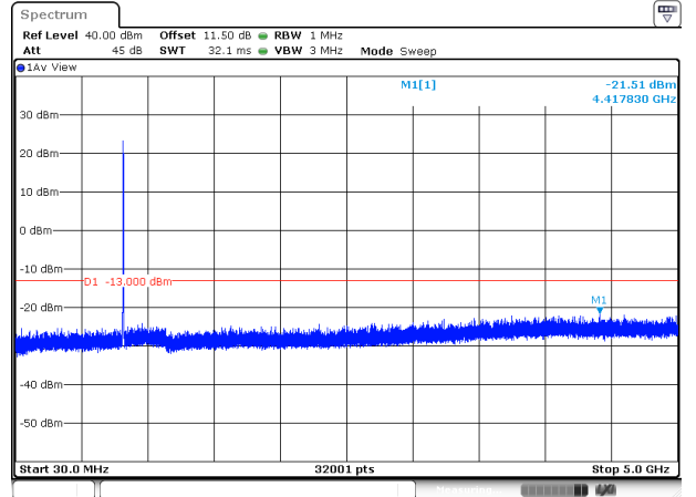
UMTS band V Conducted Emission Transmitting Mode CH 4183 30MHz – 5GHz
