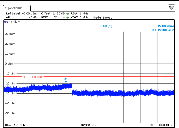
Conducted Emission Transmitting Mode CH 4183 5GHz – 10GHz
