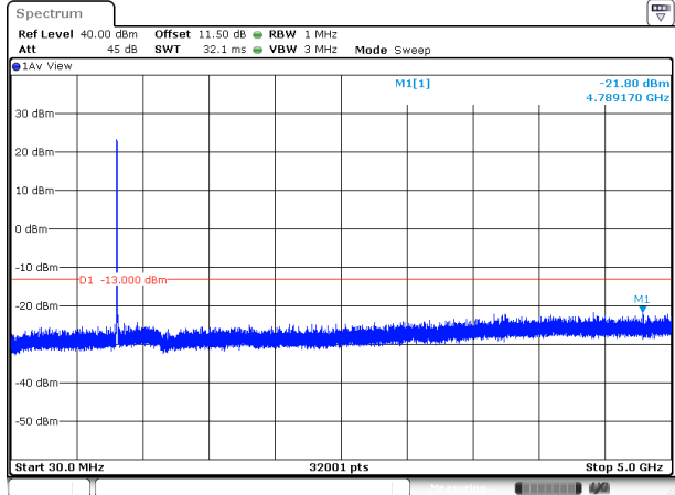
UMTS band V Conducted Emission Transmitting Mode CH 4132 30MHz – 5GHz
