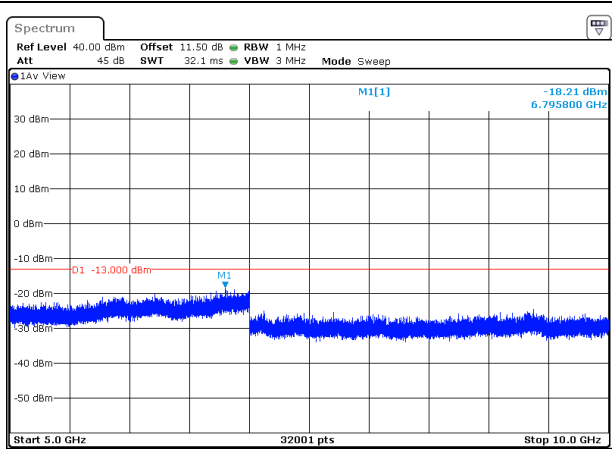
Conducted Emission Transmitting Mode CH 4132 5GHz – 10GHz
