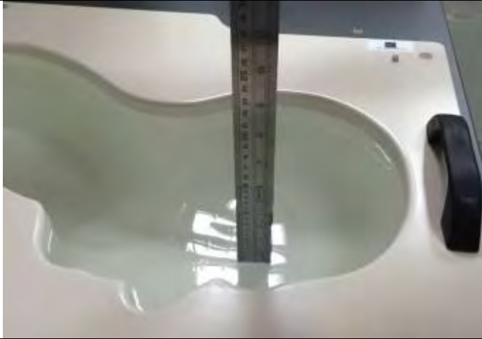
Head 1800MHz depth (15.5cm)
