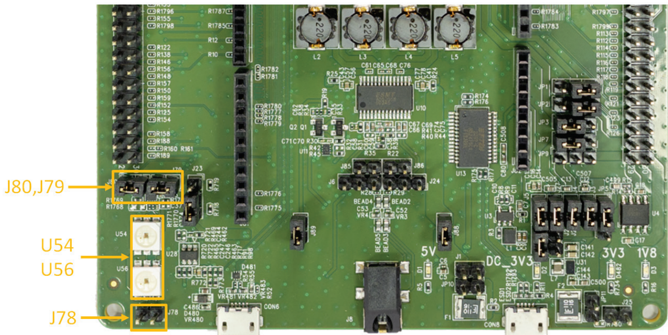
Figure 7. RGB LED
