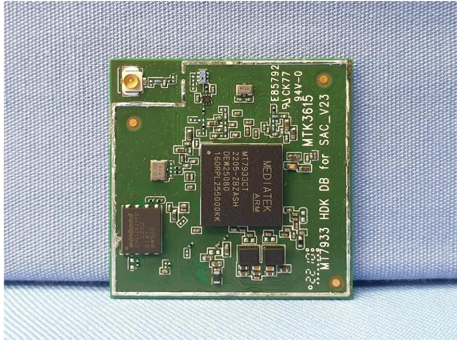
EUT Photo (1)
